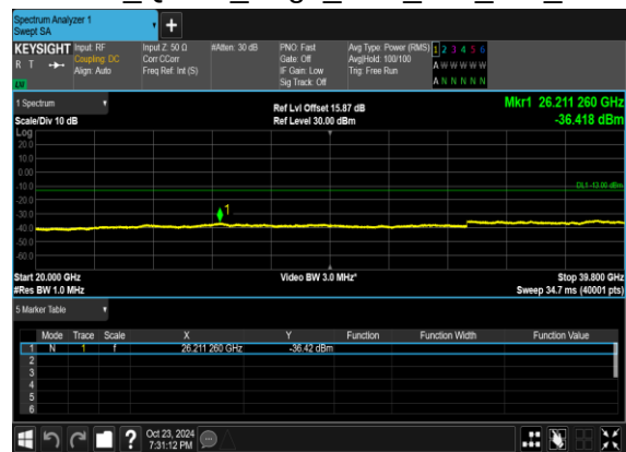
N77(60M)_DFT-s- OFDM_QPSK_Edge_1RB_Left_Mid_CH
