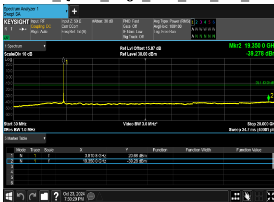
N77(60M)_DFT-s- OFDM_QPSK_Edge_1RB_Left_Mid_CH
