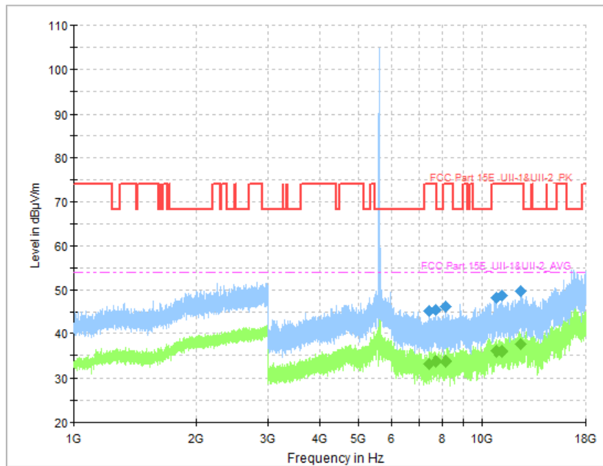
Fig. 77 Transmitter Spurious Emission (802.11a, CH116 5580MHz)
