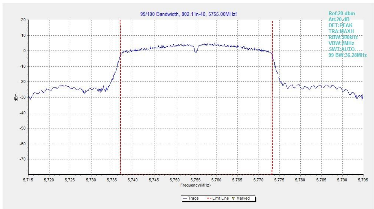
Fig. 46 99% Occupied Bandwidth (802.11n-HT40, 5755MHz)
