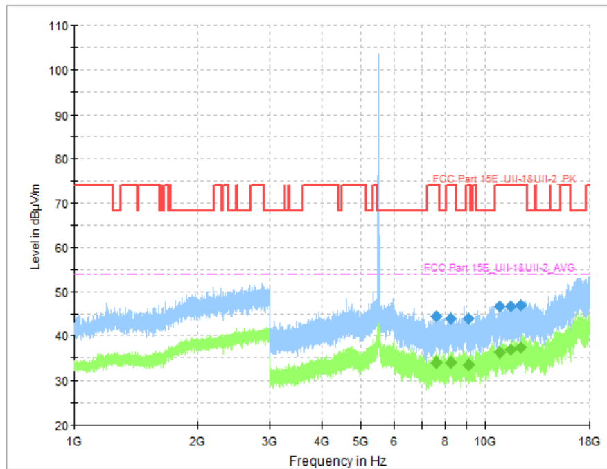
Fig. 76 Transmitter Spurious Emission (802.11a, CH100 5500MHz)
