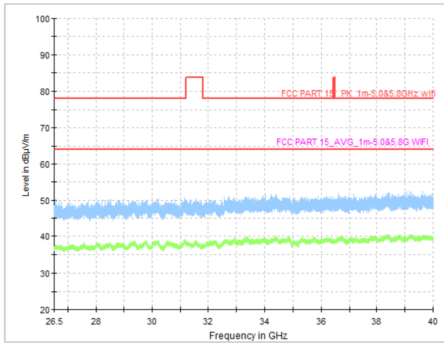
Fig. 98 Transmitter Spurious Emission (All channel, 26.5GHz~40GHz)
