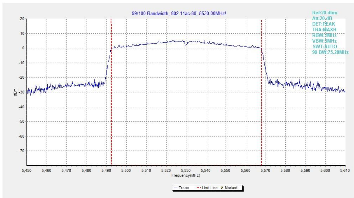
Fig. 50 99% Occupied Bandwidth (802.11ac-VHT80, 5530MHz)
