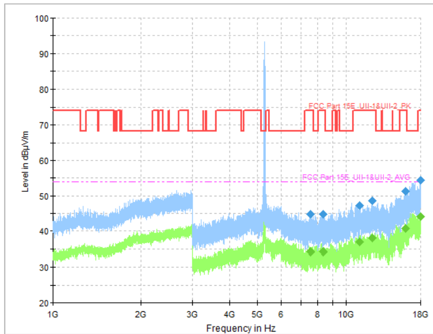
Fig. 84 Transmitter Spurious Emission (802.11n-HT40, CH54 5270MHz)
