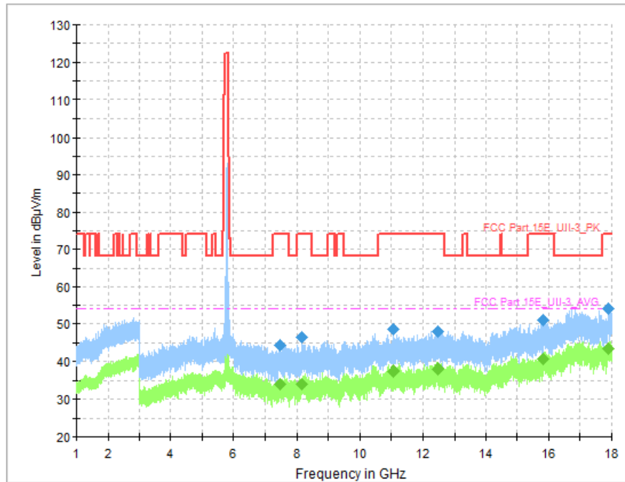
Fig. 90 Transmitter Spurious Emission (802. 11n-HT40, CH159 5795MHz)
