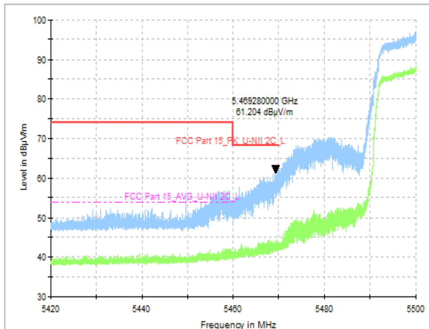
Fig. 61 Band Edges (802.11n-HT40, CH102 5510MHz)
