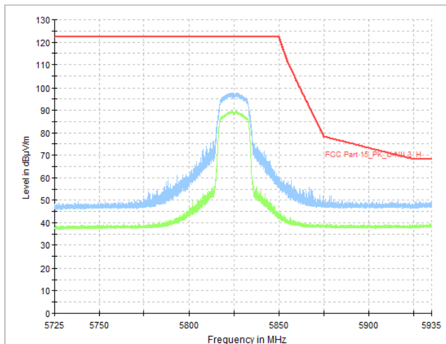
Fig. 58 Band Edges (802.11a, CH165 5825MHz)
