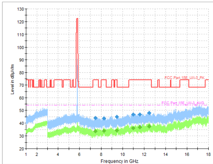
Fig. 80 Transmitter Spurious Emission (802. 11a, CH157 5785MHz)
