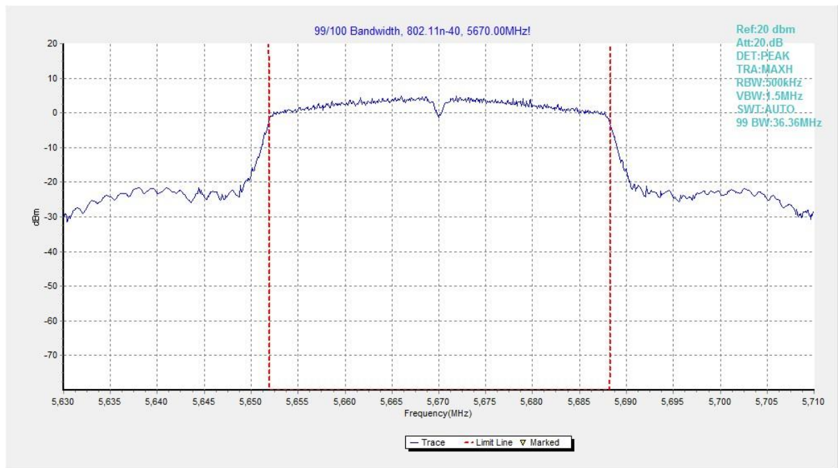
Fig. 45 99% Occupied Bandwidth (802.11n-HT40, 5670MHz)
