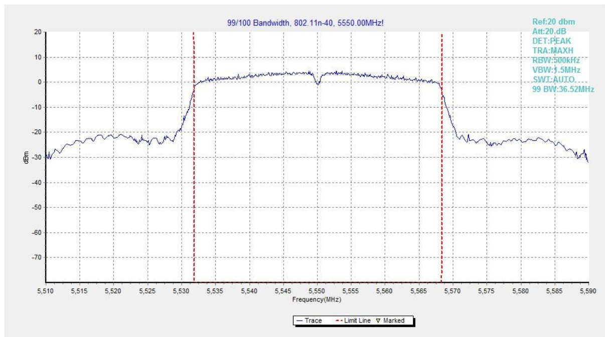
Fig. 44 99% Occupied Bandwidth (802.11n-HT40, 5550MHz)
