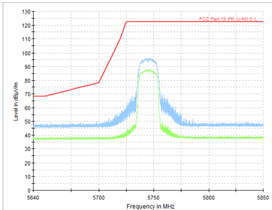
Fig. 57 Band Edges (802.11a, CH149 5745MHz)
