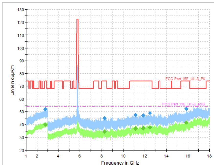
Fig. 95 Transmitter Spurious Emission (802. 11ac-VHT80, CH155 5775MHz)
