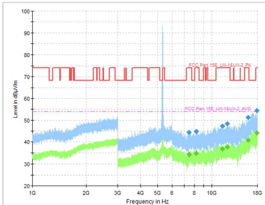
Fig. 85 Transmitter Spurious Emission (802.11n-HT40, CH62 5310MHz)
