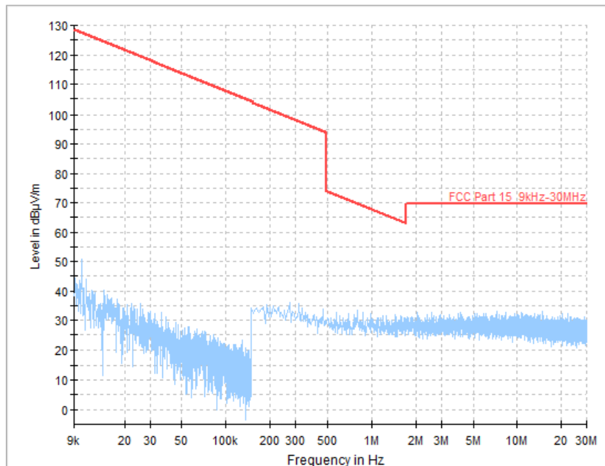
Fig. 99 Radiated Spurious Emission (All Channel, 9 kHz ~30 MHz)
