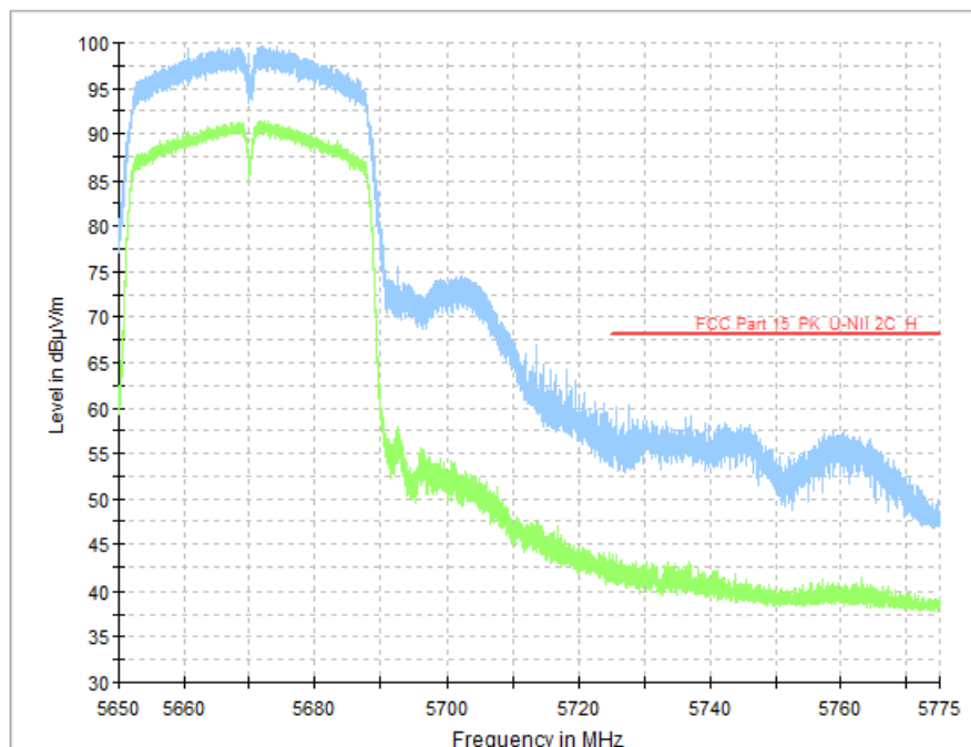
Fig. 62 Band Edges (802.11n-HT40, CH134 5670MHz)
