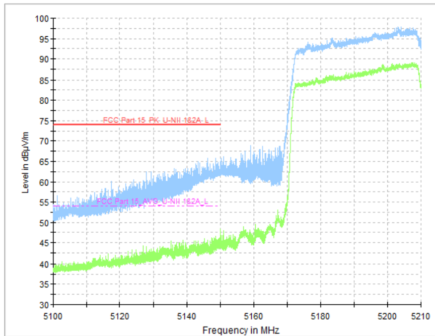
Fig. 65 Band Edges (802.11ac-VHT80, CH42 5210MHz)
