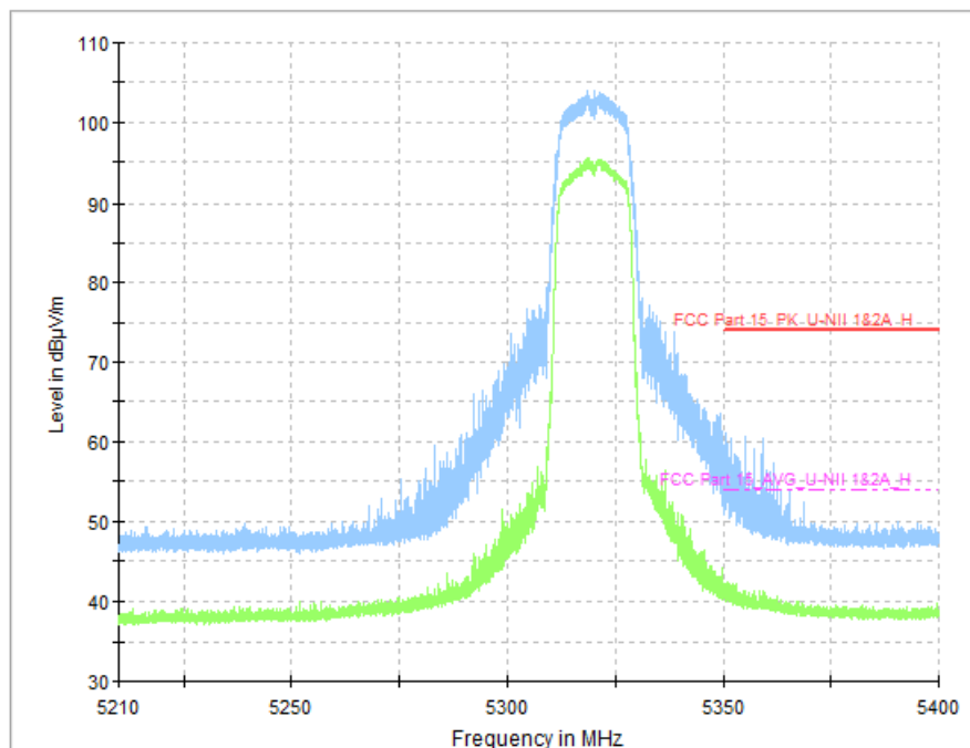
Fig. 54 Band Edges (802.11a, CH64 5320MHz)
