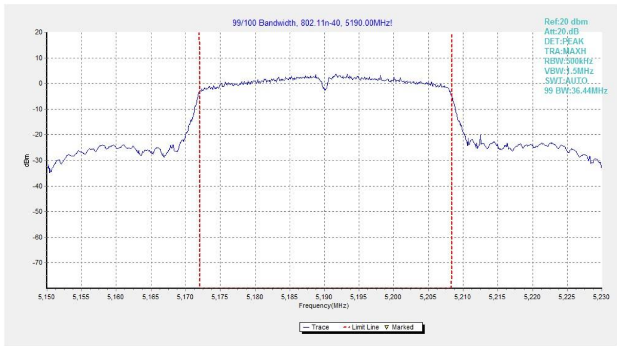
Fig. 39 99% Occupied Bandwidth (802.11n-HT40, 5190MHz)
