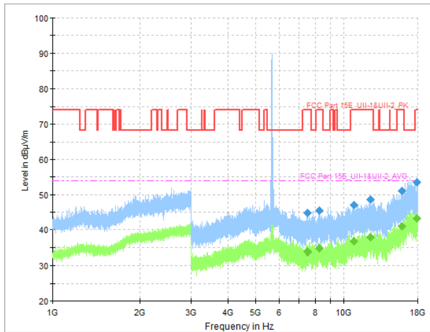
Fig. 88 Transmitter Spurious Emission (802.11n-HT40, CH134 5670MHz)
