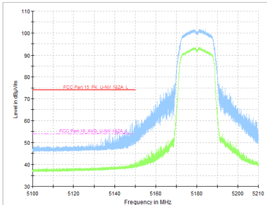
Fig. 53 Band Edges (802.11a, CH36 5180MHz)
