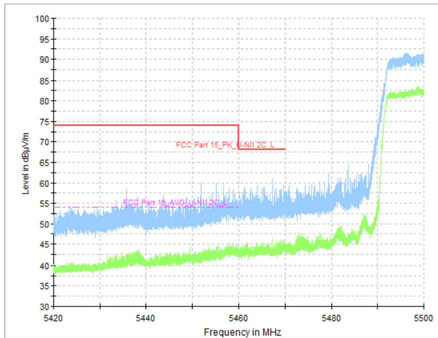
Fig. 67 Band Edges (802.11ac-VHT80, CH106 5530MHz)
