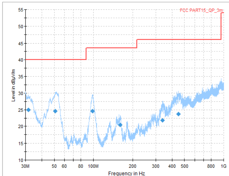
Fig. 96 Transmitter Spurious Emission (All channel, 30MHz~1GHz)
