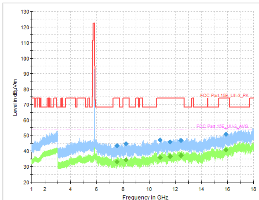
Fig. 81 Transmitter Spurious Emission (802. 11a, CH165 5825MHz)
