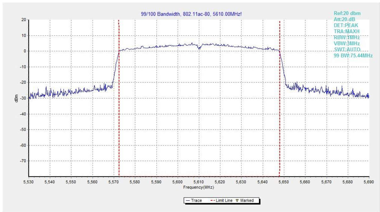
Fig. 51 99% Occupied Bandwidth (802.11ac-VHT80, 5610MHz)
