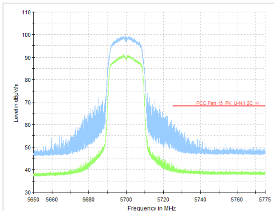
Fig. 56 Band Edges (802.11a, CH140 5700MHz)
