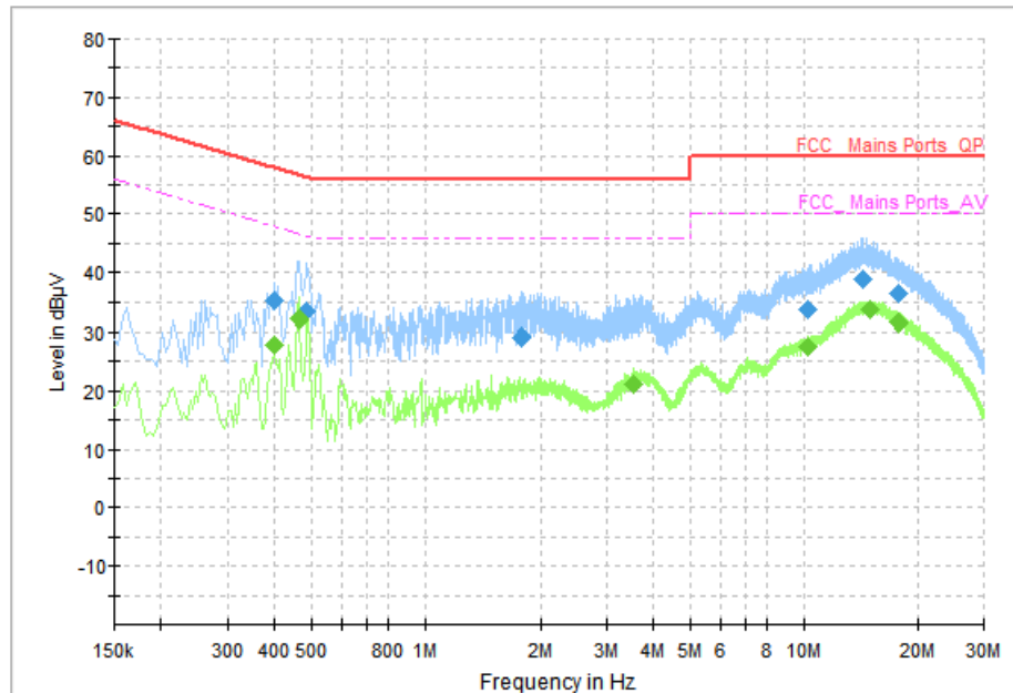
Fig. 100 AC Power line Conducted Emission (Traffic)
