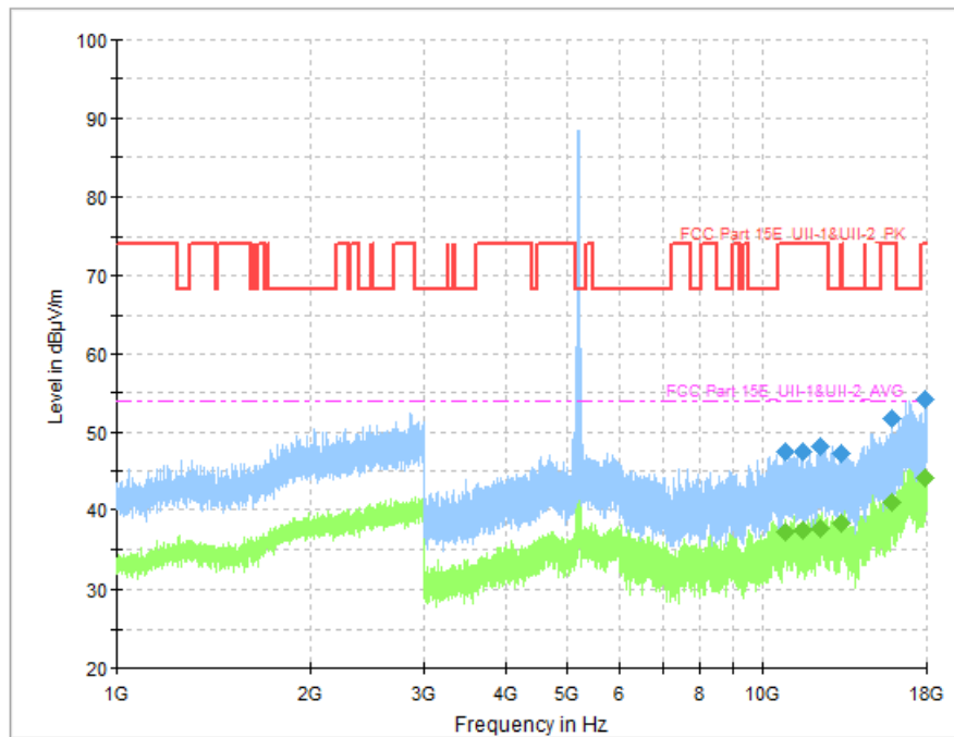
Fig. 82 Transmitter Spurious Emission (802.11n-HT40, CH38 5190MHz)
