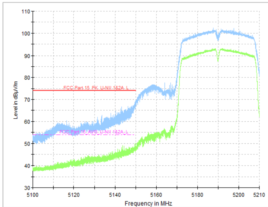
Fig. 59 Band Edges (802.11n-HT40, CH38 5190MHz)
