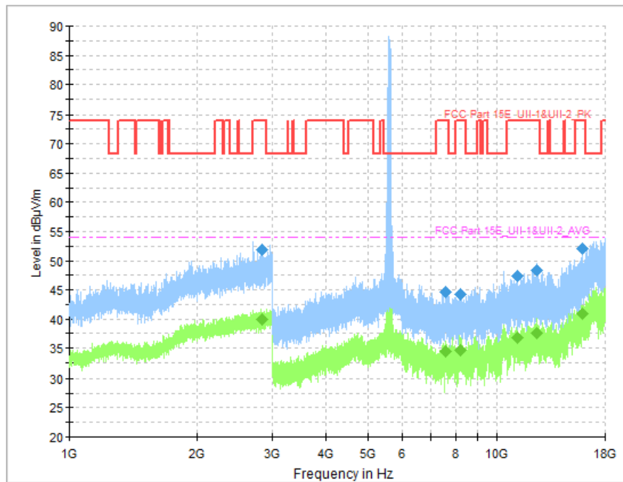
Fig. 94 Transmitter Spurious Emission (802. 11ac-VHT80, CH122 5610MHz)
