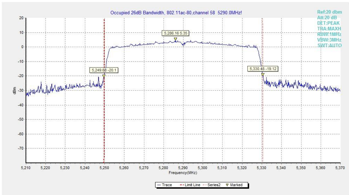
Fig. 18 Occupied 26dB Bandwidth (802. 11ac-VHT80, 5290MHz)
