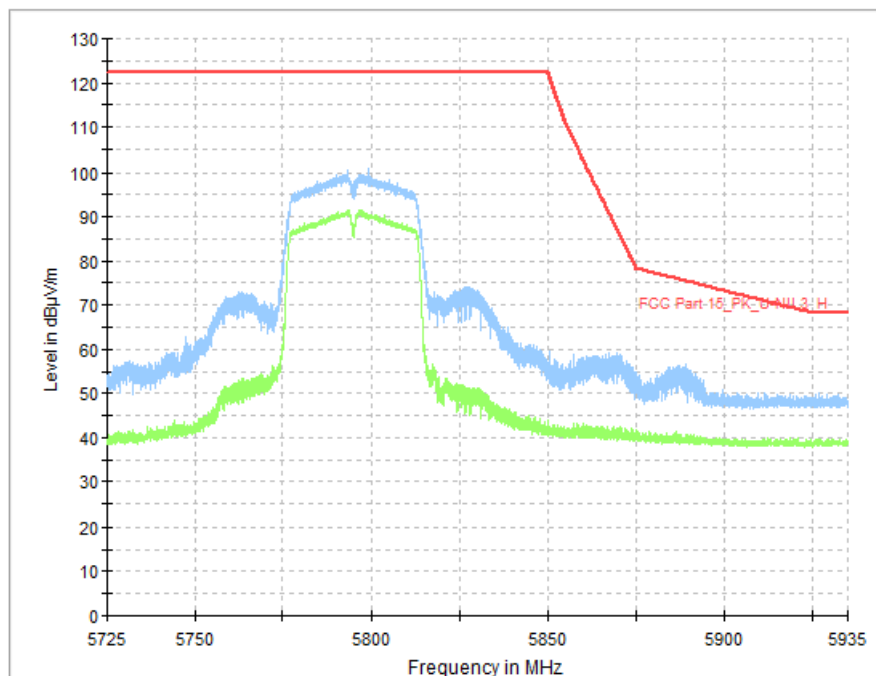
Fig. 64 Band Edges (802.11n-HT40, CH159 5795MHz)
