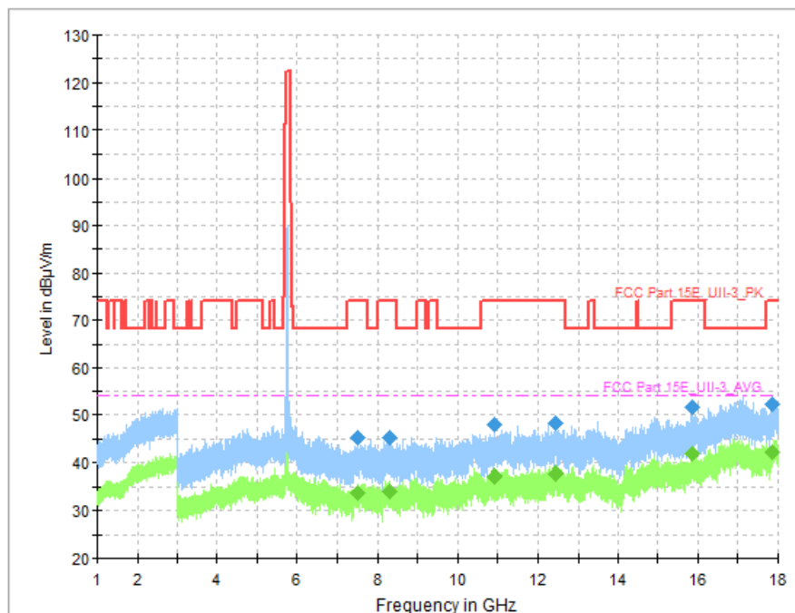
Fig. 89 Transmitter Spurious Emission (802. 11n-HT40, CH151 5755MHz)
