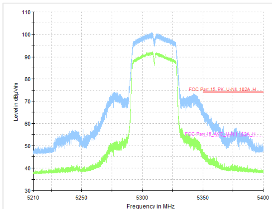
Fig. 60 Band Edges (802.11n-HT40, CH62 5310MHz)
