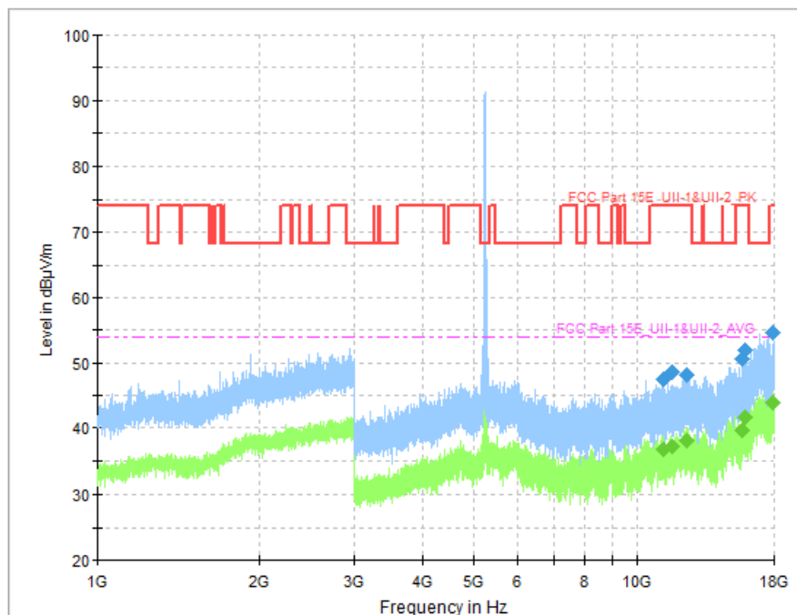
Fig. 83 Transmitter Spurious Emission (802.11n-HT40, CH46 5230MHz)
