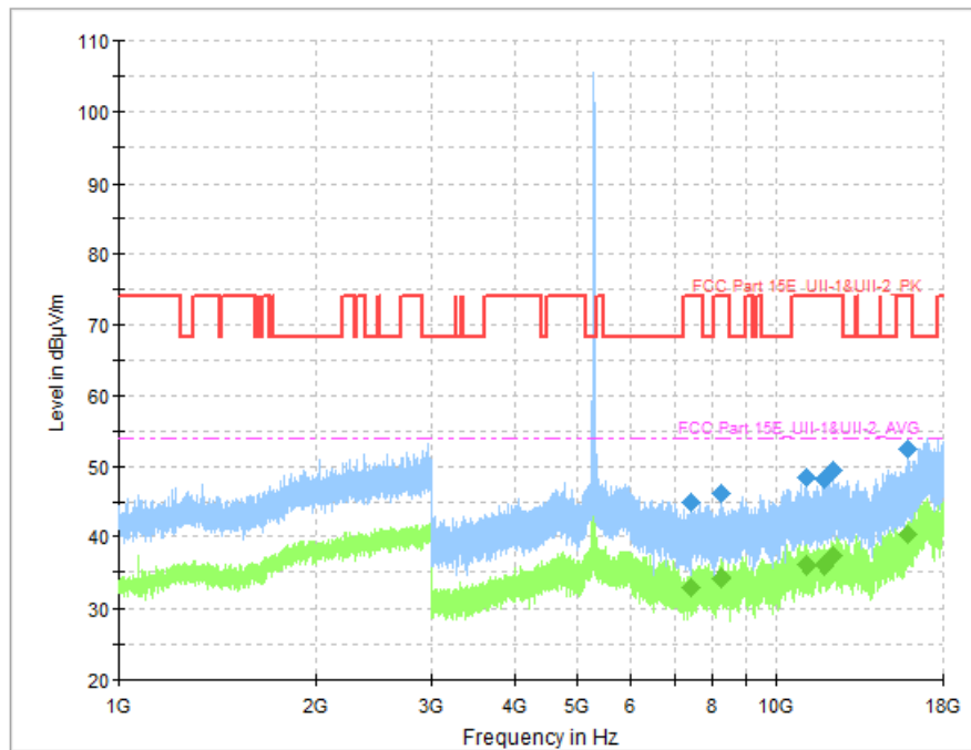
Fig. 74 Transmitter Spurious Emission (802.11a, CH56 5280MHz)
