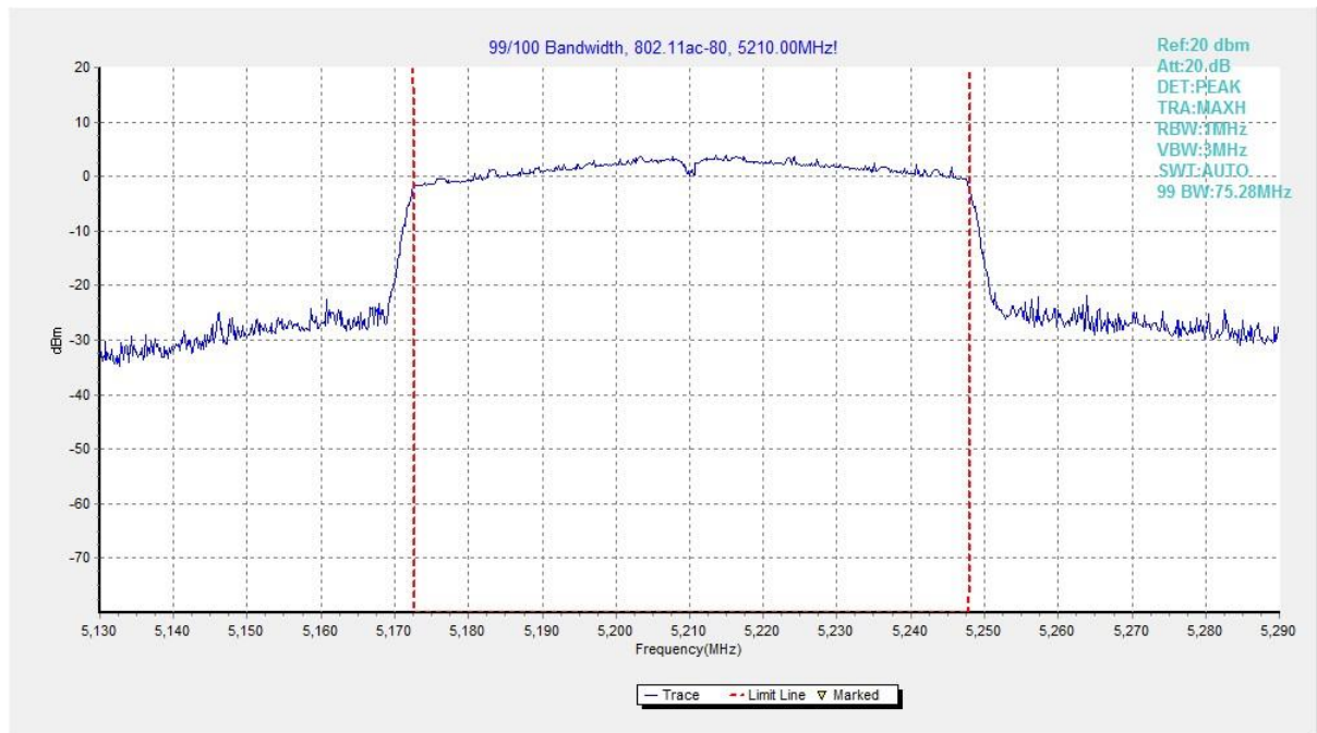
Fig. 48 99% Occupied Bandwidth (802.11ac-VHT80, 5210MHz)
