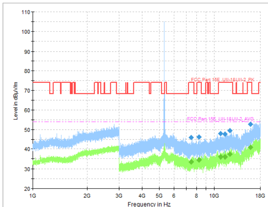
Fig. 75 Transmitter Spurious Emission (802.11a, CH64 5320MHz)
