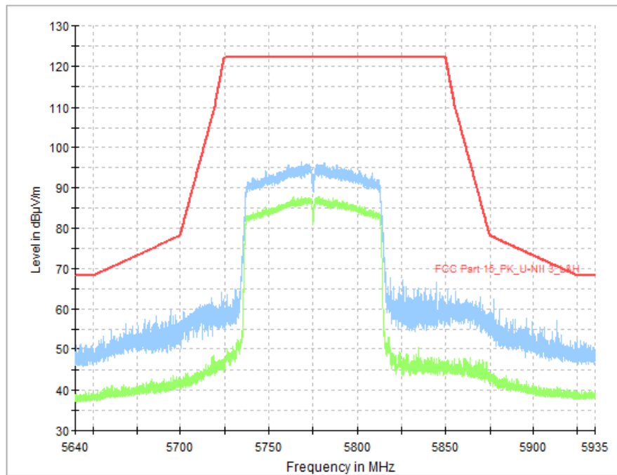
Fig. 69 Band Edges (802.11ac-VHT80, CH155 5775MHz)
