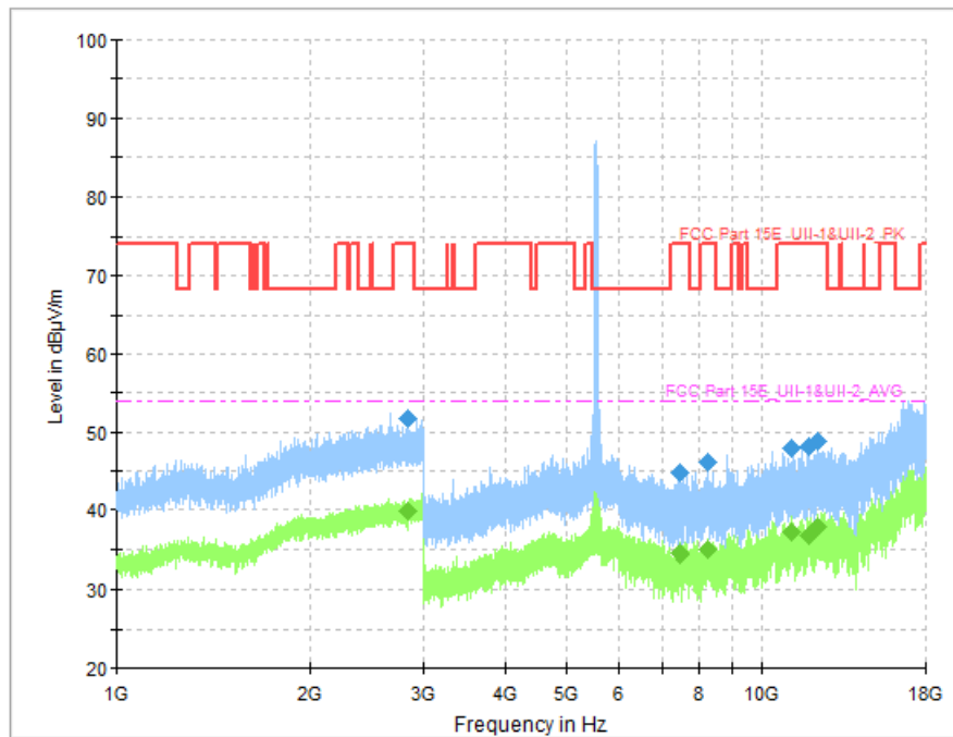
Fig. 93 Transmitter Spurious Emission (802. 11ac-VHT80, CH106 5530MHz)
