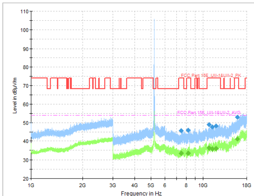
Fig. 71 Transmitter Spurious Emission (802.11a, CH40 5200MHz)
