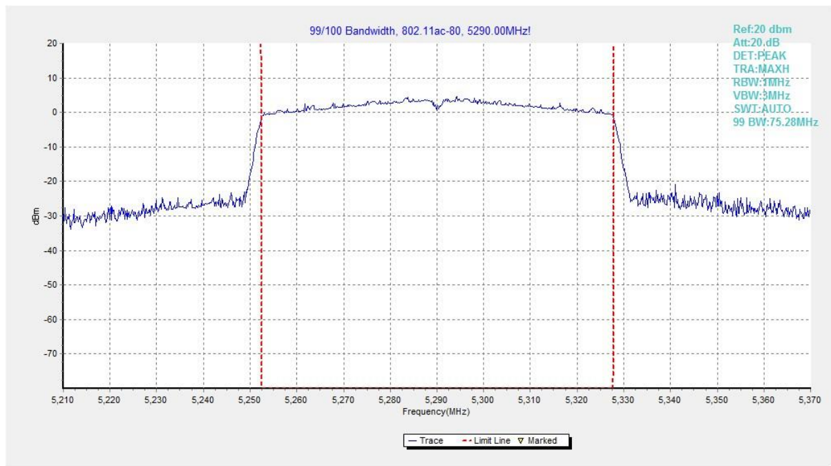
Fig. 49 99% Occupied Bandwidth (802.11ac-VHT80, 5290MHz)
