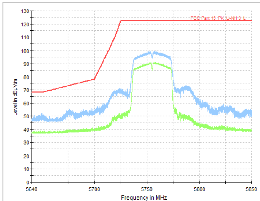
Fig. 63 Band Edges (802.11n-HT40, CH151 5755MHz)
