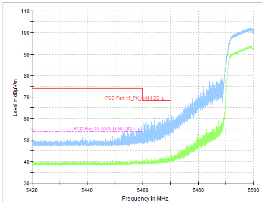
Fig. 55 Band Edges (802.11a, CH100 5500MHz)
