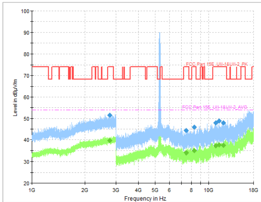
Fig. 92 Transmitter Spurious Emission (802. 11ac-VHT80, CH58 5290MHz)
