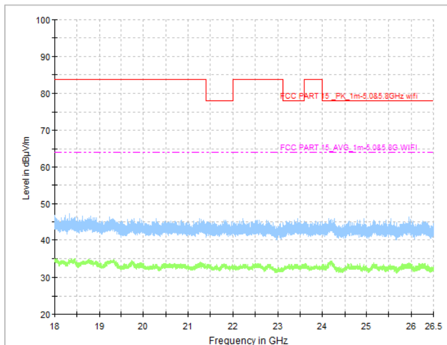
Fig. 97 Transmitter Spurious Emission (All channel, 18GHz~26.5GHz)
