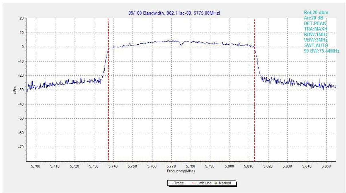
Fig. 52 99% Occupied Bandwidth (802.11ac-VHT80, 5775MHz)
