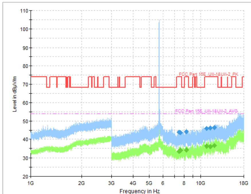
Fig. 78 Transmitter Spurious Emission (802.11a, CH140 5700MHz)
