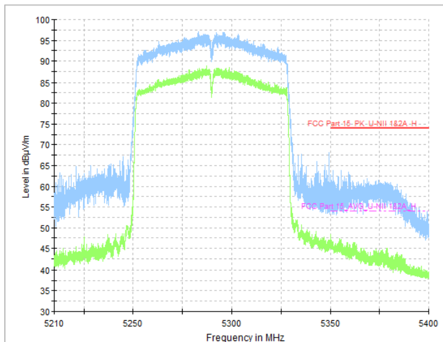
Fig. 66 Band Edges (802.11ac-VHT80, CH58 5290MHz)
