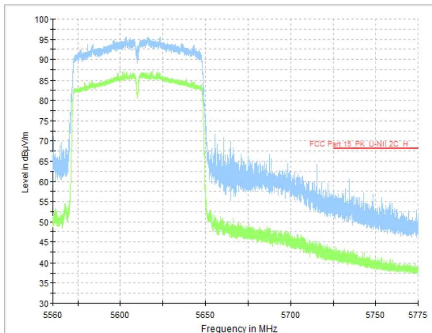
Fig. 68 Band Edges (802.11ac-VHT80, CH122 5610MHz)
