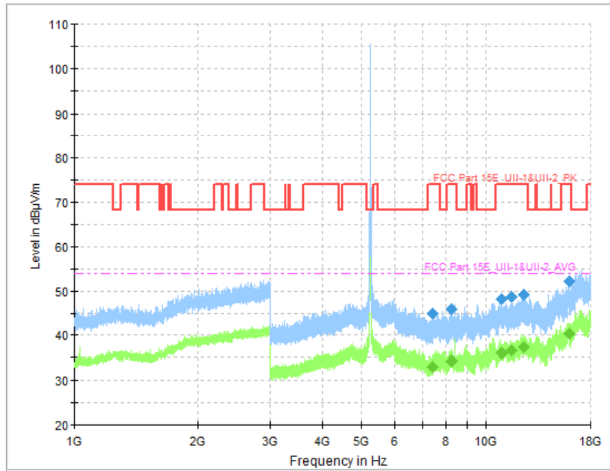
Fig. 72 Transmitter Spurious Emission (802.11a, CH48 5240MHz)
