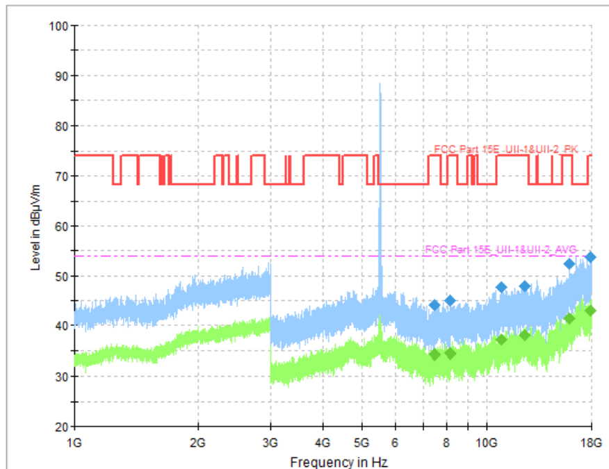
Fig. 86 Transmitter Spurious Emission (802.11n-HT40, CH102 5510MHz)
