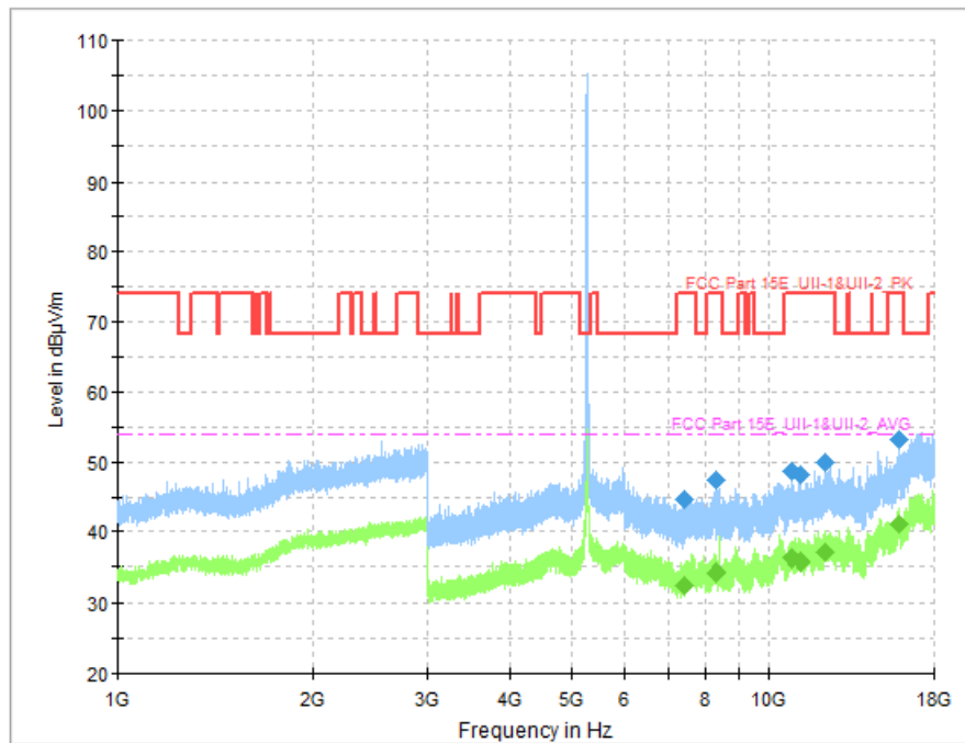
Fig. 73 Transmitter Spurious Emission (802.11a, CH52 5260MHz)
