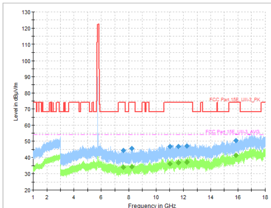
Fig. 79 Transmitter Spurious Emission (802. 11a, CH149 5745MHz)
