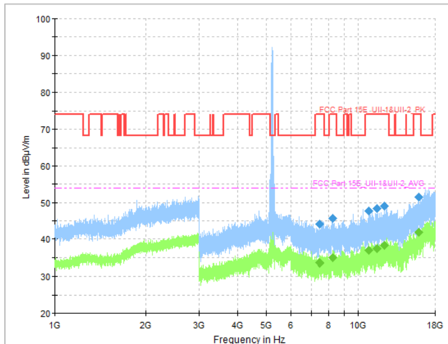
Fig. 91 Transmitter Spurious Emission (802. 11ac-VHT80, CH42 5210MHz)
