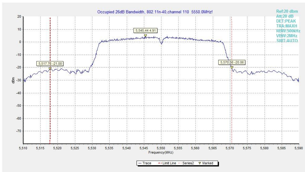
Fig. 15 Occupied 26dB Bandwidth (802.11n-HT40, 5550MHz)
