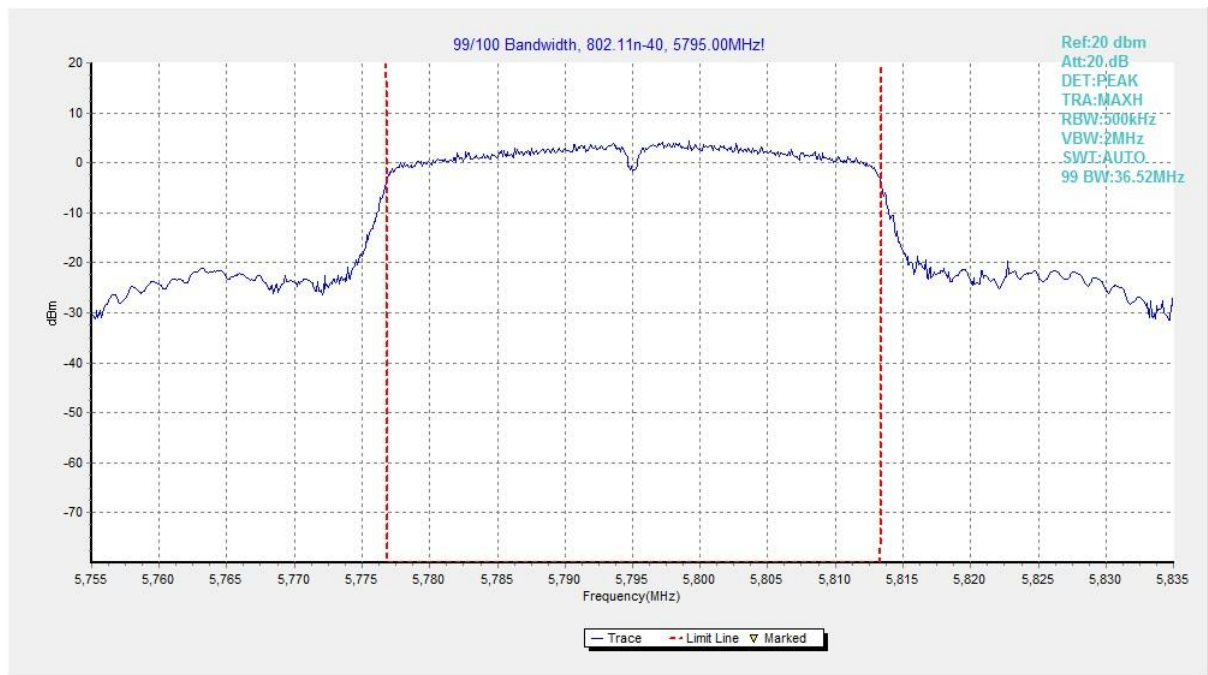
Fig. 47 99% Occupied Bandwidth (802.11n-HT40, 5795MHz)
