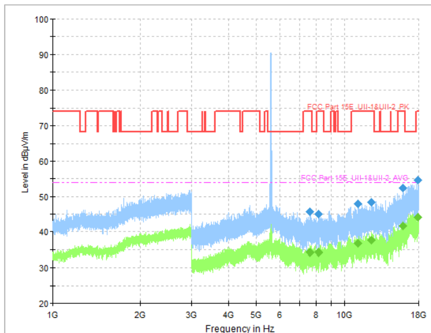
Fig. 87 Transmitter Spurious Emission (802.11n-HT40, CH110 5550MHz)
