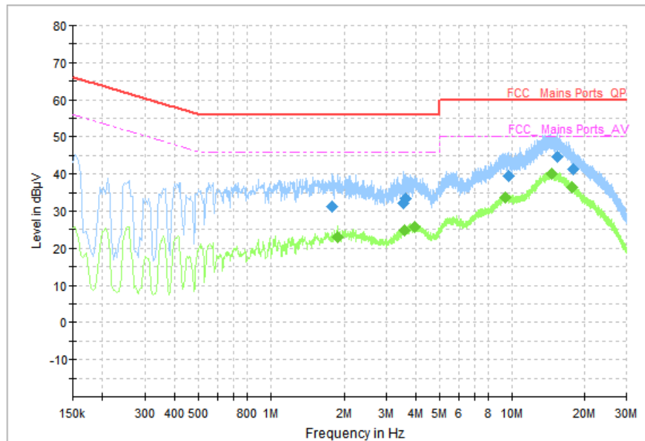
Fig. 101 AC Power line Conducted Emission (Idle)
