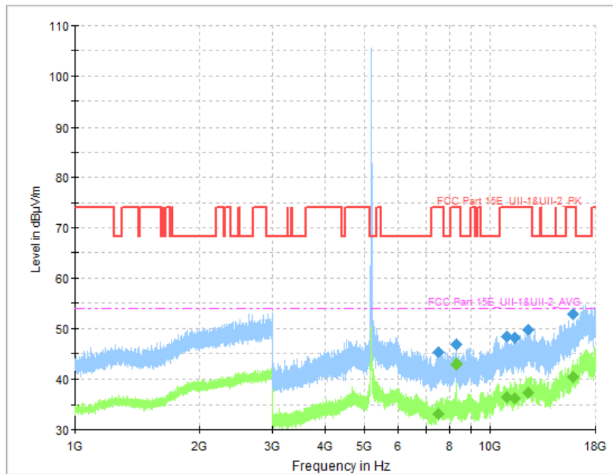
Fig. 70 Transmitter Spurious Emission (802.11a, CH36 5180MHz)
