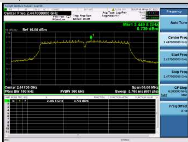
VHT(40 MHz) CHANNEL 8, CARRIER LEVEL
