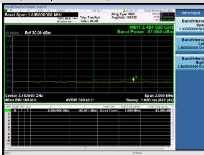
VHT(20 MHz) CHANNEL 10, BAND EDGE
