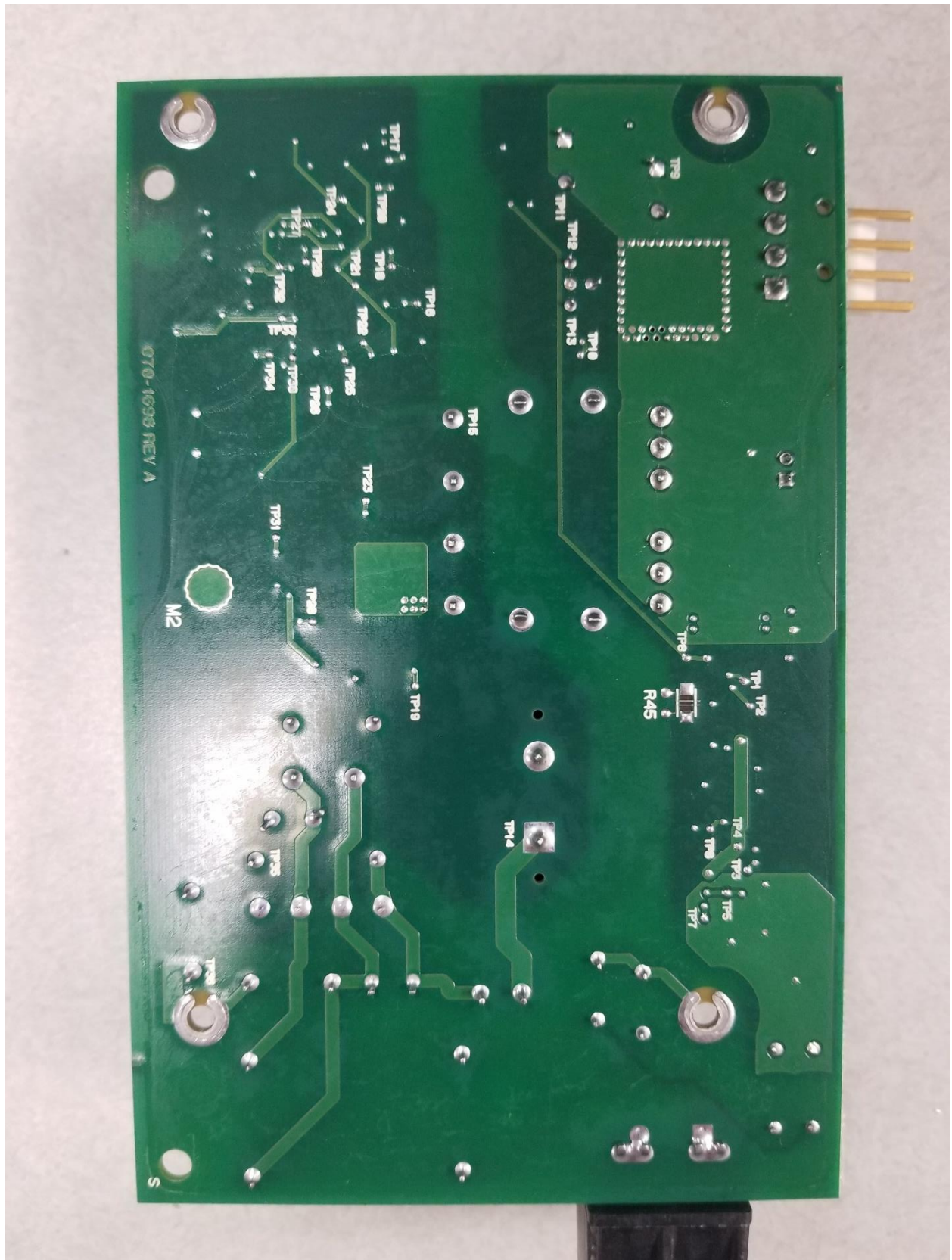
Figure 9: POWER BOARD BOTTOM
