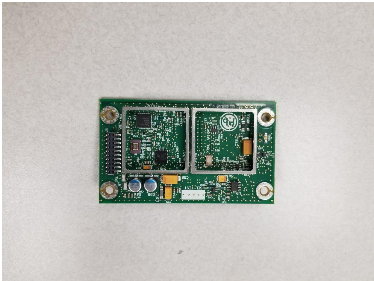
Figure 6: RADIO BOARD BOTTOM - NO SHIELD
