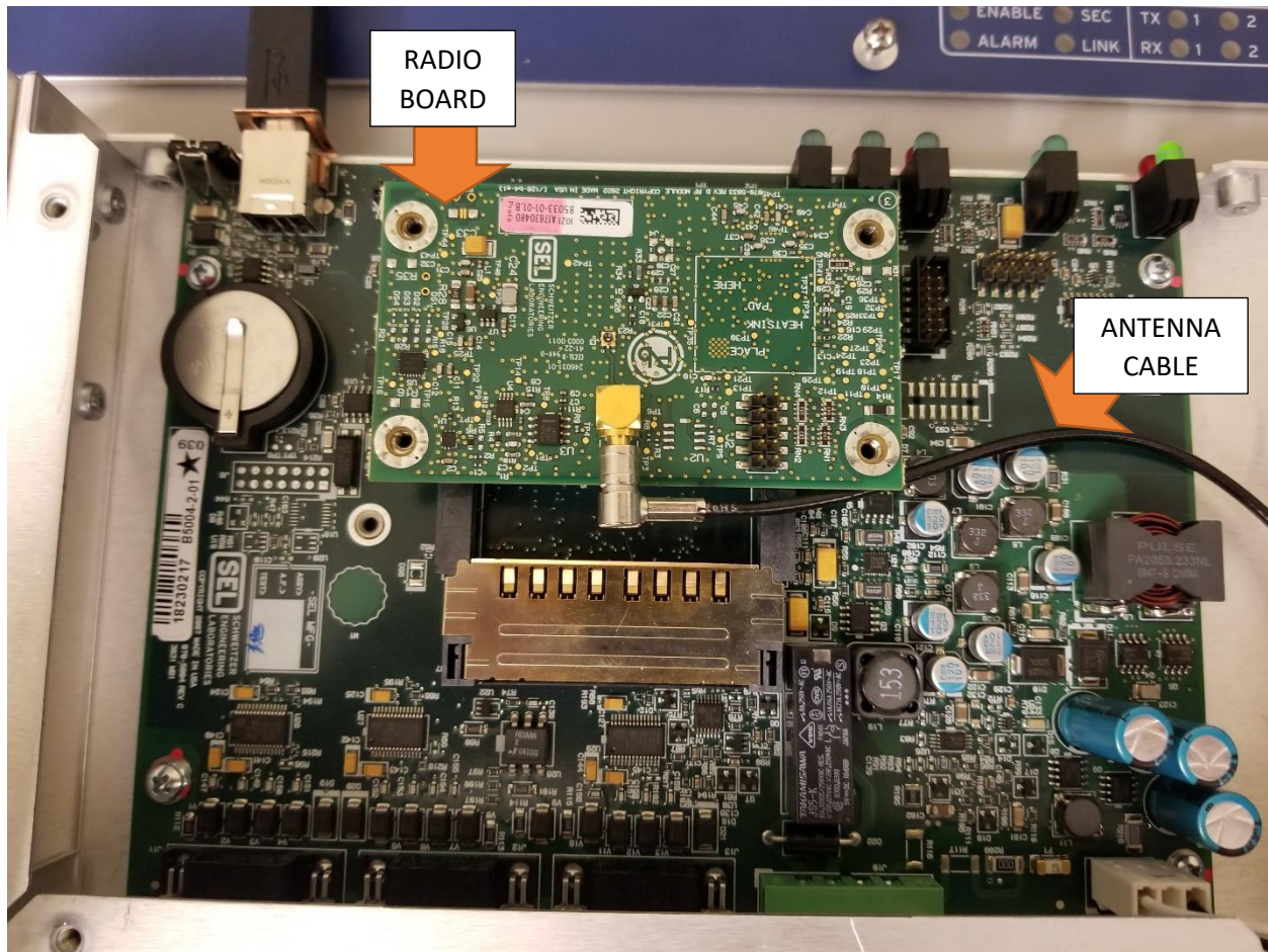
Figure 2: RADIO AND MAIN BOARD
