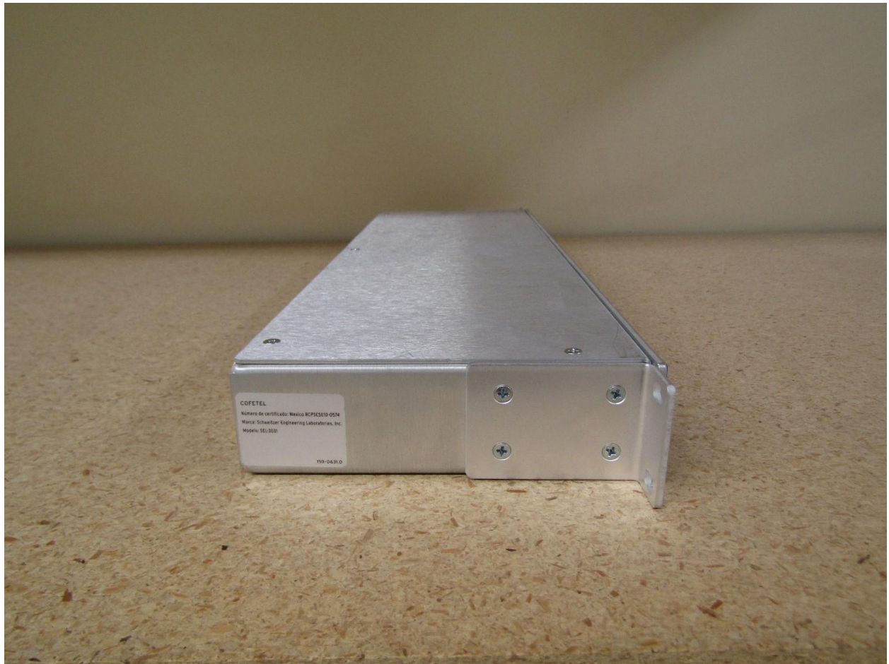
Figure 5: RACK MOUNT LEFT
