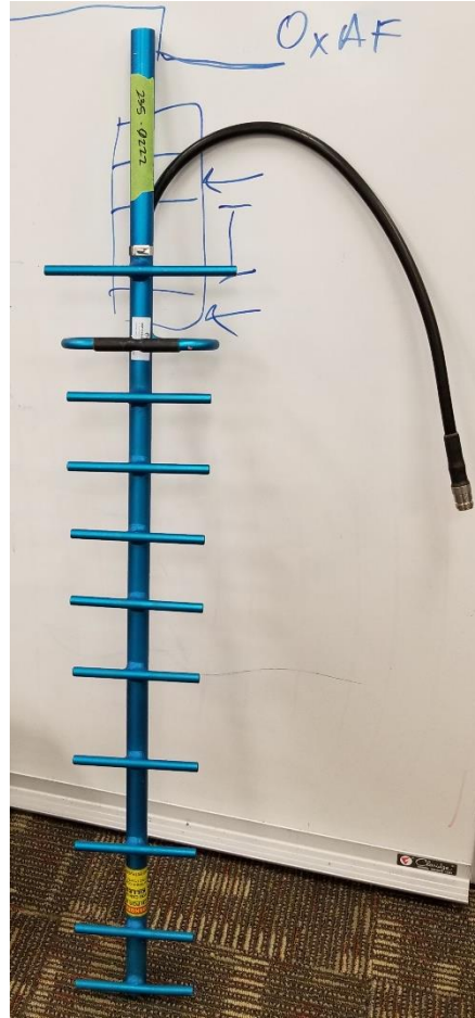
Figure 7: PCTEL BMYD890M YAGI
