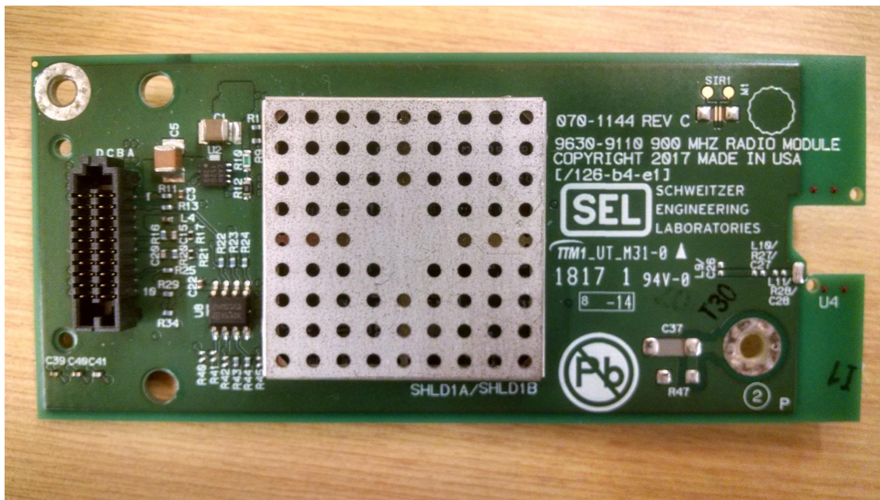
Figure 4: RF connector variant, bottom
