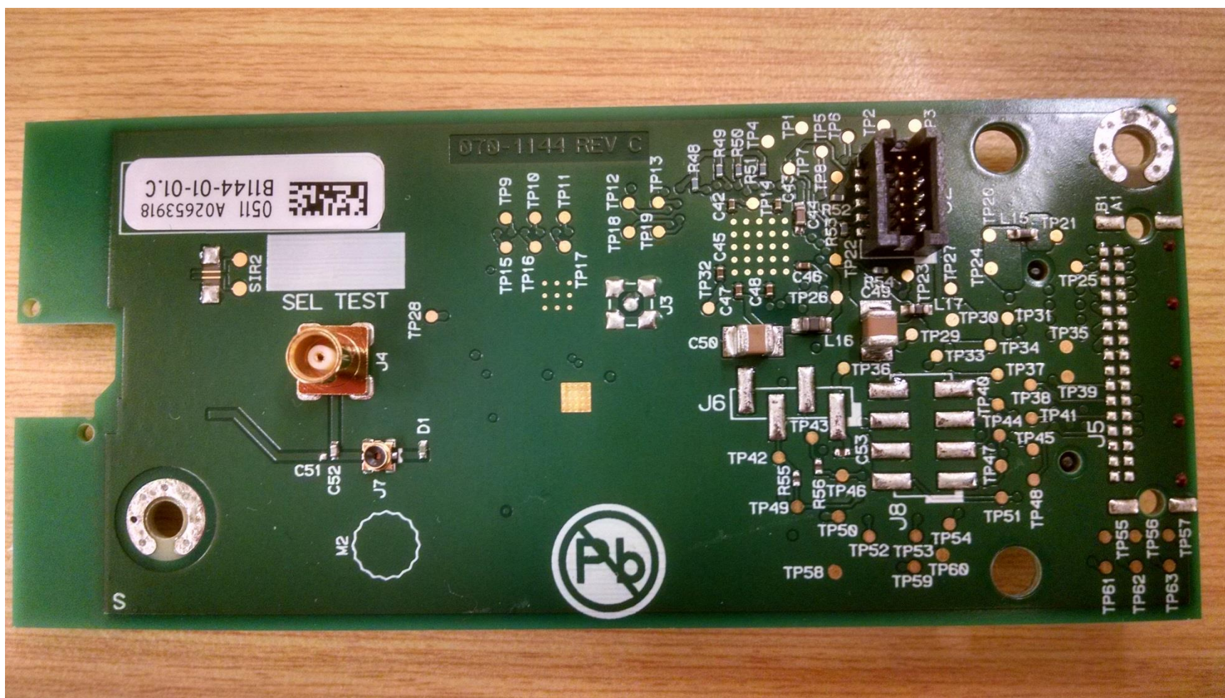
Figure 3: RF connector variant, top
