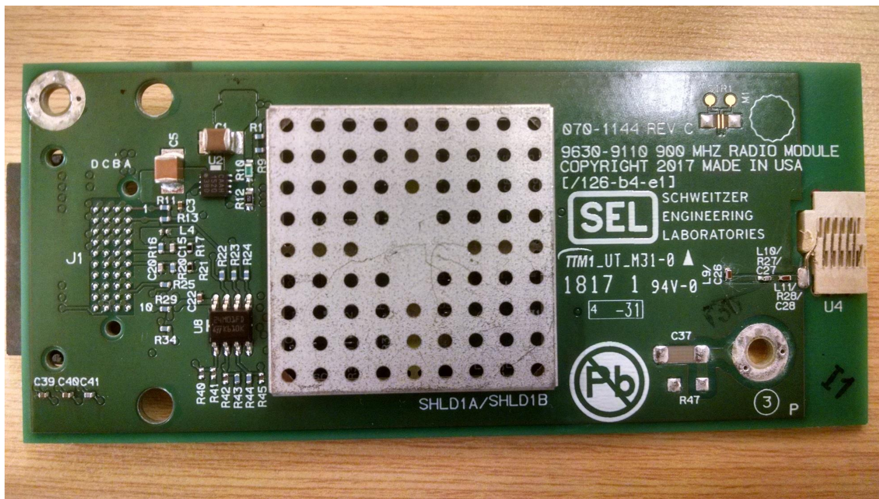
Figure 2: Integral antenna variant, bottom
