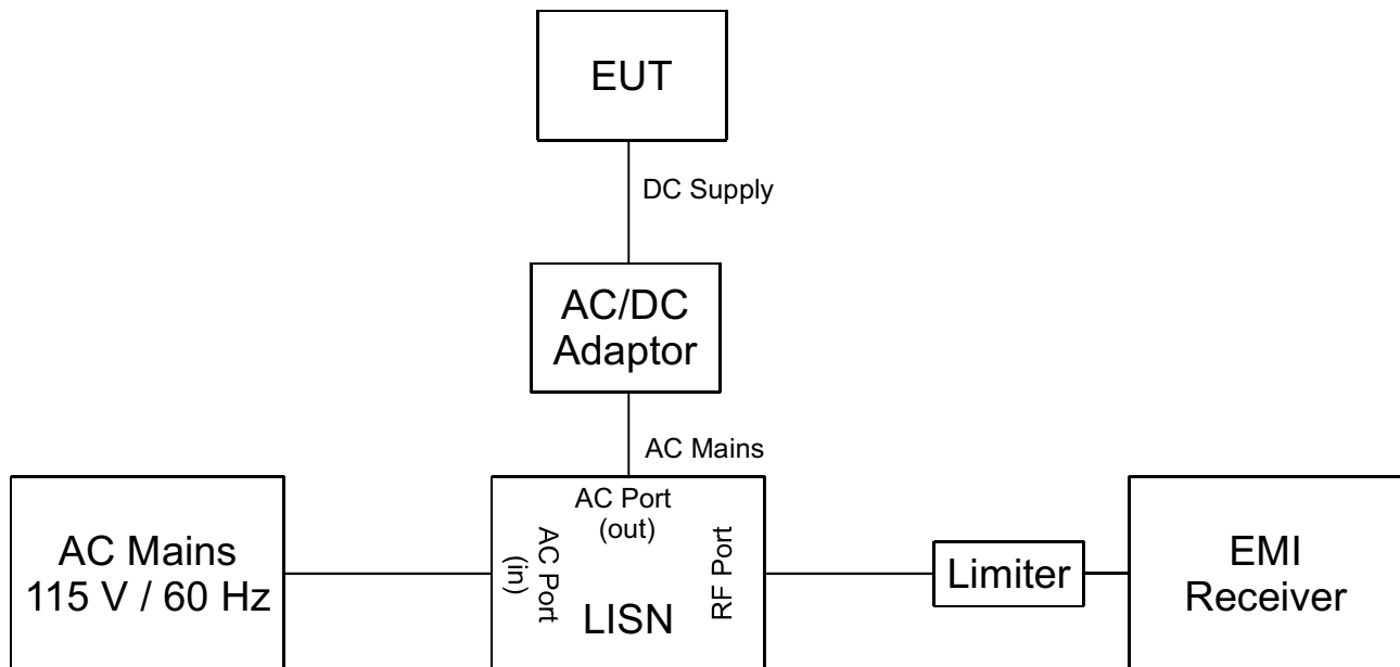
Schematic diagram
