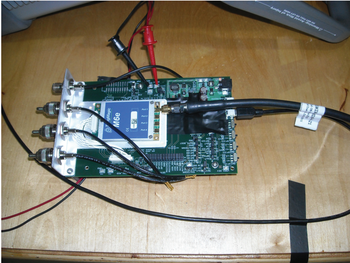
Module on the test board
