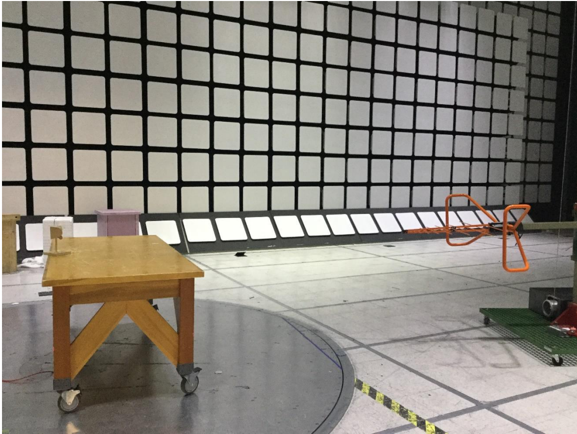
Figure 1 – Radiated Emissions Test Setup, 30MHz – 1GHz
