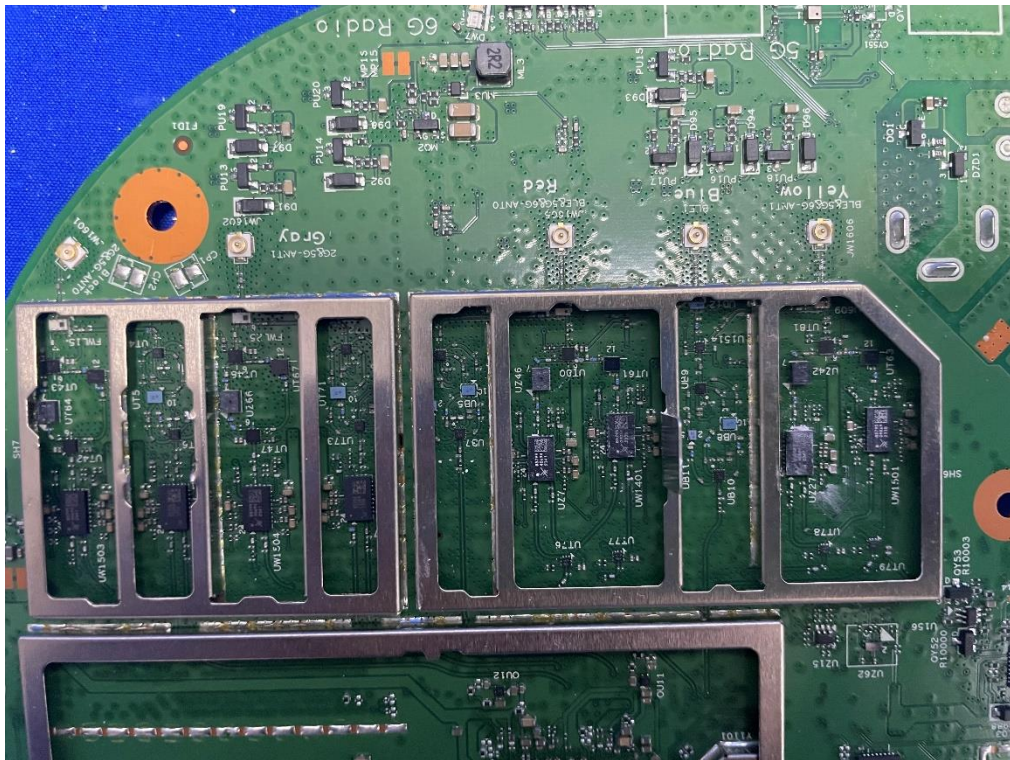
(17) EUT Photo (Model: APIN0734)
