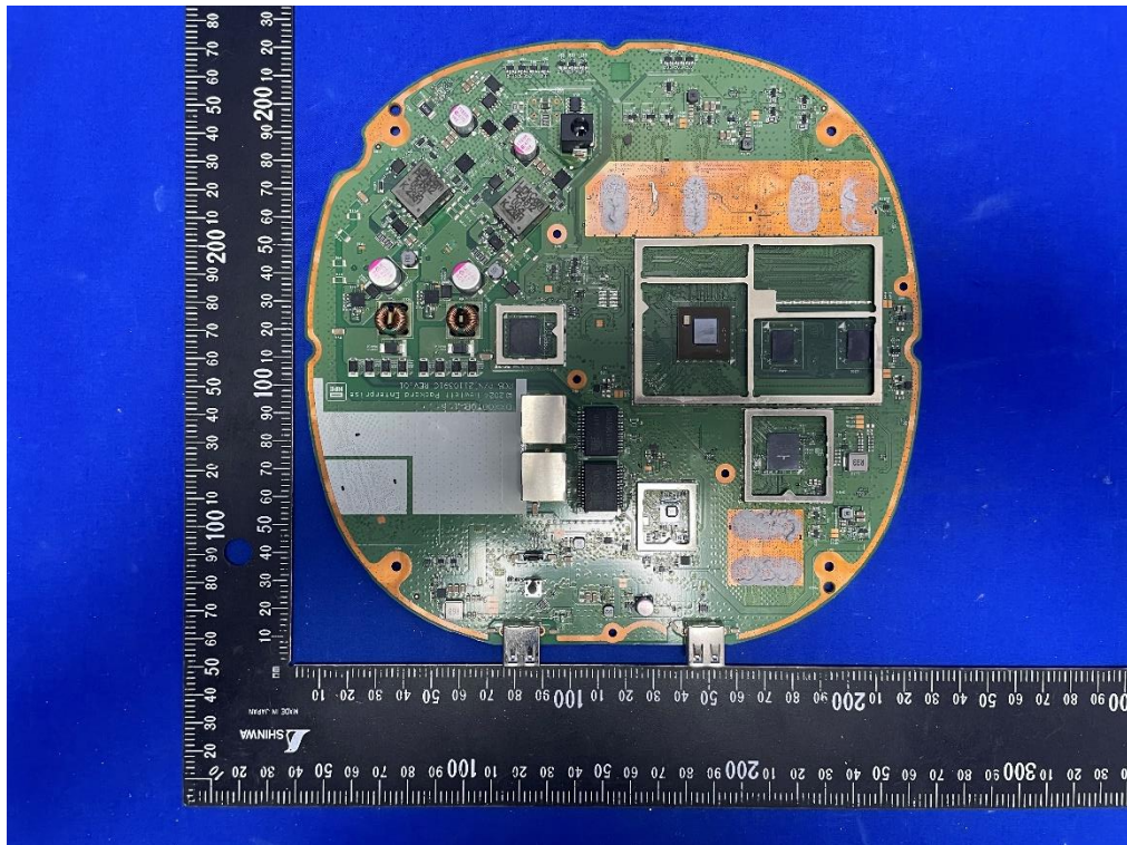
(9) EUT Photo (Model: APIN0734)
