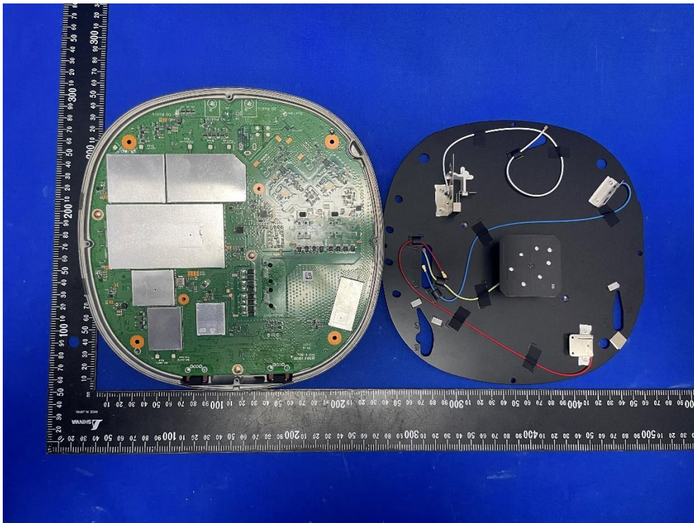
(3) EUT Photo (Model: APIN0734)
