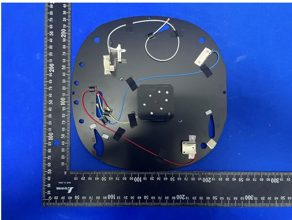
(4) EUT Photo (Model: APIN0734)
