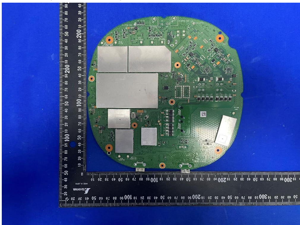
(8) EUT Photo (Model: APIN0734)
