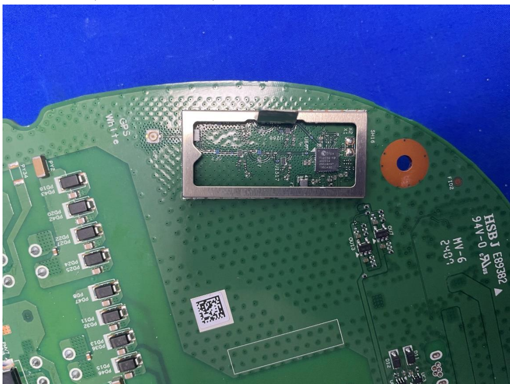
(18) EUT Photo (Model: APIN0734)
