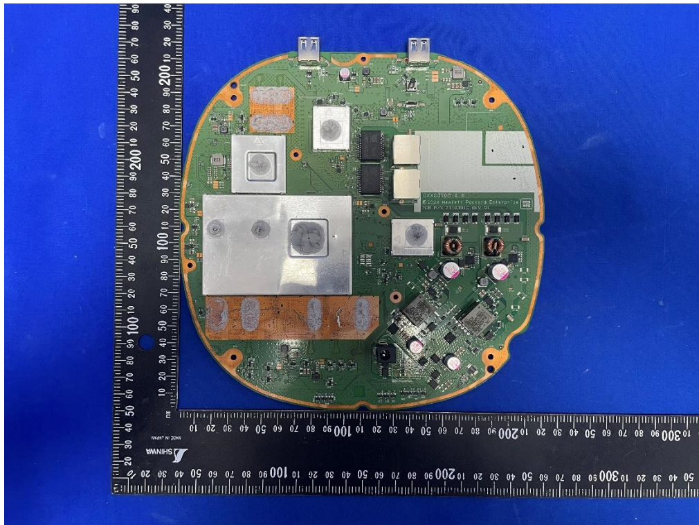
(7) EUT Photo (Model: APIN0734)
