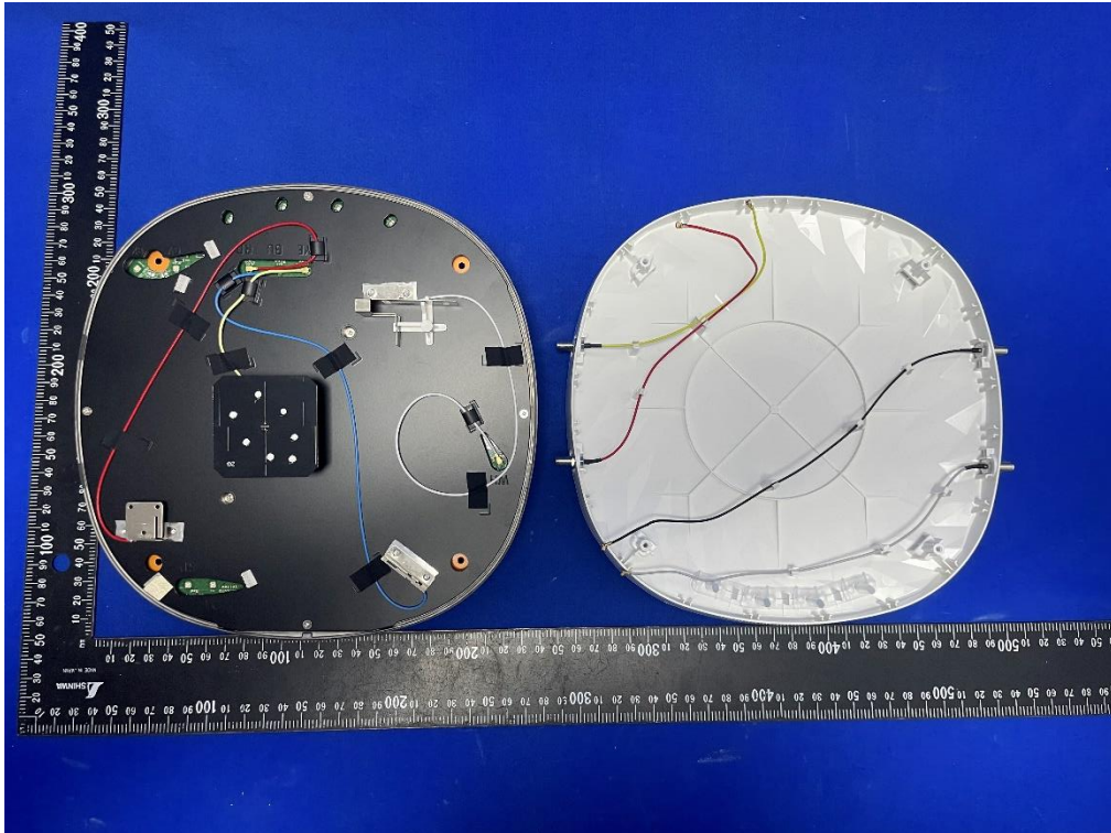
(2) EUT Photo (Model: APIN0734)
