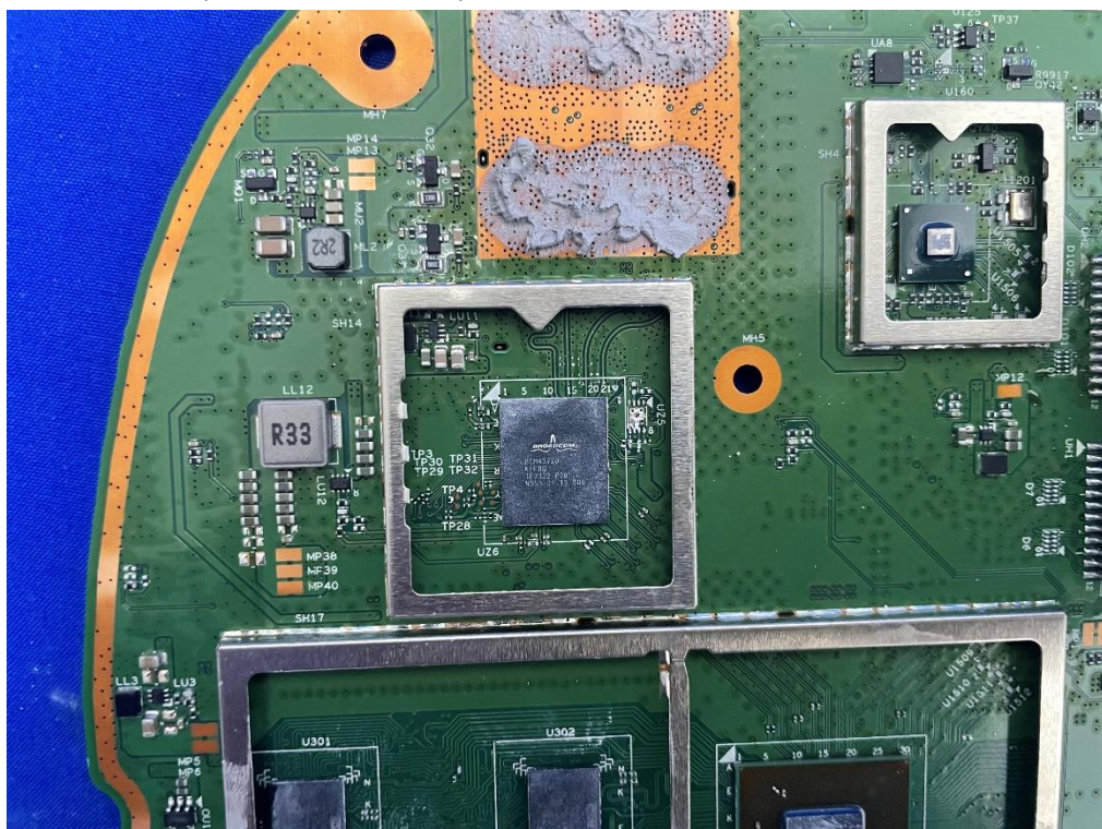
(10) EUT Photo (Model: APIN0734)
