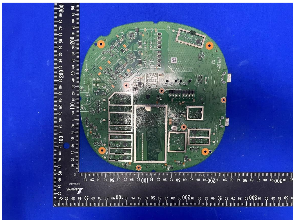
(14) EUT Photo (Model: APIN0734)
