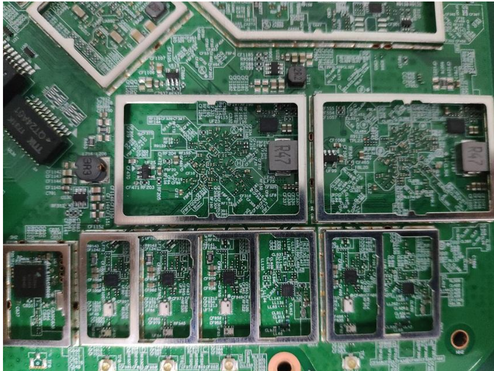
(26) EUT Photo (APIN0515)
