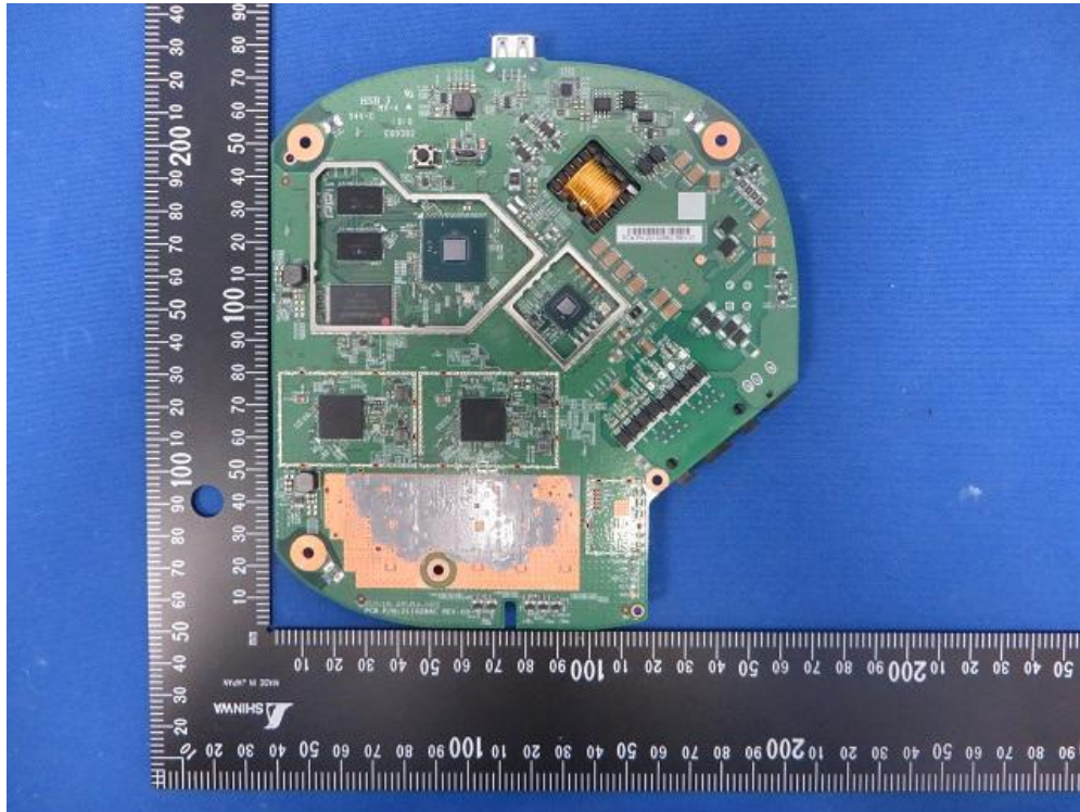
(21) EUT Photo (APIN0515)
