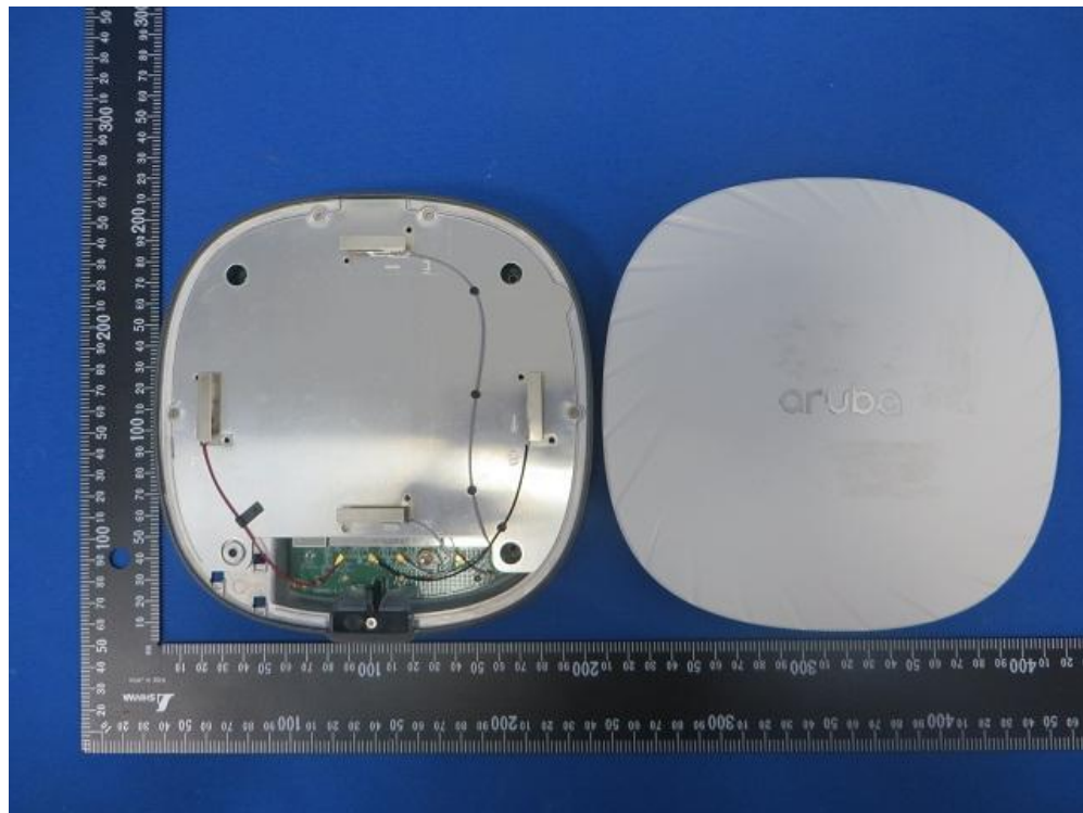
(15) EUT Photo (APIN0515)
