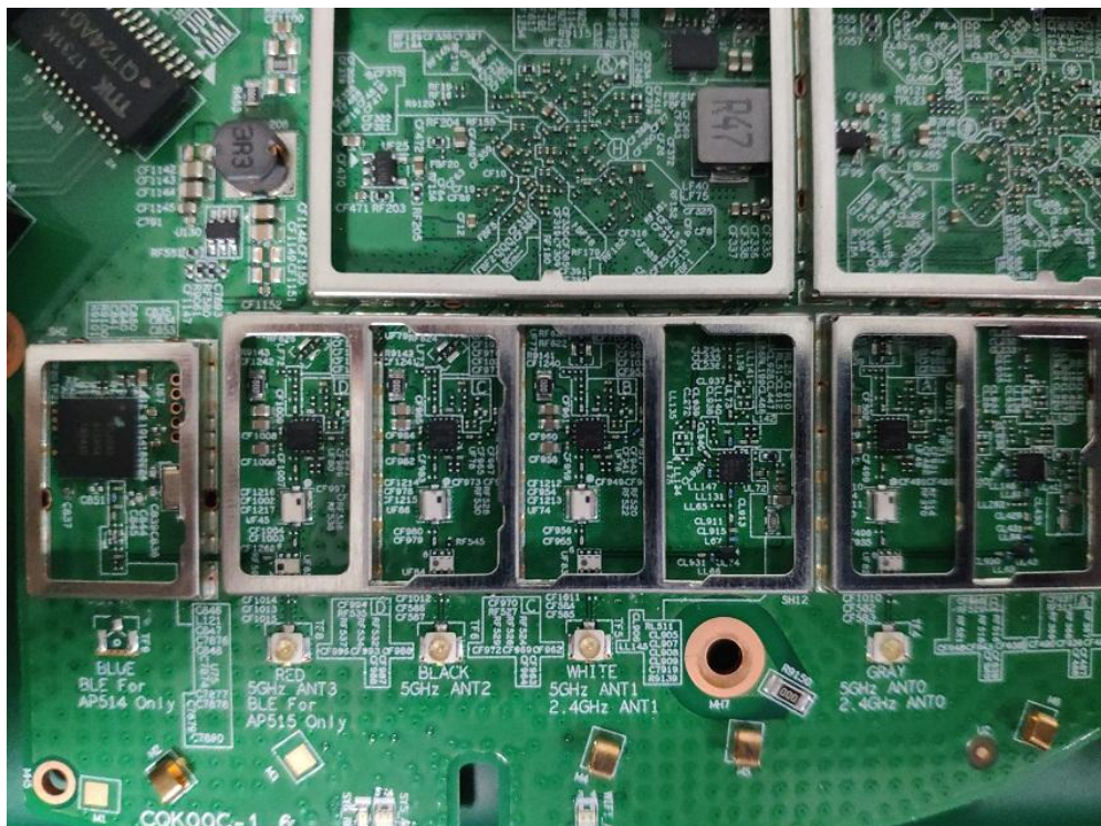
(28) EUT Photo (APIN0515)
