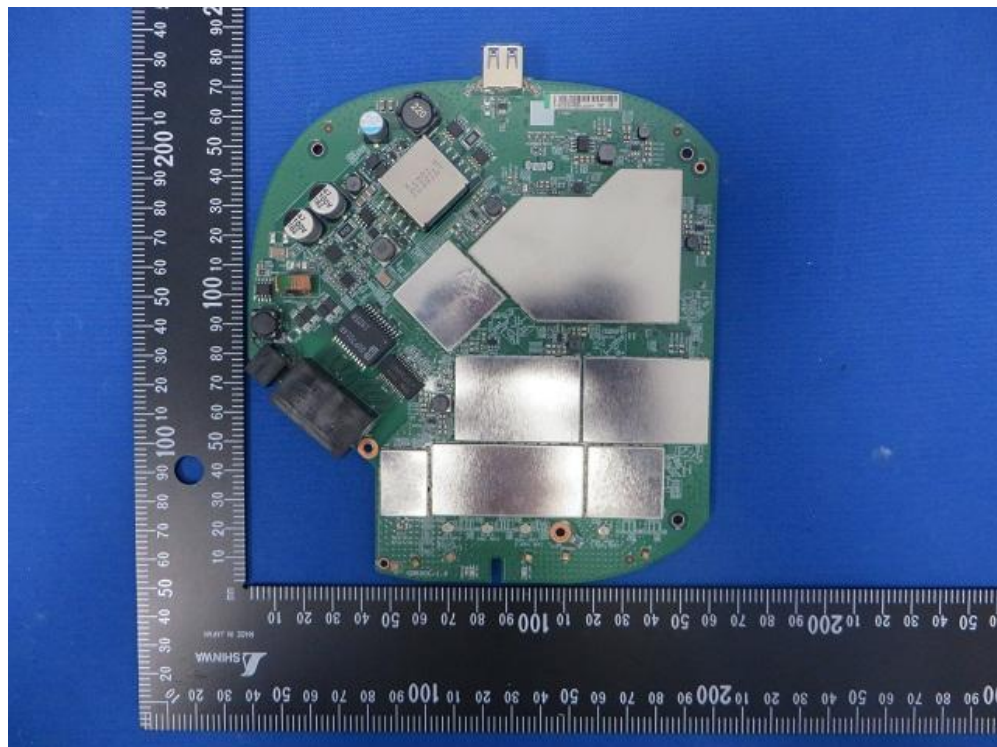
(18) EUT Photo (APIN0515)
