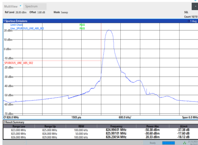
Band5-1.4MHz-QPSK-20427-6RB#0
