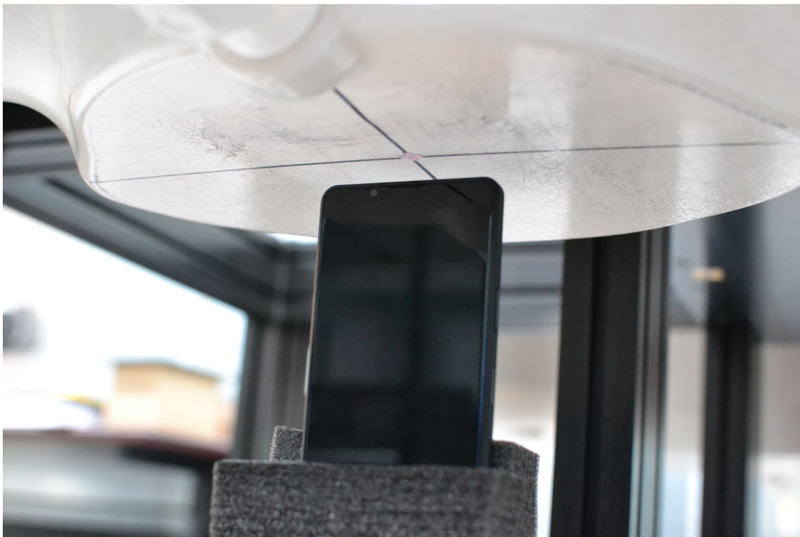
SAR Test Setup Photo 9 – Hotspot, Top Edge, 10 mm
