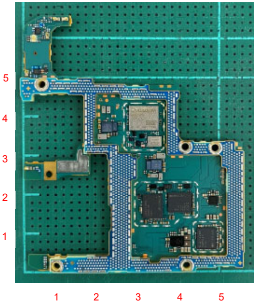
Internal Main-PWB Rear without Shield case (Front-side)
