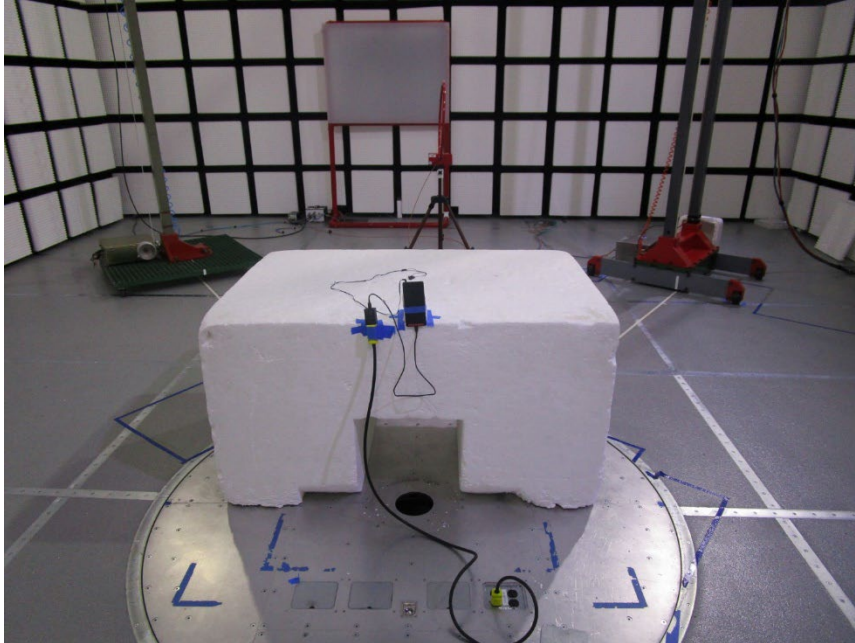
RADIATED PHOTO (<30 MHz WLAN MIMO)
