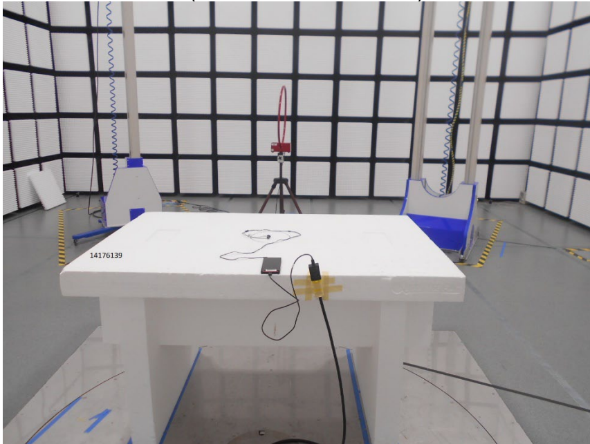
RADIATED PHOTO (<30 MHz BT/BLE ANT 1)
