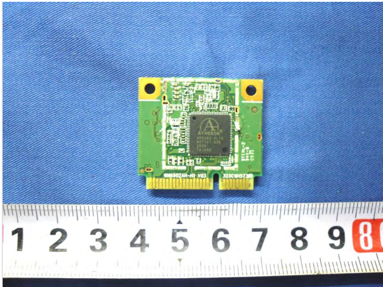
EUT: WLAN module (Atheros / AR5BHB92)
