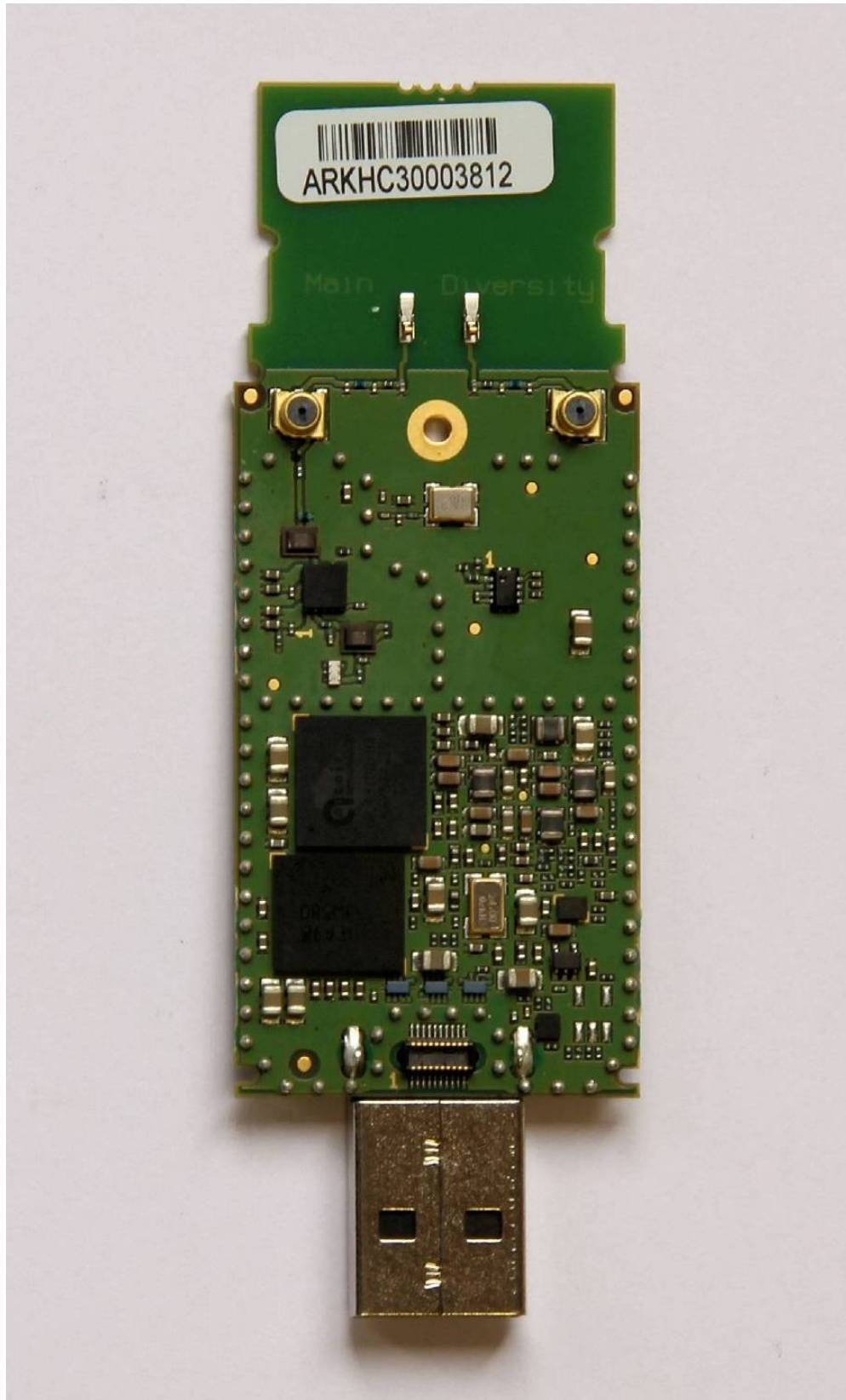
Figure 9: Main Board Bottom – Shield Removed
