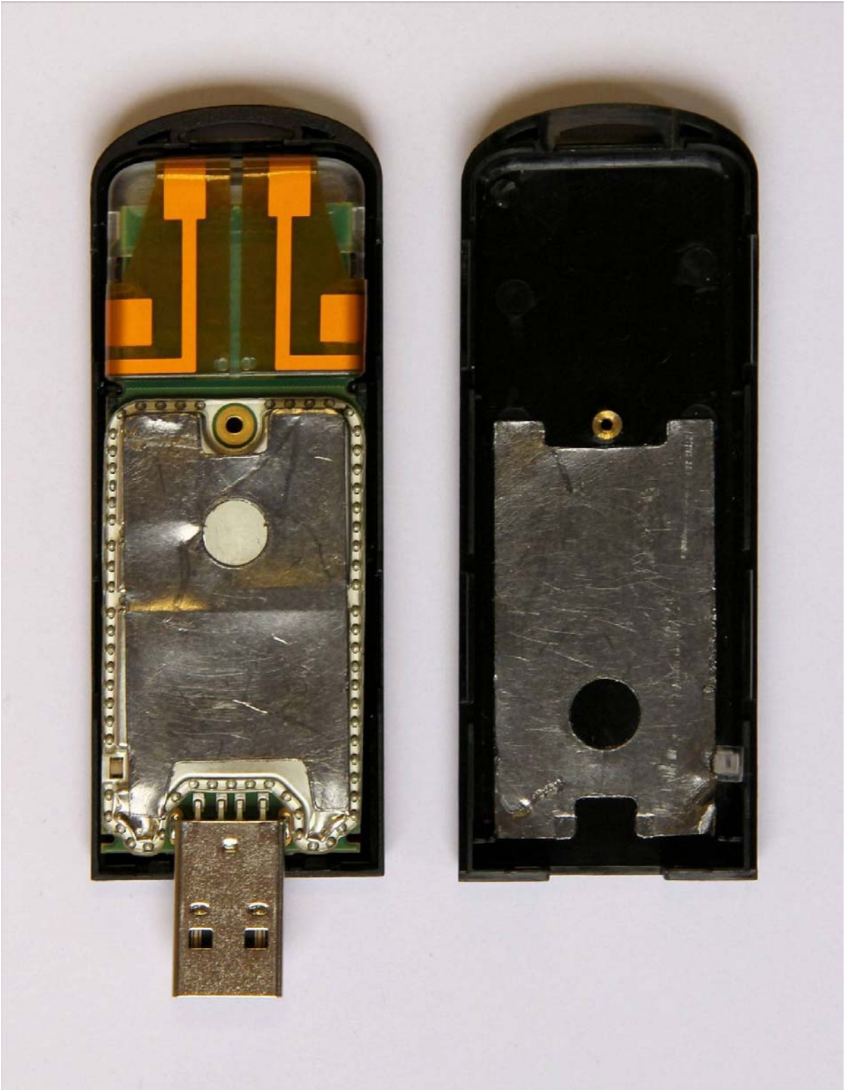
Figure 1: Top Cover Removed
