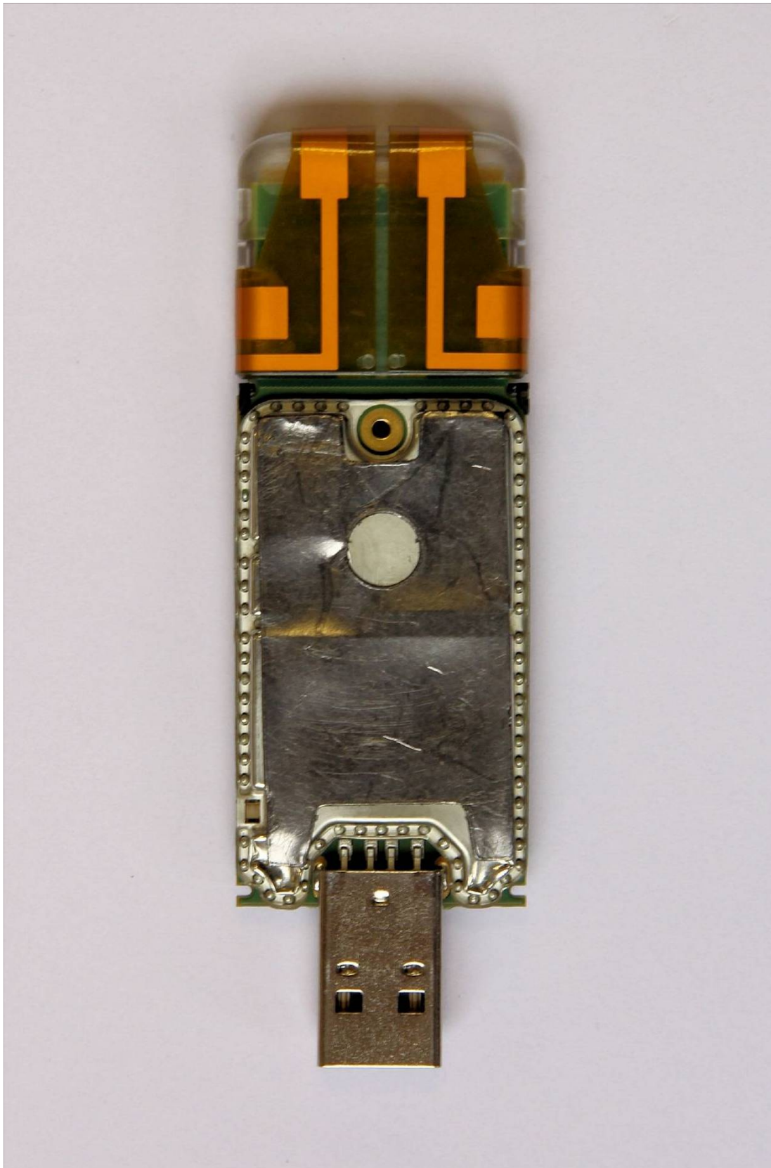
Figure 3: Top of Main Board with Shield and Antenna
