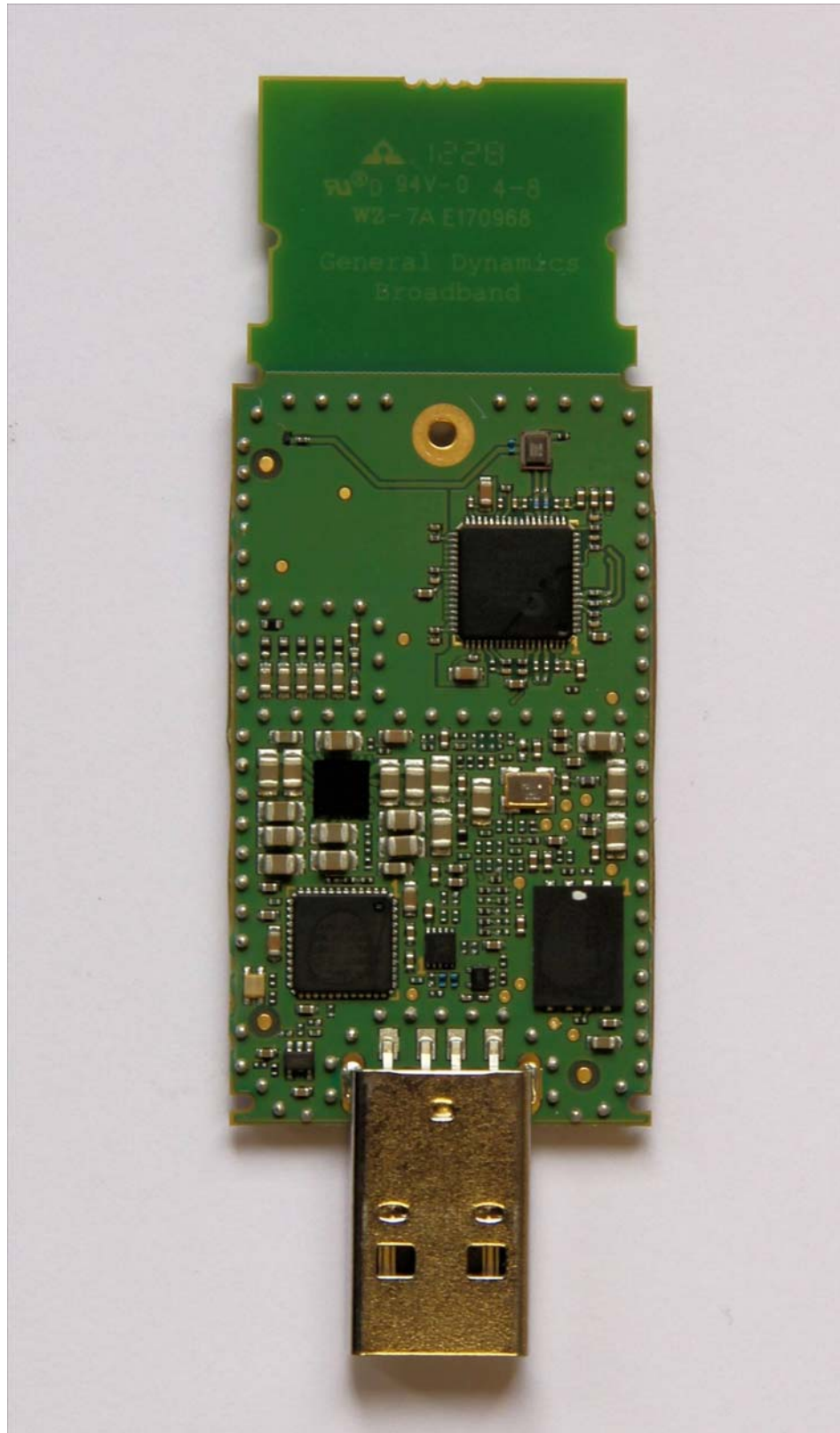
Figure 8: Main Board Top - Shield Removed
