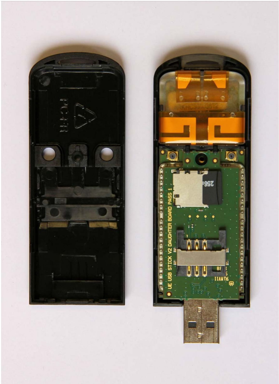
Figure 2: Bottom Cover Removed
