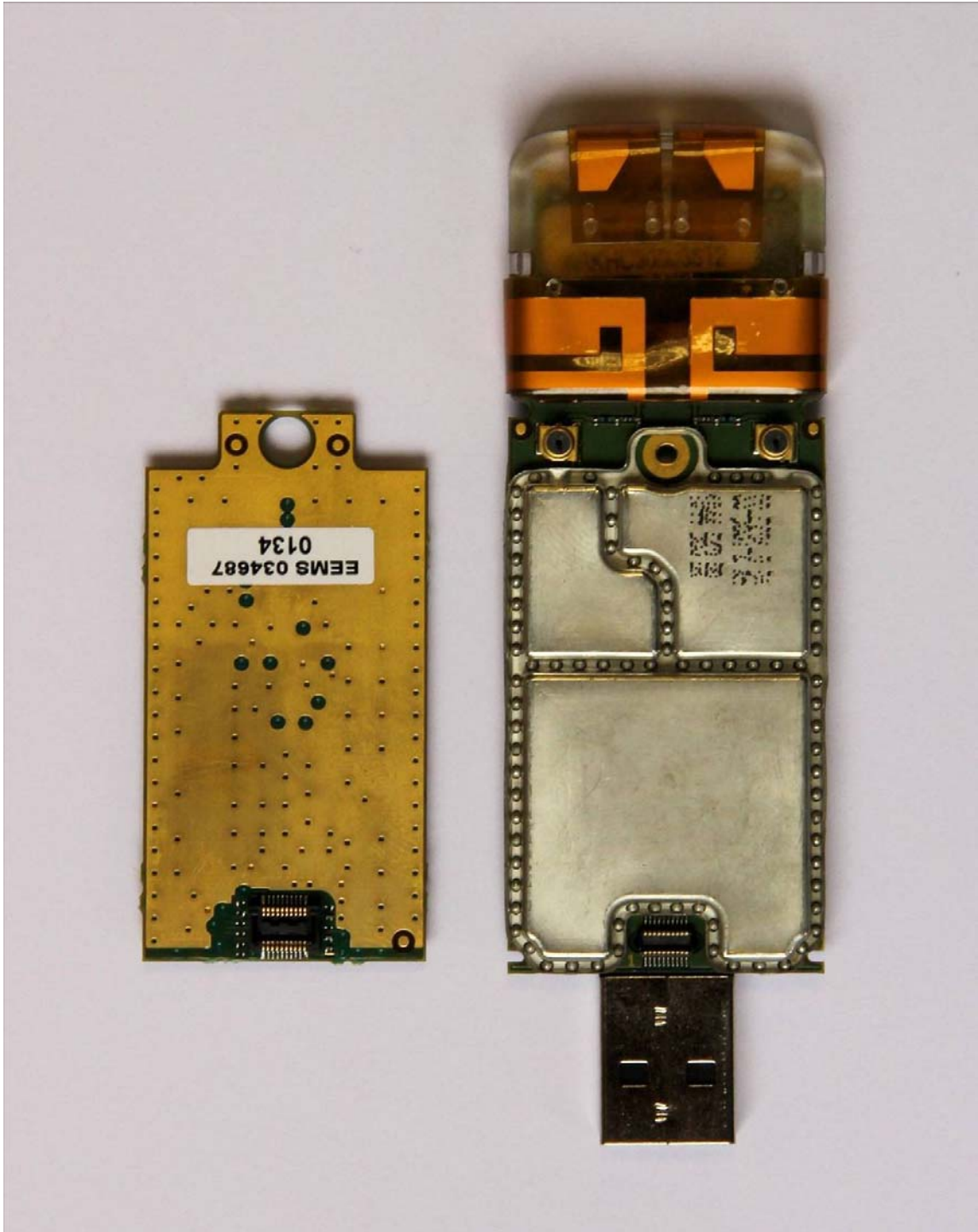
Figure 5: Bottom with Daughter Card Removed
