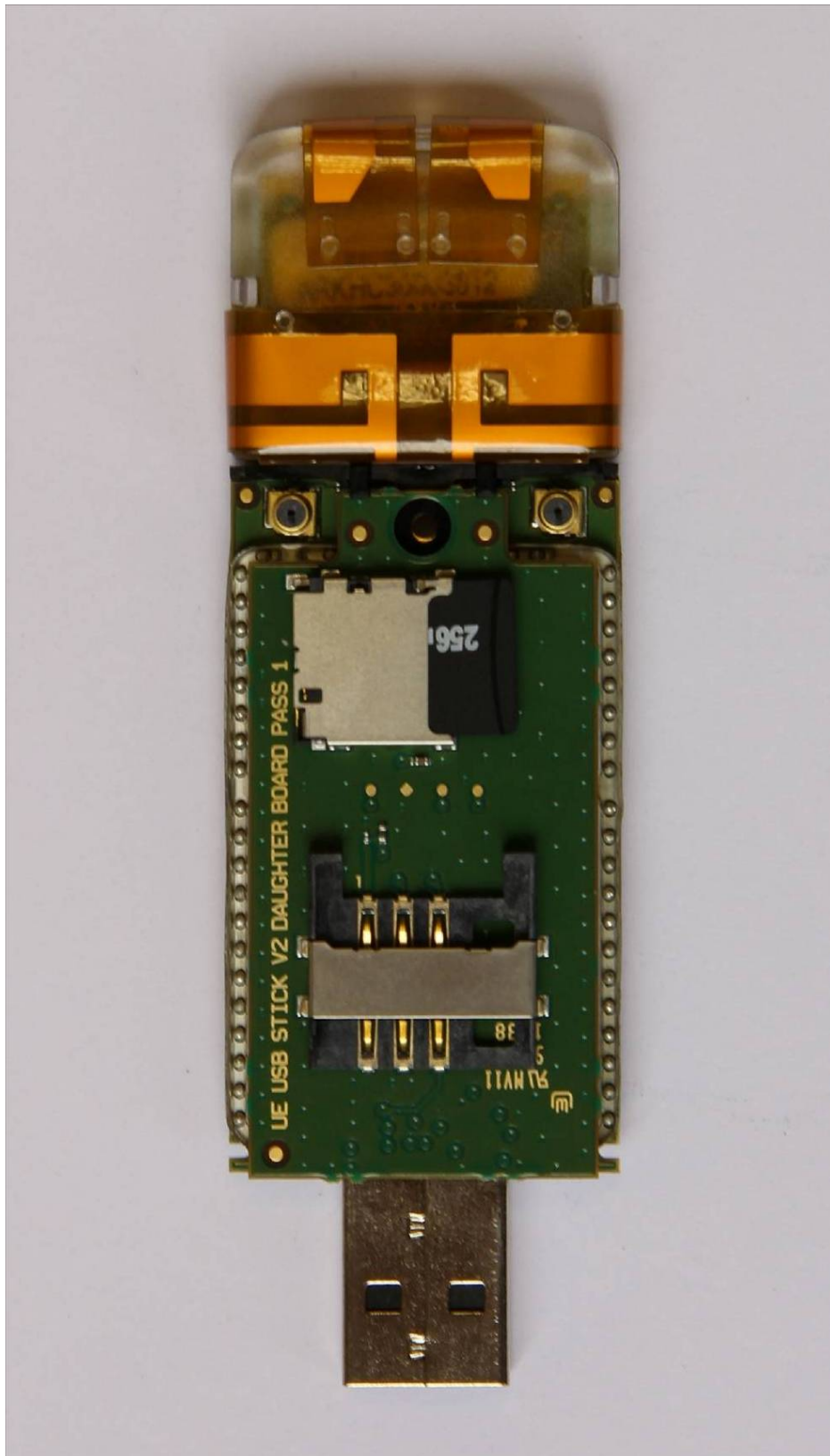
Figure 4: Bottom with Daughter card Fitted
