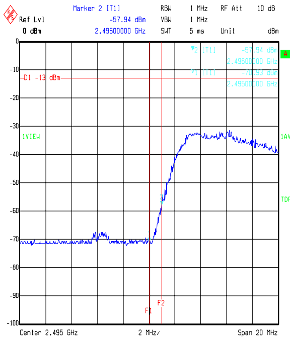
Title: 49131JD01 FCC PART 27 Comment A: TX RADIATED EMISSIONS LOWER BAND EDGE AVG DET Date: 03.JUL.2007 14:16:43
