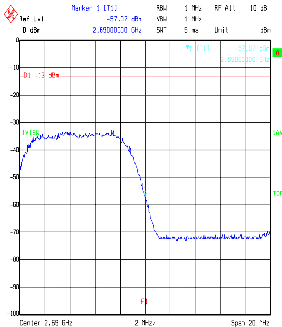
Title: 49131JD01 FCC PART 27 Comment A: TX RADIATED EMISSIONS UPPER BAND EDGE AVG DET Date: 03.JUL.2007 14:34:27
