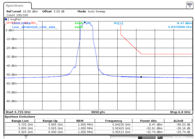
BE-NR-HIGH, MIMO-B, 802.11n20-HT8, Ch169
