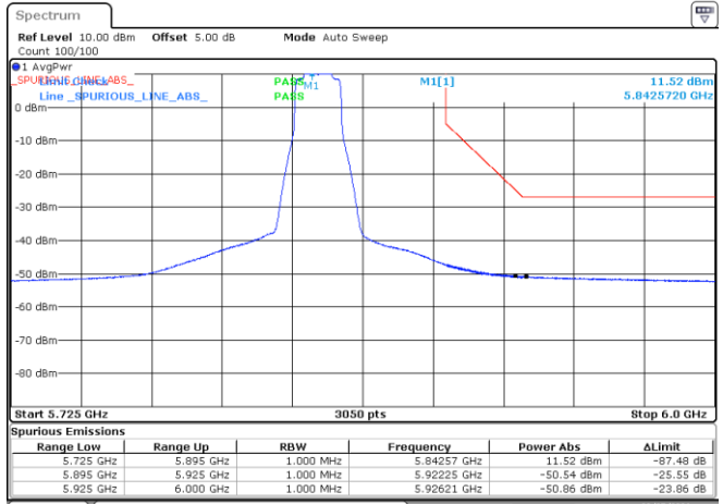
BE-NR-HIGH, SISO-B, 802.11n20-HT0, Ch169
