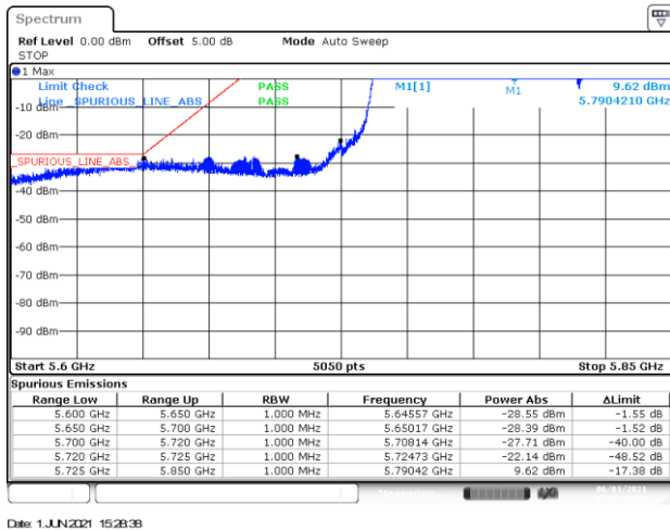
BE-NR-LOW, SISO-A, 802.11ac160-VHT0, Ch163
