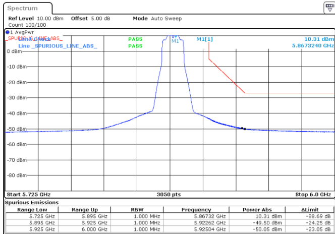
BE-NR-HIGH, SISO-B, 802.11n20-HT0, Ch173
