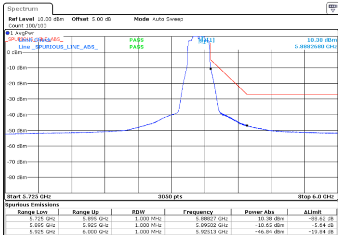
BE-NR-HIGH, SISO-B, 802.11n20-HT0, Ch177
