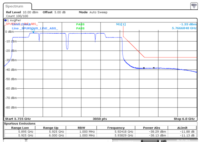
BE-NR-HIGH, MIMO-A, 802.11ac160-VHT0, Ch163
