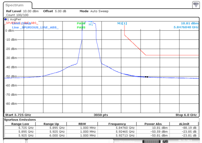
BE-NR-HIGH, SISO-B, 802.11ax20-HE0, Ch169
