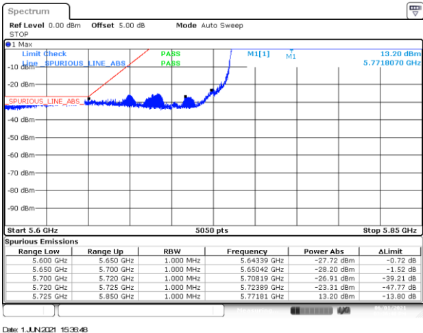
BE-NR-LOW, SISO-A, 802.11ax160-HE0, Ch163
