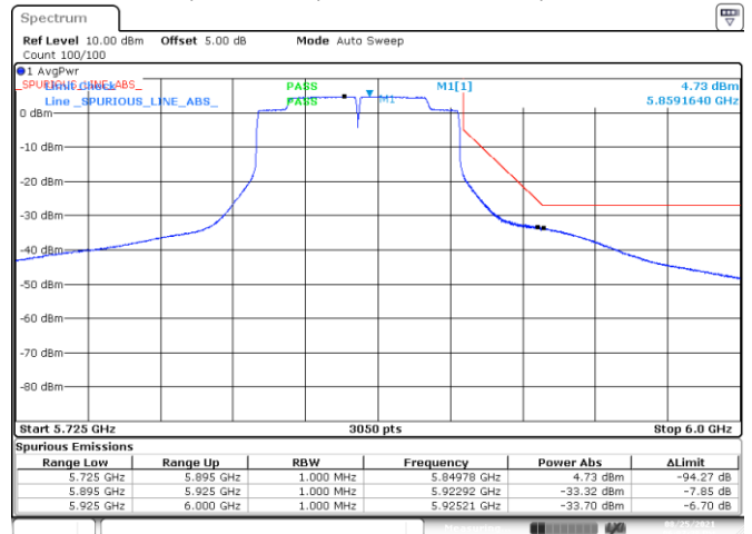
BE-NR-HIGH, MIMO-A, 802.11ac80-VHT0, Ch171
