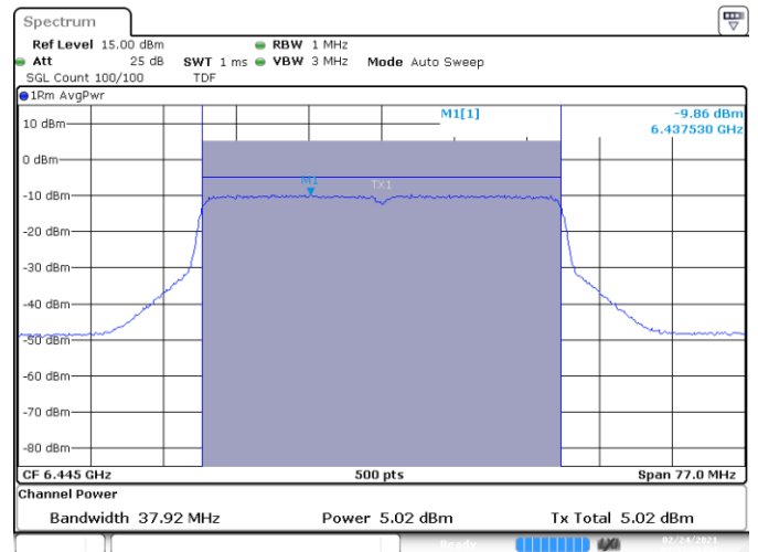
MIMO B-802.11ax-40MHz-Ch99-6445MHz-HE0
