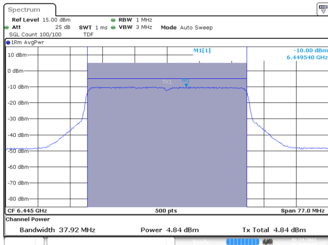
MIMO A-802.11ax-40MHz-Ch99-6445MHz-HE0
