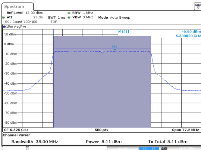
SISO A-802.11ax-40MHz-Ch115-6525MHz-HE0
