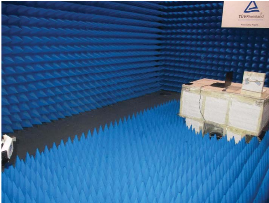
Photo 4: Photograph radiated emissions 26.5 – 36 GHz
