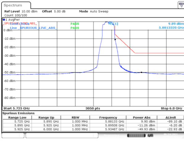
BE-NR-HIGH, MIMO-B, 802.11n20-HT8, Ch177
