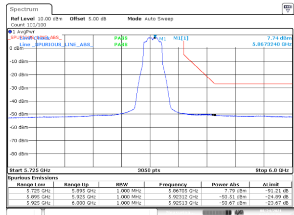
BE-NR-HIGH, MIMO-A, 802.11n20-HT8, Ch173
