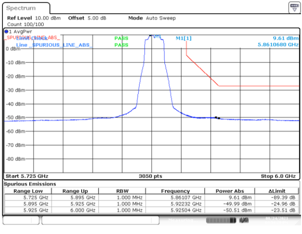
BE-NR-HIGH, MIMO-B, 802.11n20-HT8, Ch173
