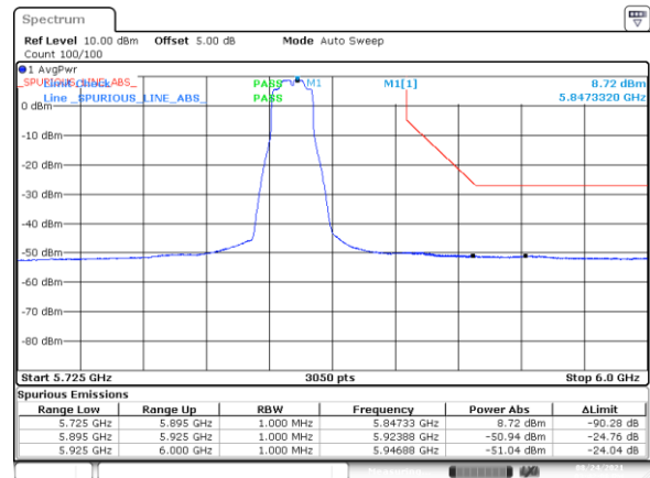
BE-NR-HIGH, MIMO-A, 802.11n20-HT8, Ch169
