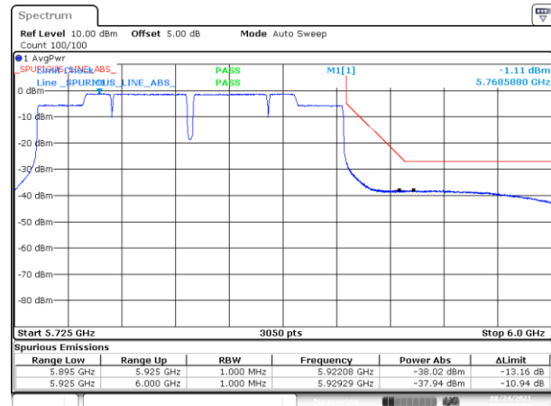
BE-NR-HIGH, MIMO-B, 802.11ac160-VHT0, Ch163
