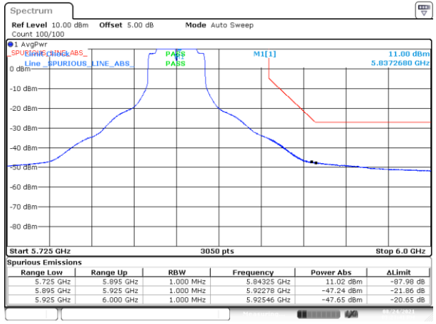
BE-NR-HIGH, SISO-A, 802.11n40-HT0, Ch167
