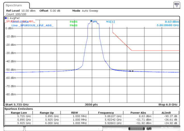
BE-NR-HIGH, MIMO-A, 802.11n20-HT8, Ch173
