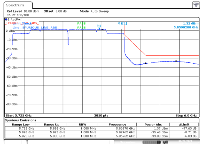
BE-NR-HIGH, SISO-B, 802.11ax160-HE0, Ch163
