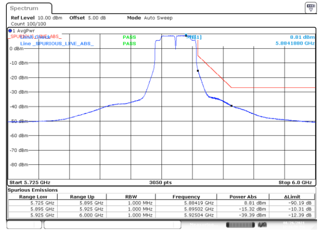
BE-NR-HIGH, MIMO-B, 802.11n40-HT8, Ch175
