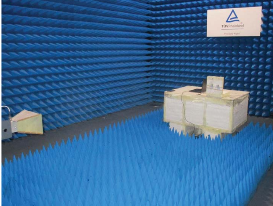
Photo 2 Photograph radiated emissions 1 – 18 GHz
