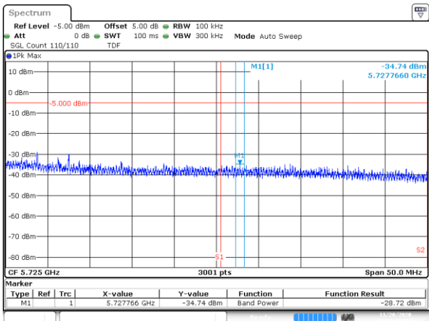
BE-NR-HIGH, DIV 2, 802.11ac80-VHT0, Ch122
