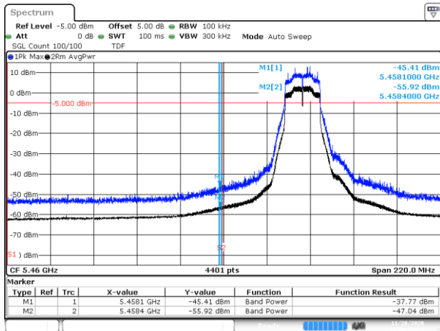
BE-R-LOW, DIV 2, 802.11n20-HT0, Ch100
