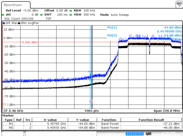
BE-R-LOW, DIV 1, 802.11ac80-VHT0, Ch106
