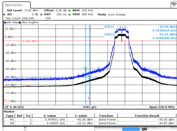
BE-R-LOW, DIV 1, 802.11n20-HT0, Ch100
