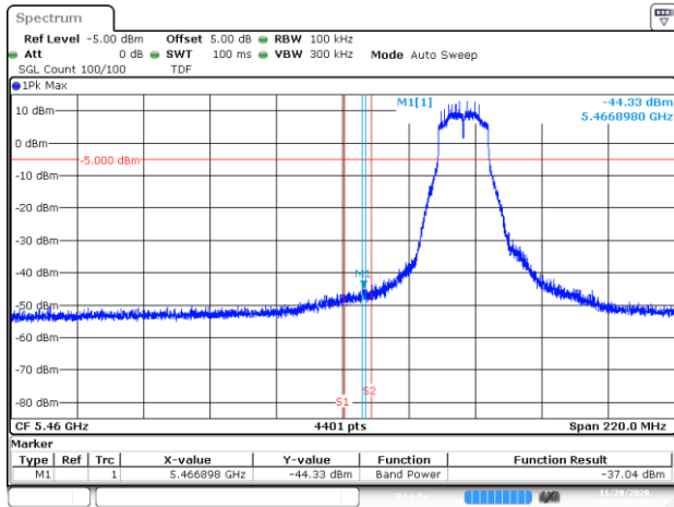
BE-NR-LOW, DIV 2, 802.11a20-6Mbps, Ch100
