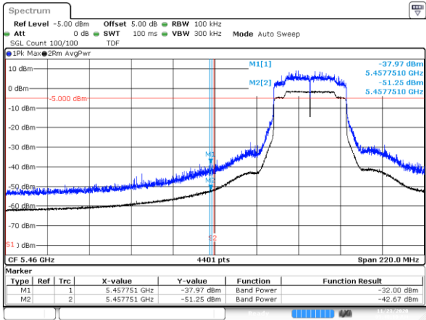
BE-R-LOW, DIV 2, 802.11ax40-HE0, Ch102
