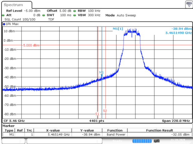
BE-NR-LOW, DIV 1, 802.11ax20-HE0, Ch100
