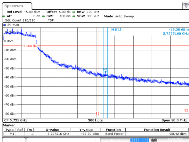
BE-NR-HIGH, DIV 2, 802.11n20-HT0, Ch140
