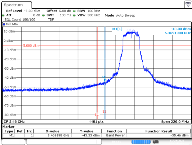
BE-NR-LOW, DIV 2, 802.11ax20-HE0, Ch100
