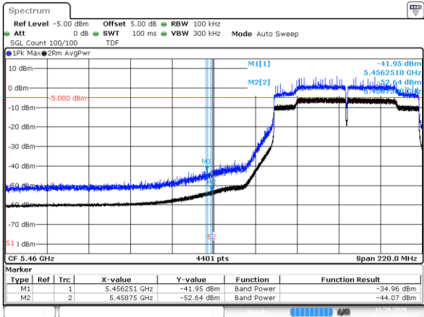
BE-R-LOW, DIV 2, 802.11ac80-VHT0, Ch106
