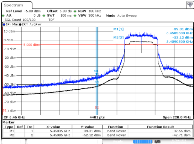
BE-R-LOW, DIV 1, 802.11ax40-HE0, Ch102
