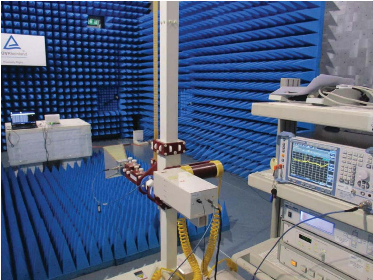
Photo 3: Photograph radiated emissions 6 – 18 GHz
