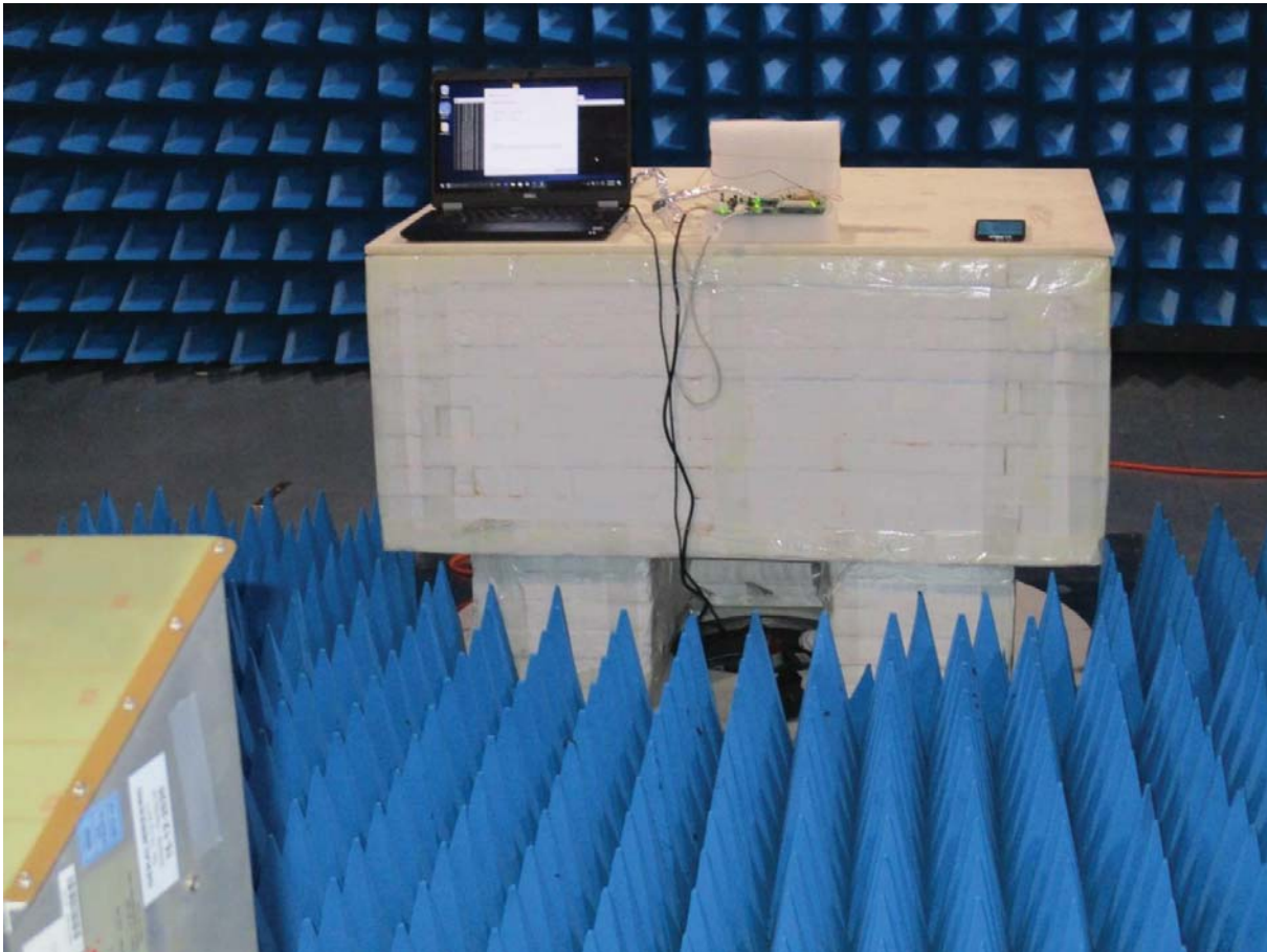
Photo 2: Photograph radiated emissions 1 – 6 GHz
