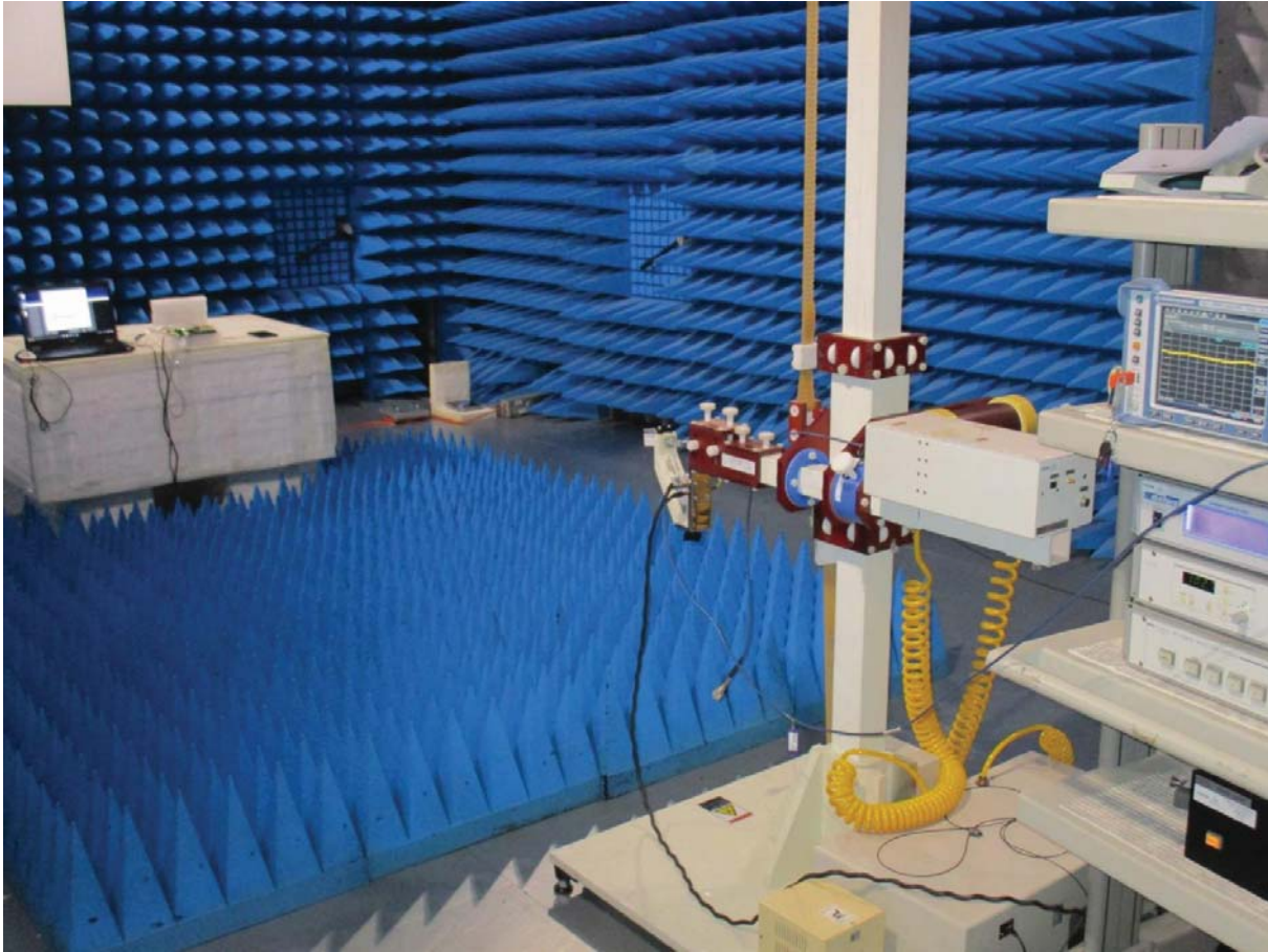
Photo 4: Photograph radiated emissions 18 – 30 GHz
