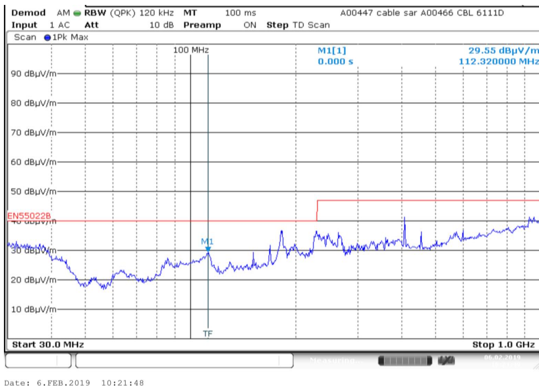
Plot 2: Pre-scan plot with peak detector. Radiated emissions from 30 MHz to 1000 MHz, 5GHz and BT mode.
