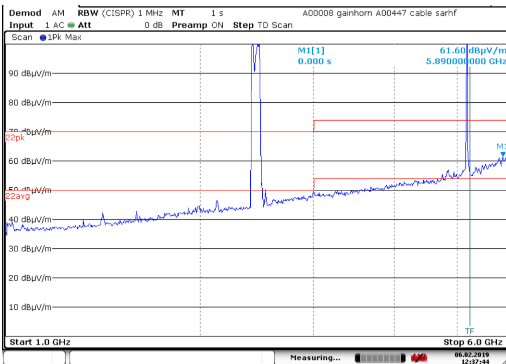
Plot 4: Pre-scan plot with peak detector. Radiated emissions from 1 GHz – 6 GHz, 5 GHz and BT mode
