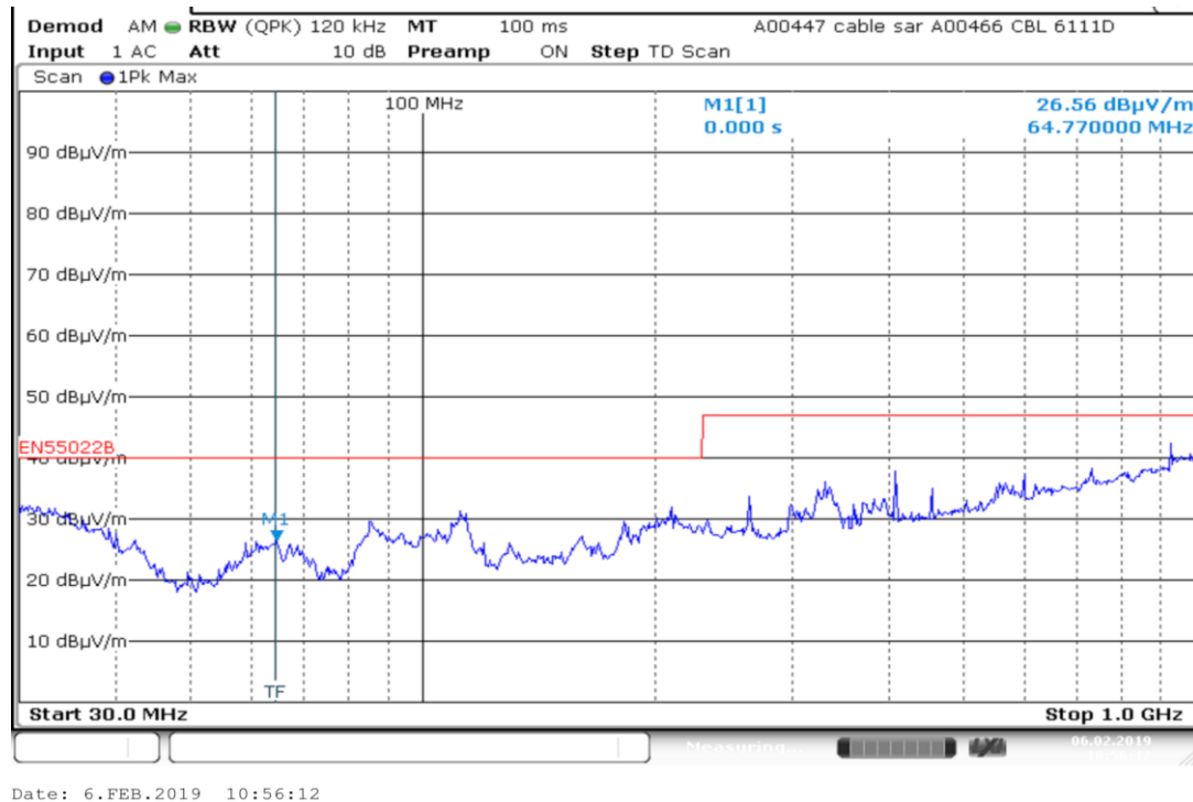
Plot 1: Pre-scan plot with peak detector. Radiated emissions from 30 MHz to 1000 MHz, 2.4GHz mode.
