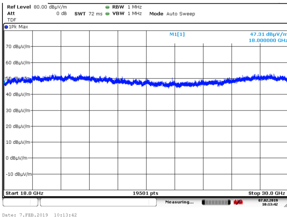
Plot 8: Pre-scan plot with peak detector. Radiated emissions from 18 GHz – 30 GHz, 5 GHz WIFI and BT mode
