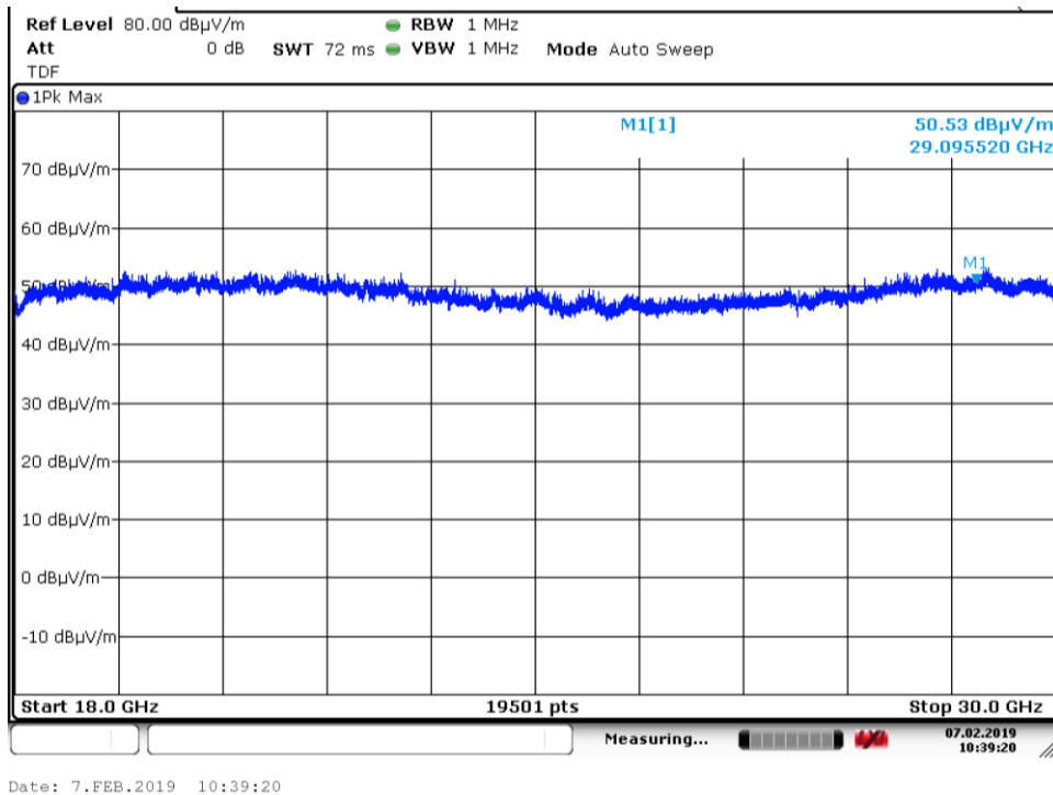
Plot 7: Pre-scan plot with peak detector. Radiated emissions from 18 GHz - 30 GHz, 2.4 GHz WIFI mode
