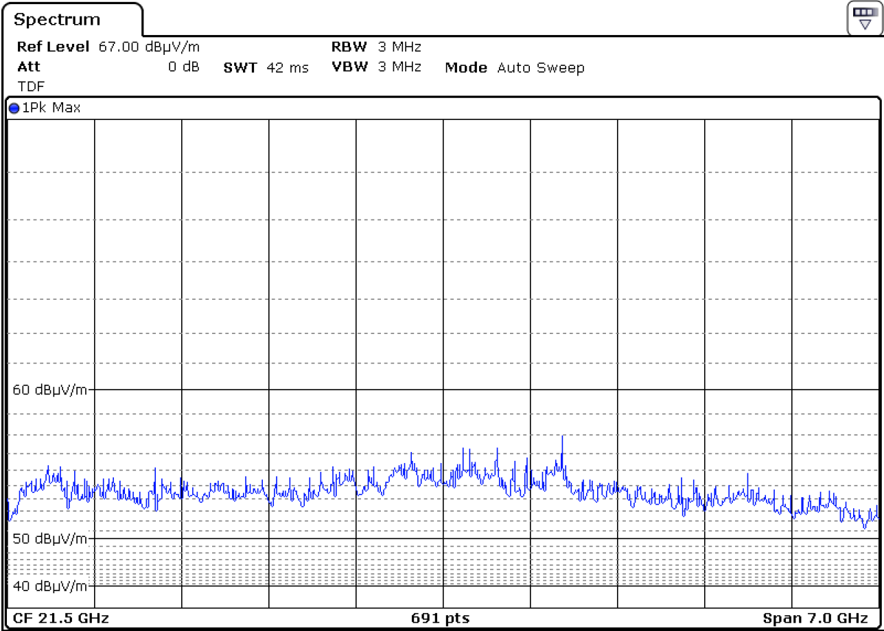
Plot 6: Pre-scan plot with peak detector. Radiated emissions from 18 GHz – 25 GHz. Noise peaks are only EUT Related if mentioned in the tables in Clause 3.2
