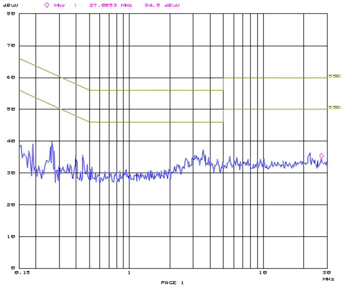
Plot 8: Pre-scan plot with peak detector. Conducted emissions from 0.15 - 30 MHz.
