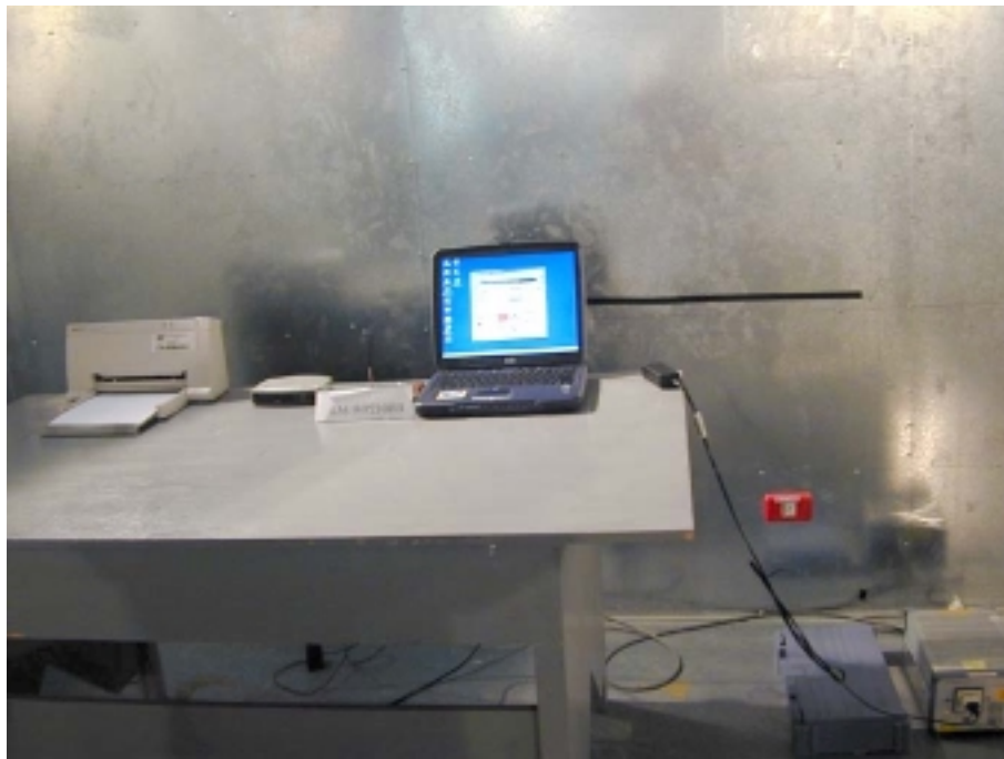
Photo 1: Conducted set-up photo (front)
