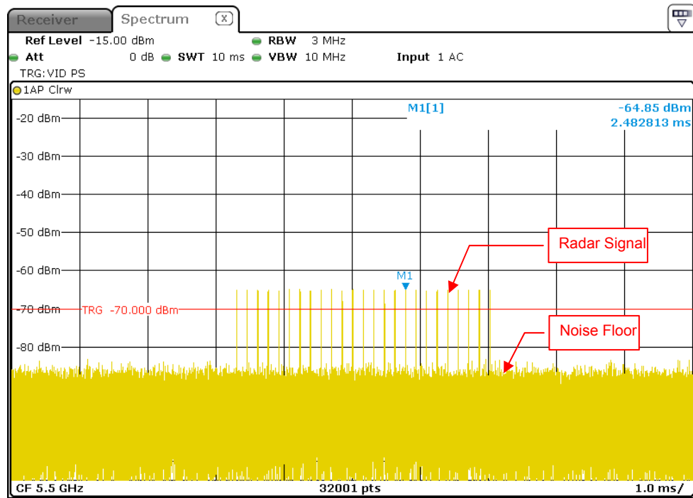
Radar Signal 2
