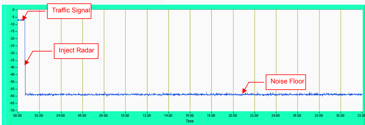
802.11n 20M Result: Pass
