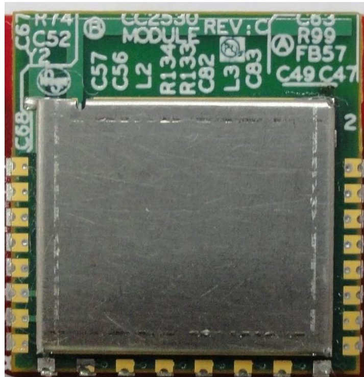
EUT Top View
