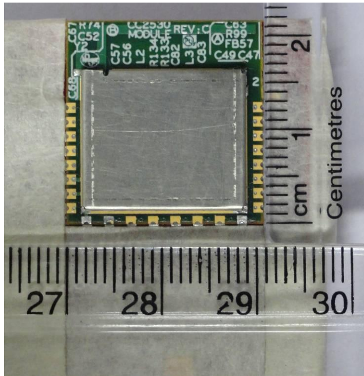
EUT Dimensional View
