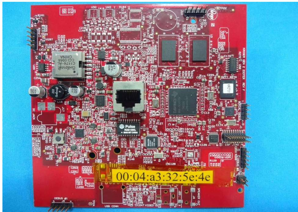
Bottom View of the internal PCB
