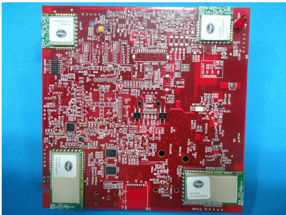
Top View of the Internal PCB
