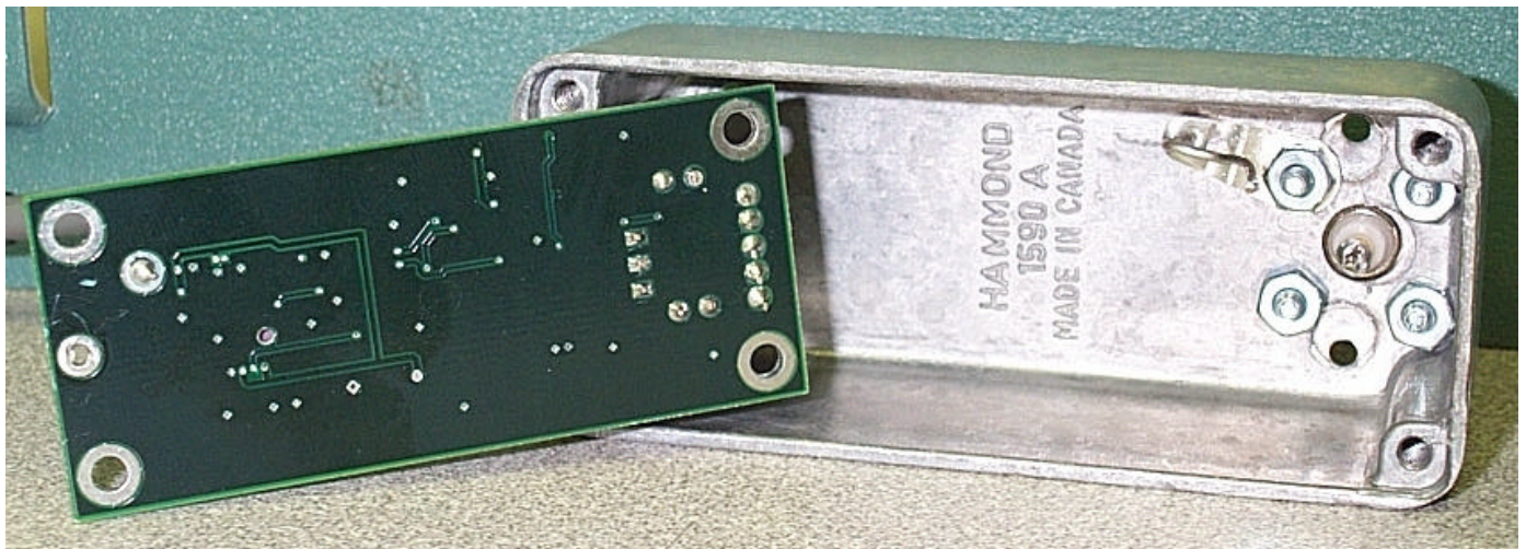
RF PCB and case
