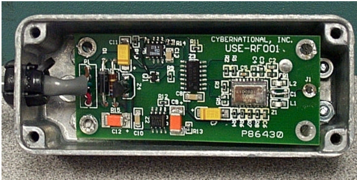
RF PCB
