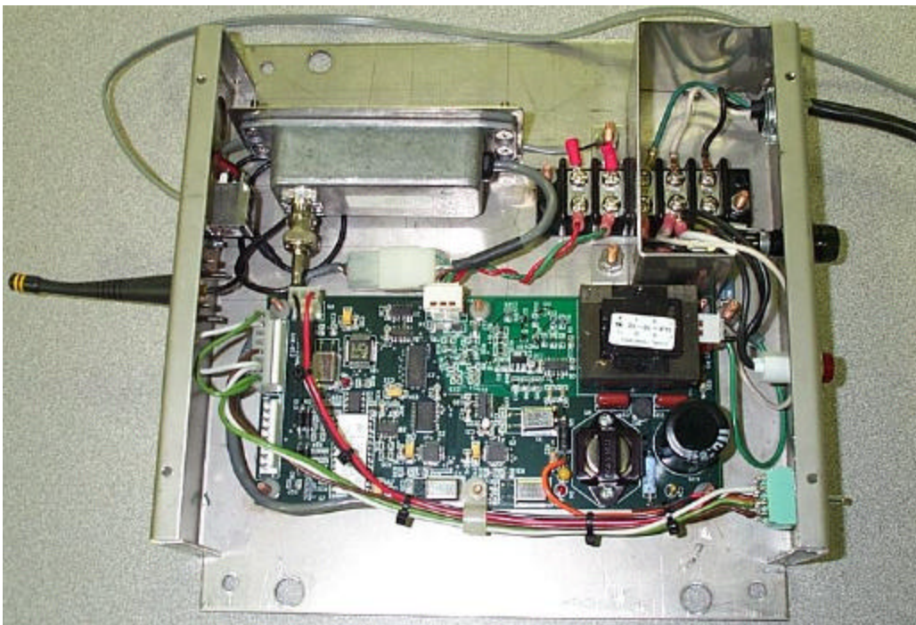
Full system; Case open
