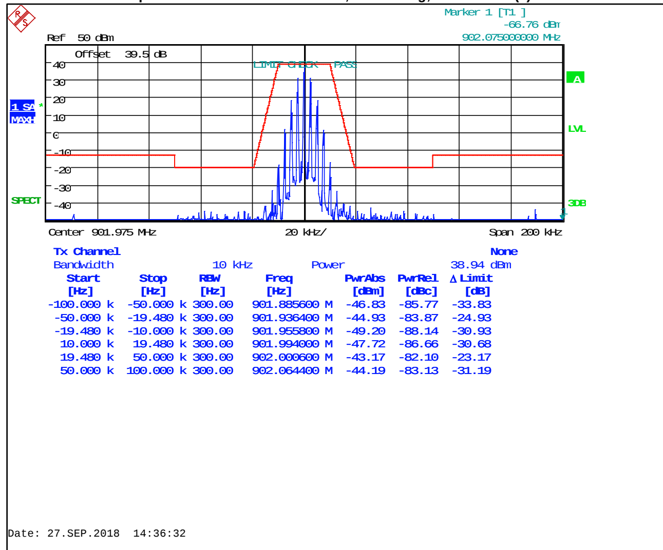
Plot 7-2: Occupied Bandwidth – 901.9750 MHz; WB Analog; Mask 24.133(1)
