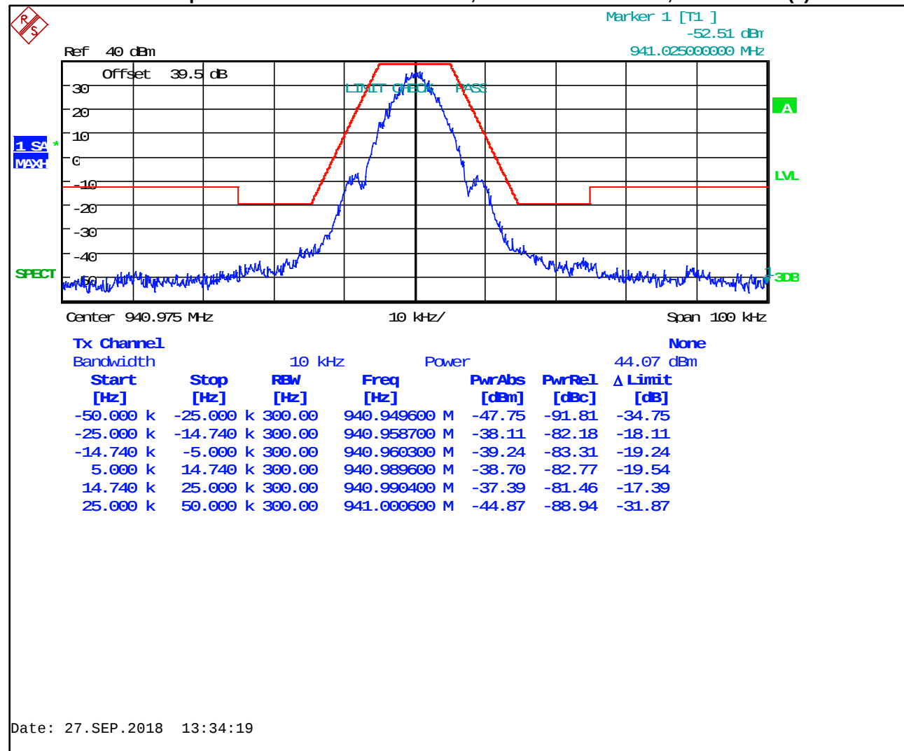
Plot 7-11: Occupied Bandwidth – 940.9750 MHz; 2-Level FSK 9600 NB; Mask 24.133(2)
