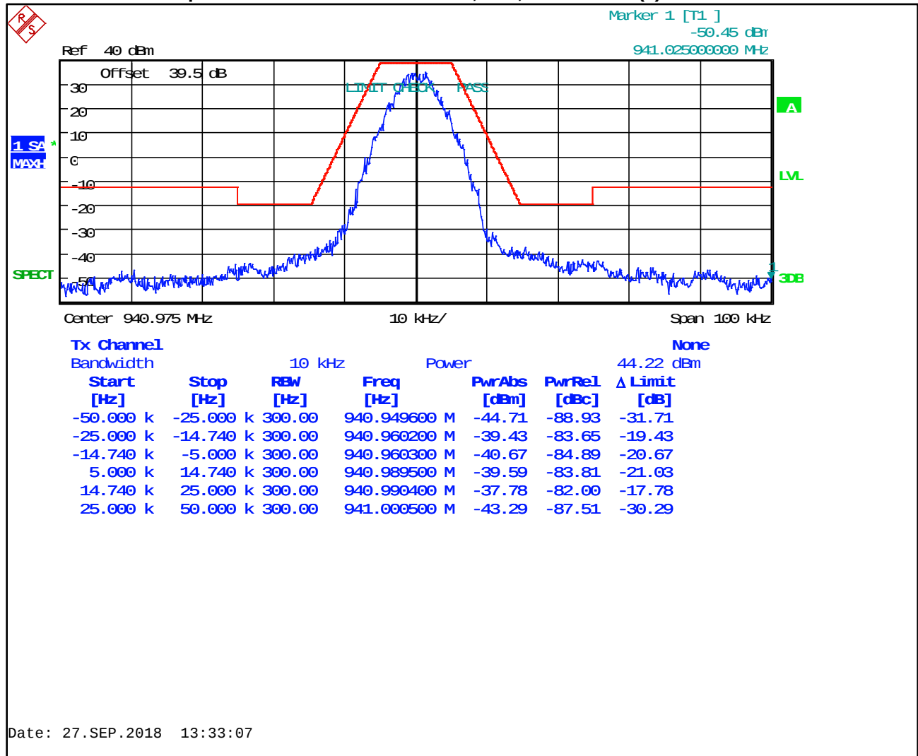
Plot 7-13: Occupied Bandwidth – 940.9750 MHz; P25; Mask 24.133(2)
