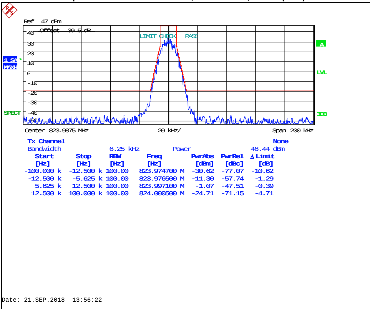
Plot 8-108: Occupied Bandwidth – 823.9875 MHz; HVD NPSPAC; Mask D (ISED)
