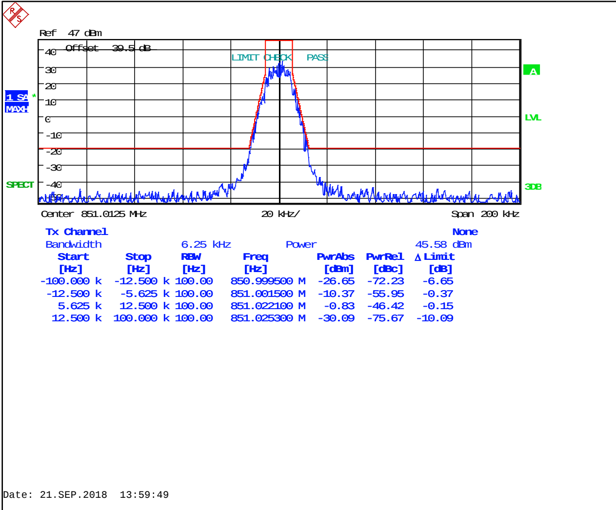
Plot 8-110: Occupied Bandwidth – 851.0125 MHz; HVD NPSPAC; Mask D (ISED)
