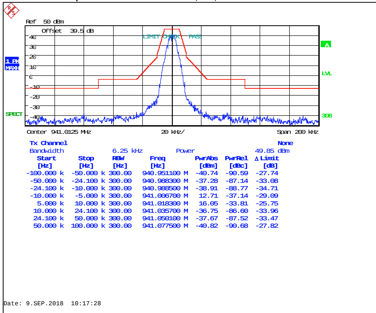
Plot 8-78: Occupied Bandwidth – 941.0125 MHz; P25; Mask C
