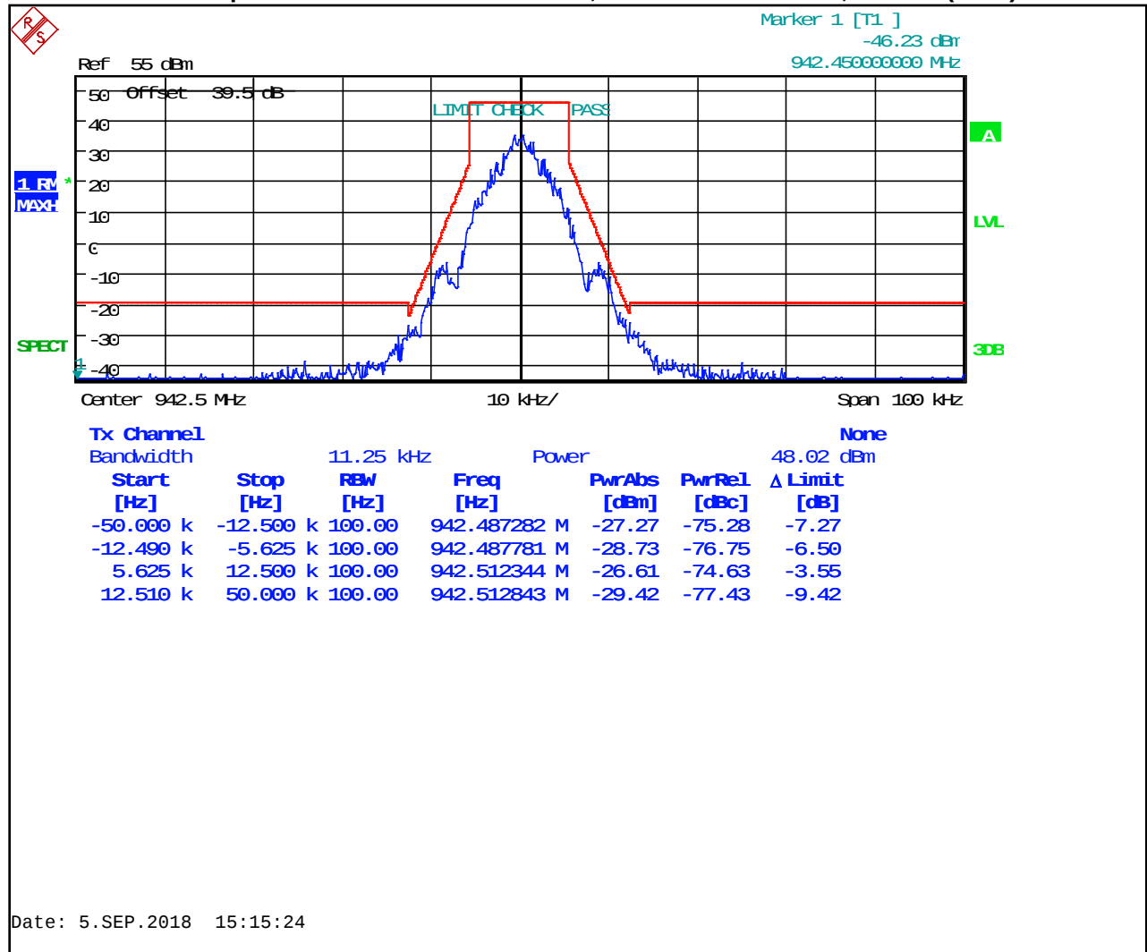
Plot 8-53: Occupied Bandwidth – 942.5000 MHz; 2-Level FSK 9600 NB; Mask D (ISED)
