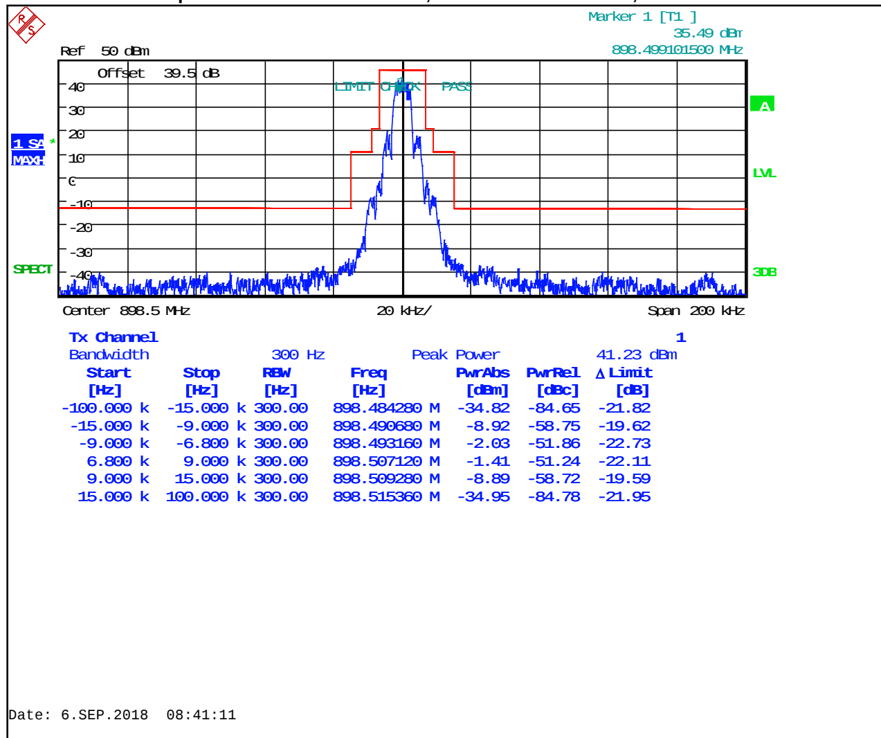
Plot 8-57: Occupied Bandwidth – 898.5 MHz; 2-Level FSK 4800 XNB; Mask J
