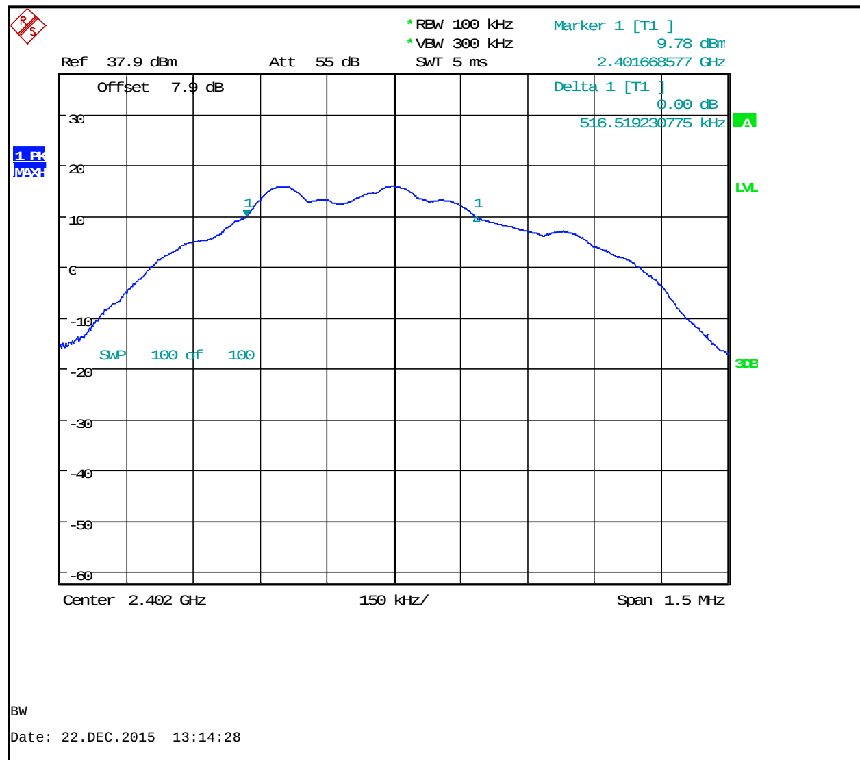
Plot 7-1: 6 dB Bandwidth – 2402 MHz
