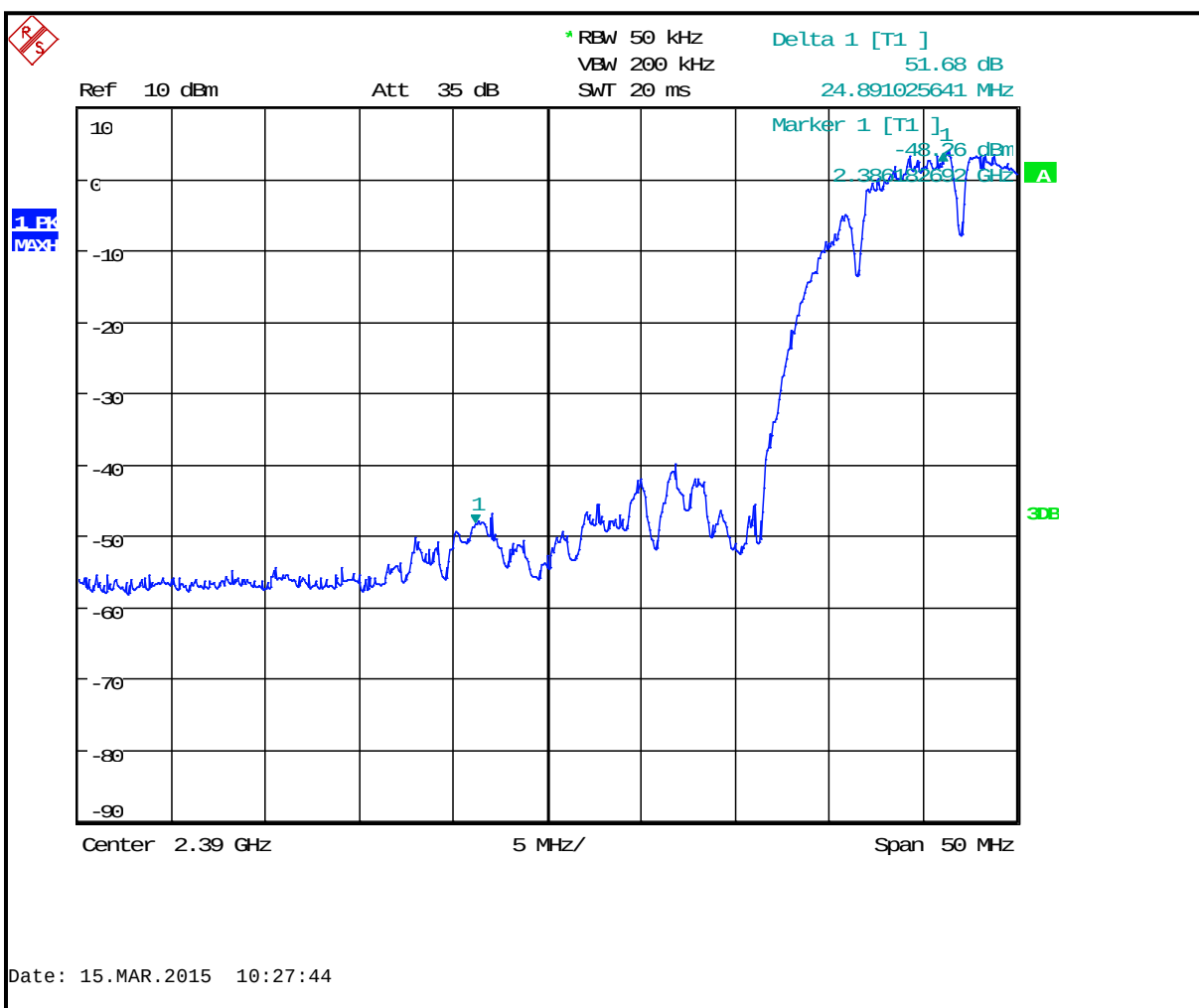
Plot 4-1: In Band Emissions - Channel 1 (2412 MHz); 802.11b (2 Mbps)
