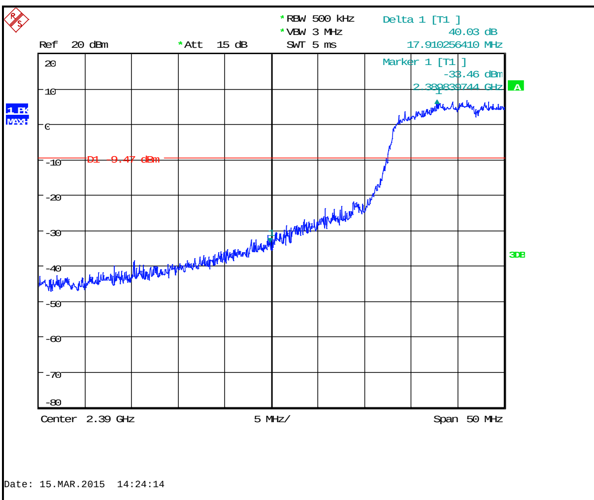
Plot 4-5: In Band Emissions - Channel 1 (2412 MHz); 802.11n (65 Mbps)
