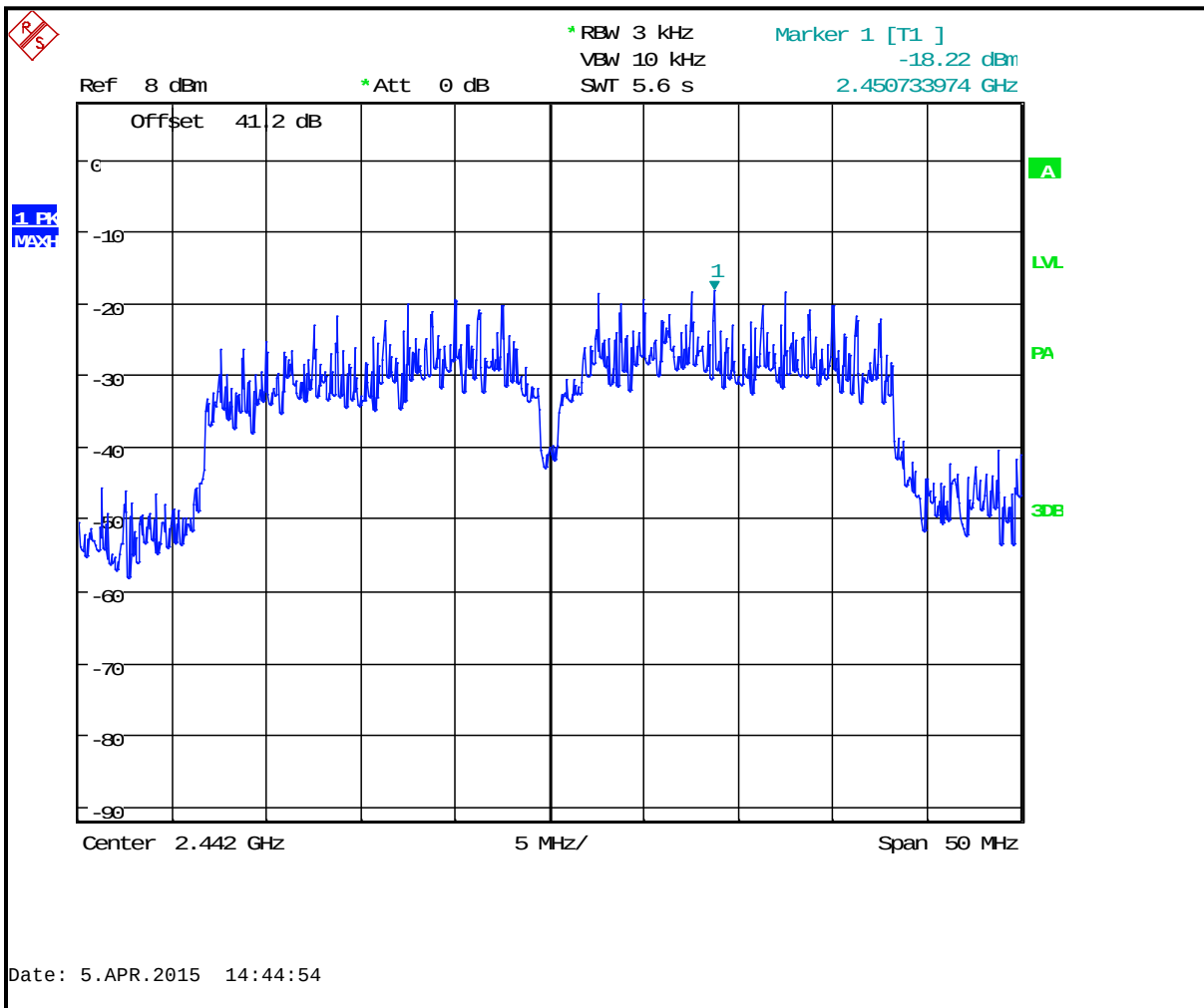
Plot 7-10: Power Spectral Density: Channel 5 (2442 MHz); 802.11n (40MHz BW)
