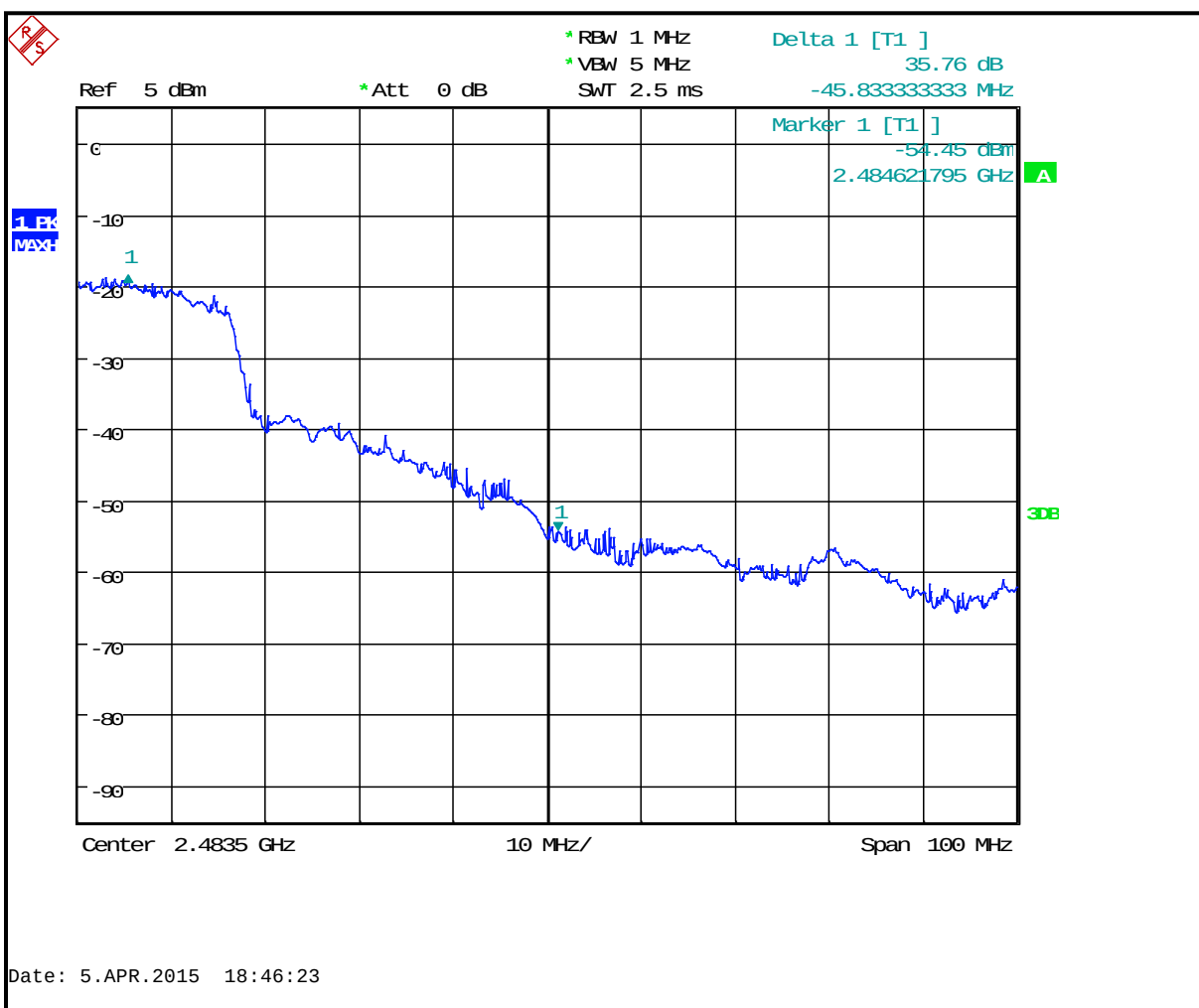
Plot 4-8: In Band Emissions - Channel 7 (2432 MHz); 802.11n (40 MHz)
