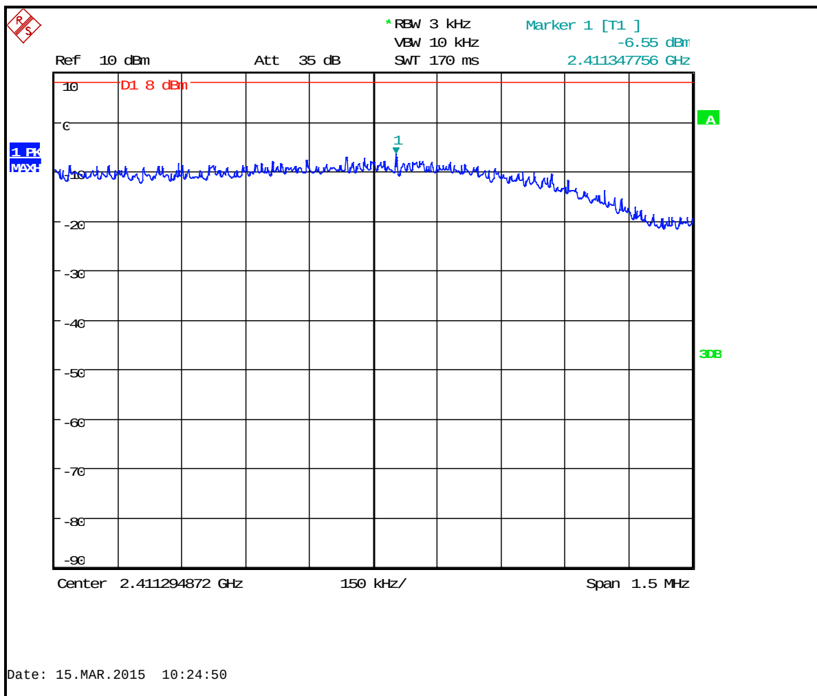
Plot 7-1: Power Spectral Density: Channel 1 (2412 MHz); 802.11b (2 Mbps)
