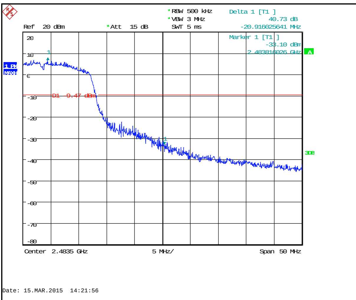
Plot 4-6: In Band Emissions - Channel 11 (2462 MHz); 802.11n (65 Mbps)
