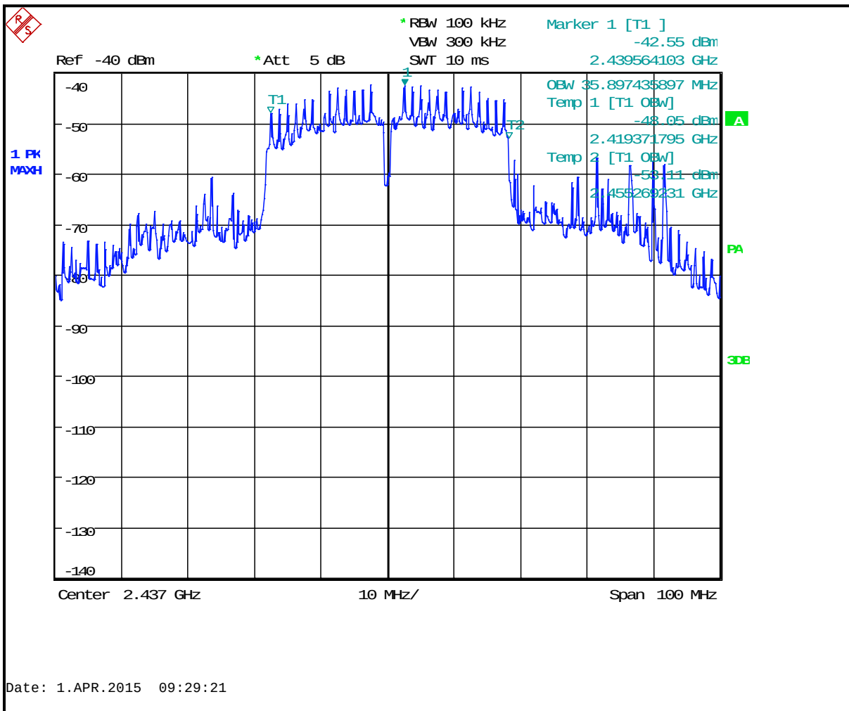
Plot 6-10: 6 dB Bandwidth Channel 8 (TX Frequency 2437 MHz-40 MHz BW) - 802.11n
