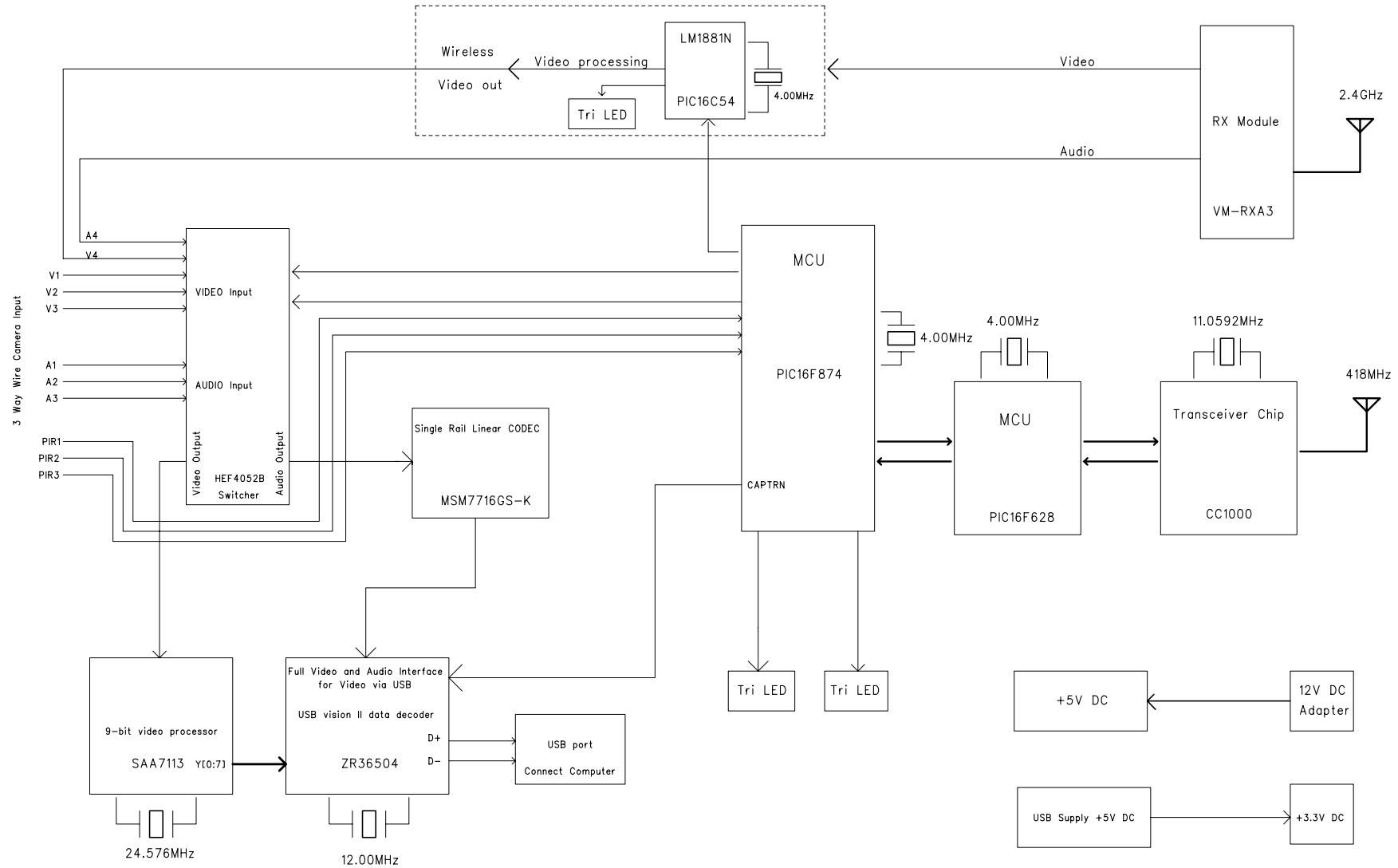
Figure 1. XBX300 Diagram block
