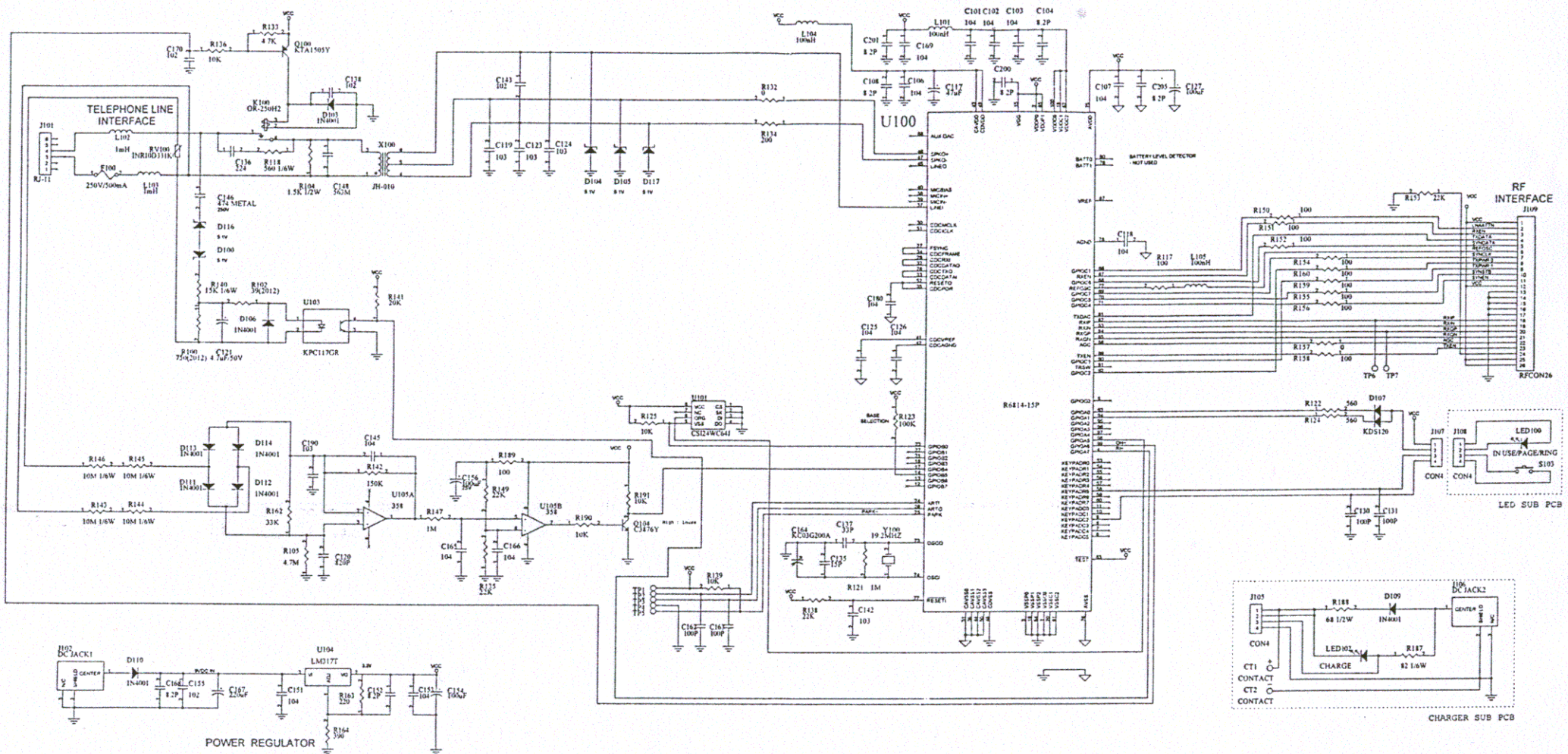
SCHEMATIC IBM3920 DSST BASEUNIT SIZE A3 DATE 27/Feb/2001 DOCUMENT NO IBM3920B 00 SCALE NONE SHEET 1 OF 4
