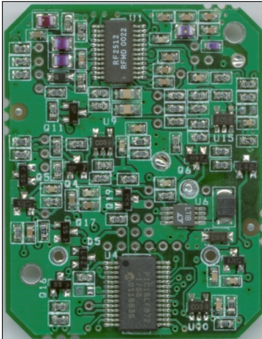
Figure 2: Internal PCB Top view
