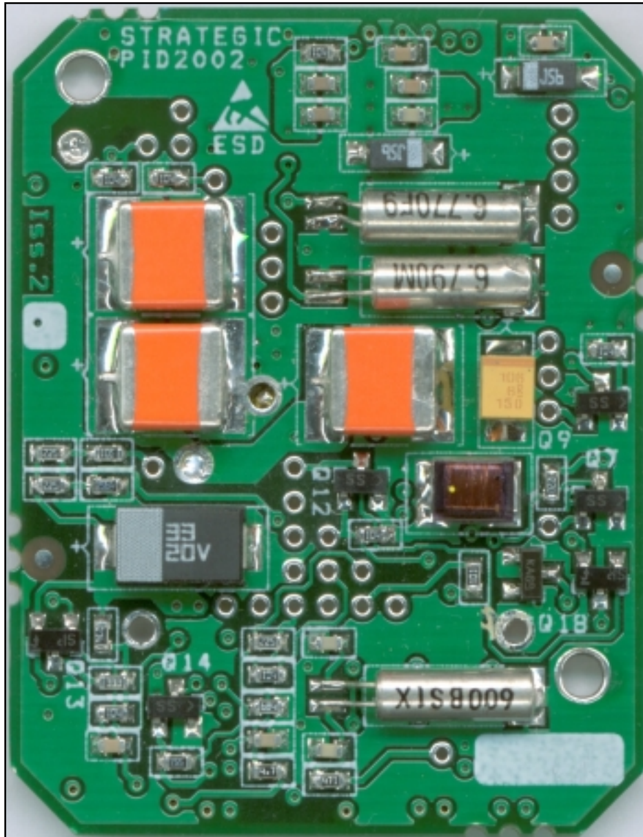
Figure 3: Internal PCB Rear view
