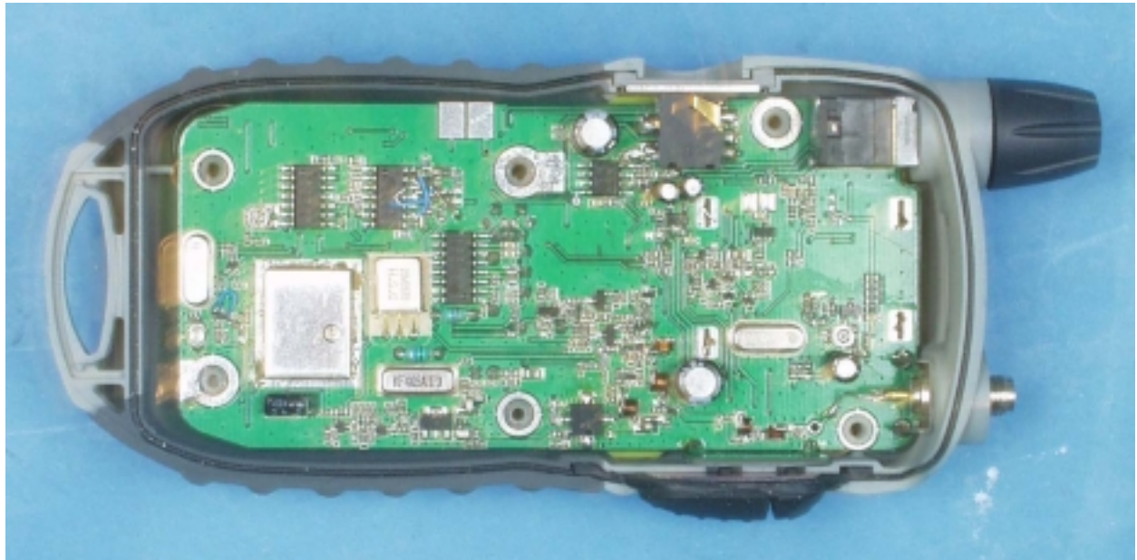
RF Board
