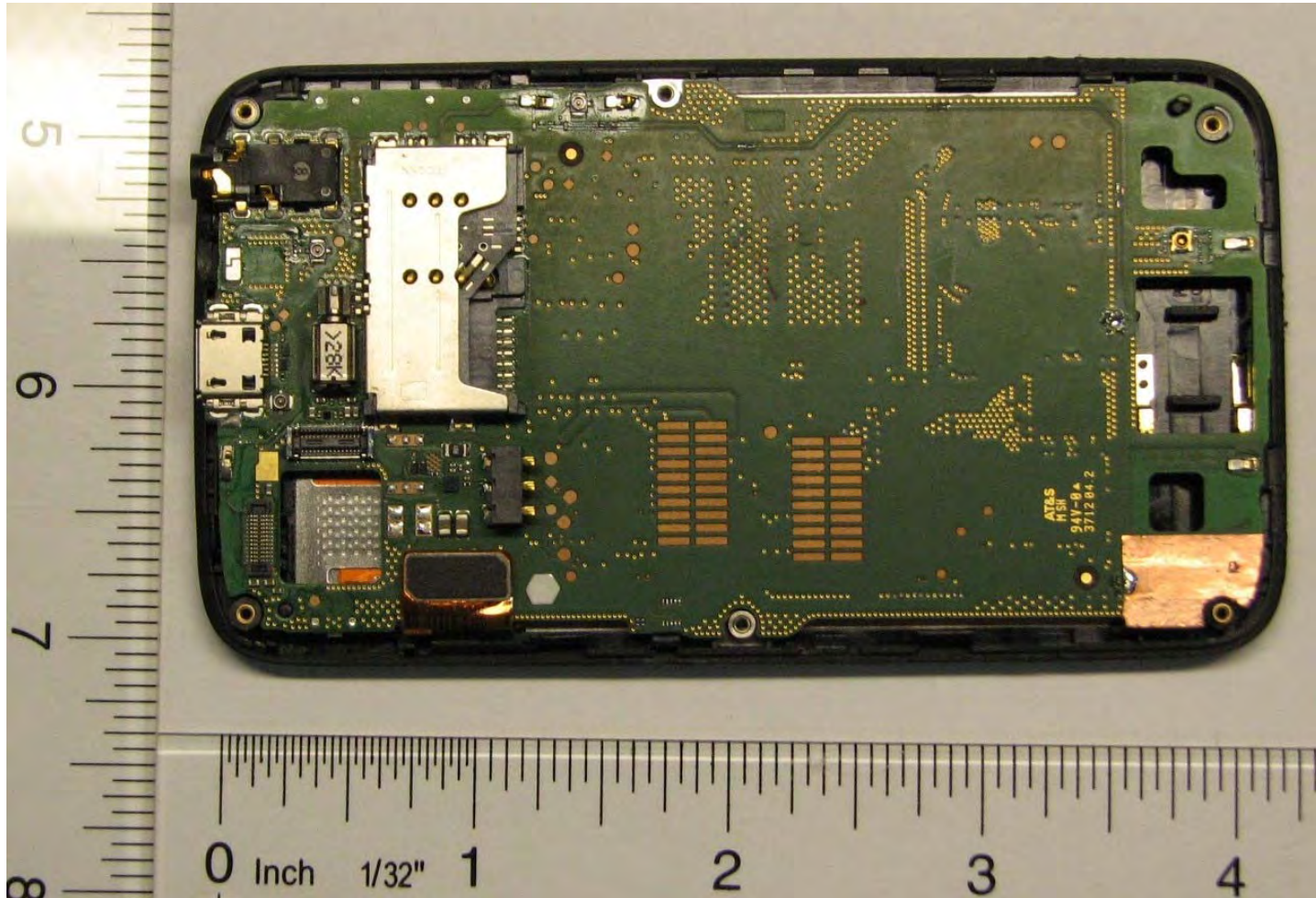
Figure 10: Battery removed
