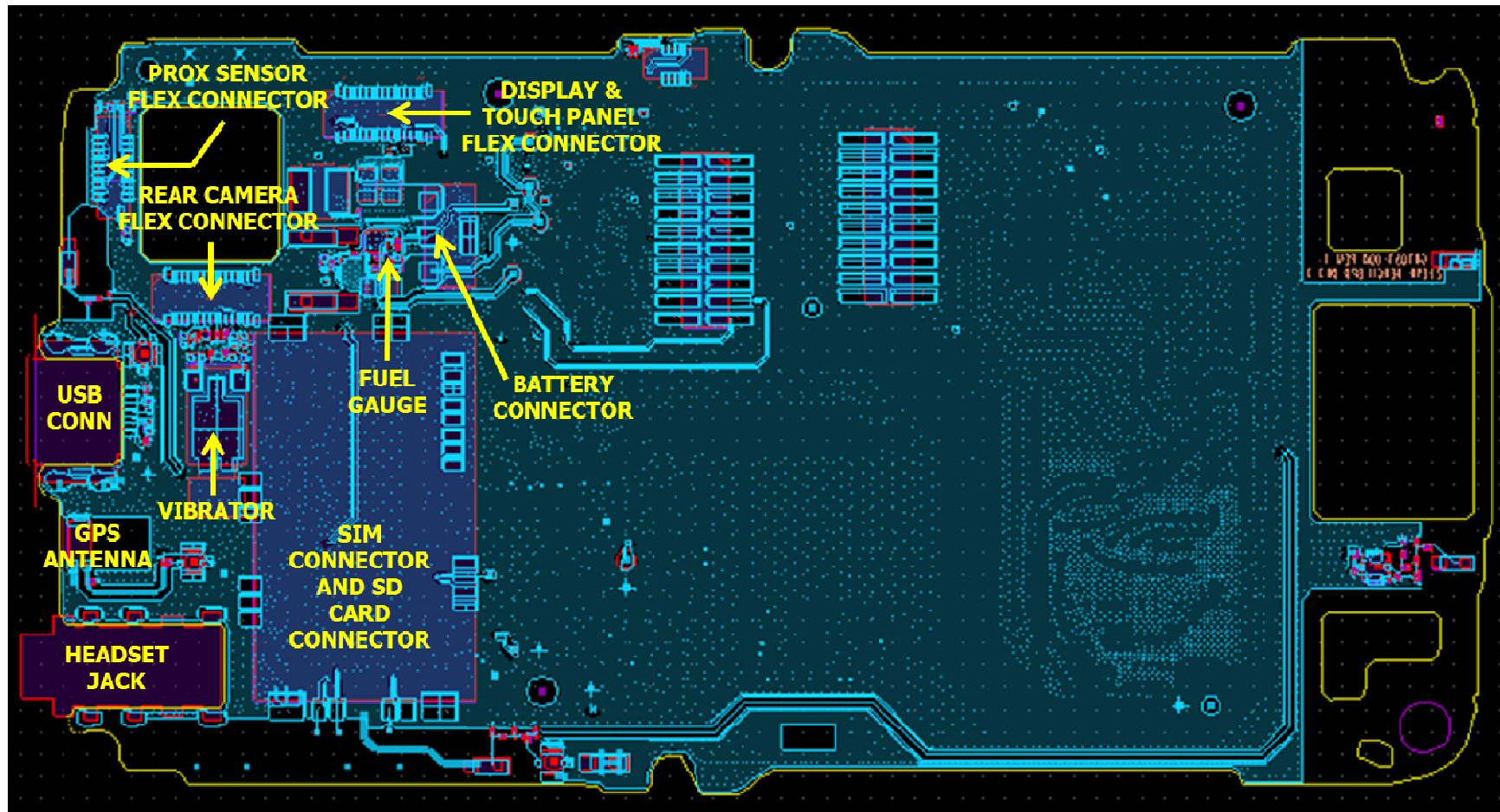
Figure 11: Component locations front side
