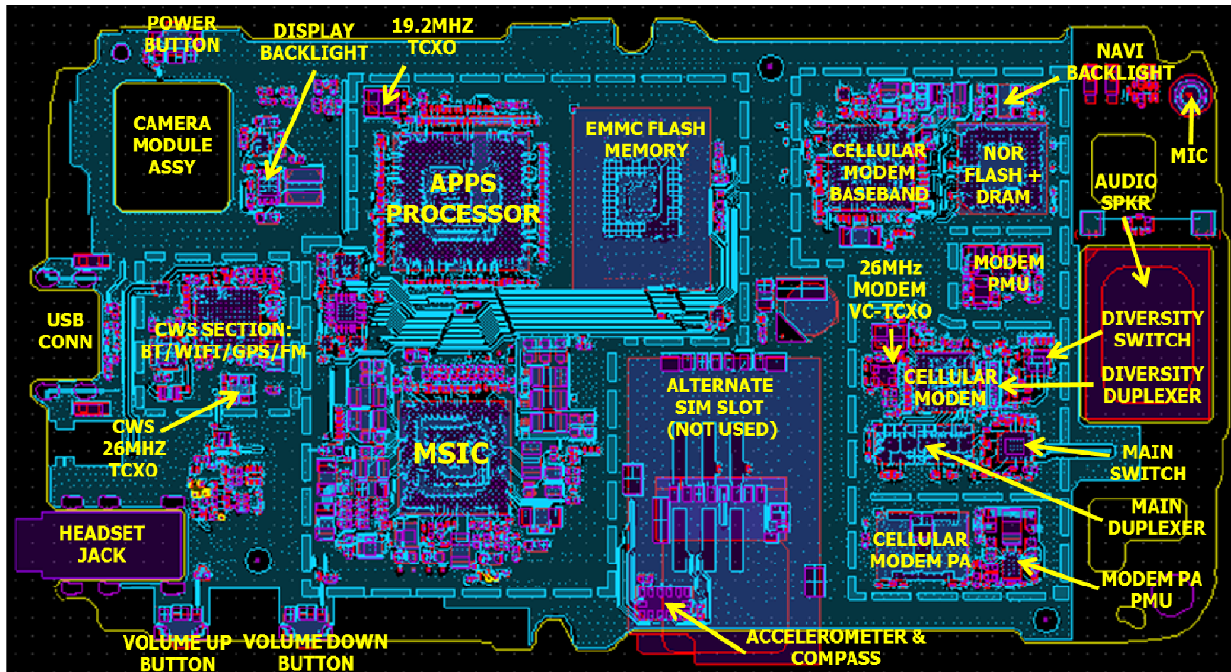
Figure 8: Component locations rear side
