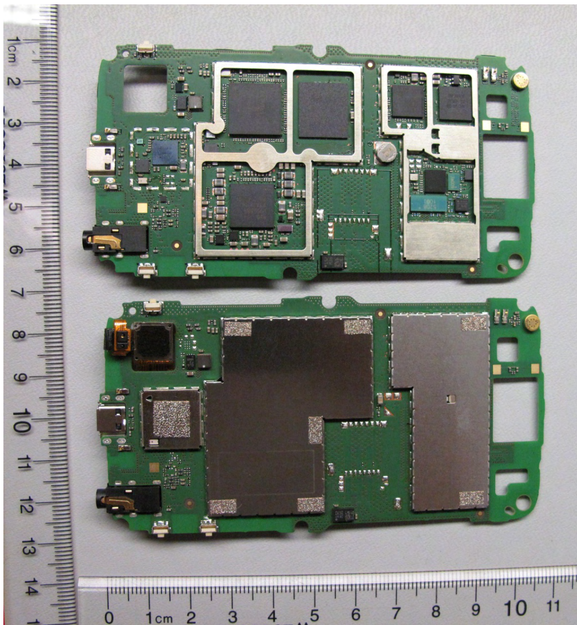
Figure 7: Main circuit board rear view
