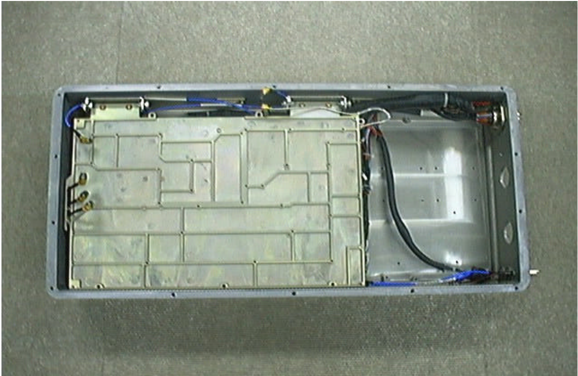
G27: INSIDE HOUSING WITH PLATE CLOSED
