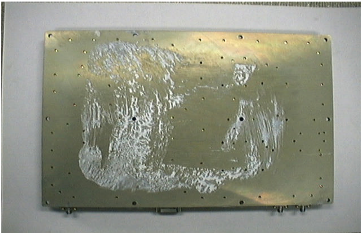
G22: POWER AMPLIFIER MODULE HOUSING (BACK VIEW)
