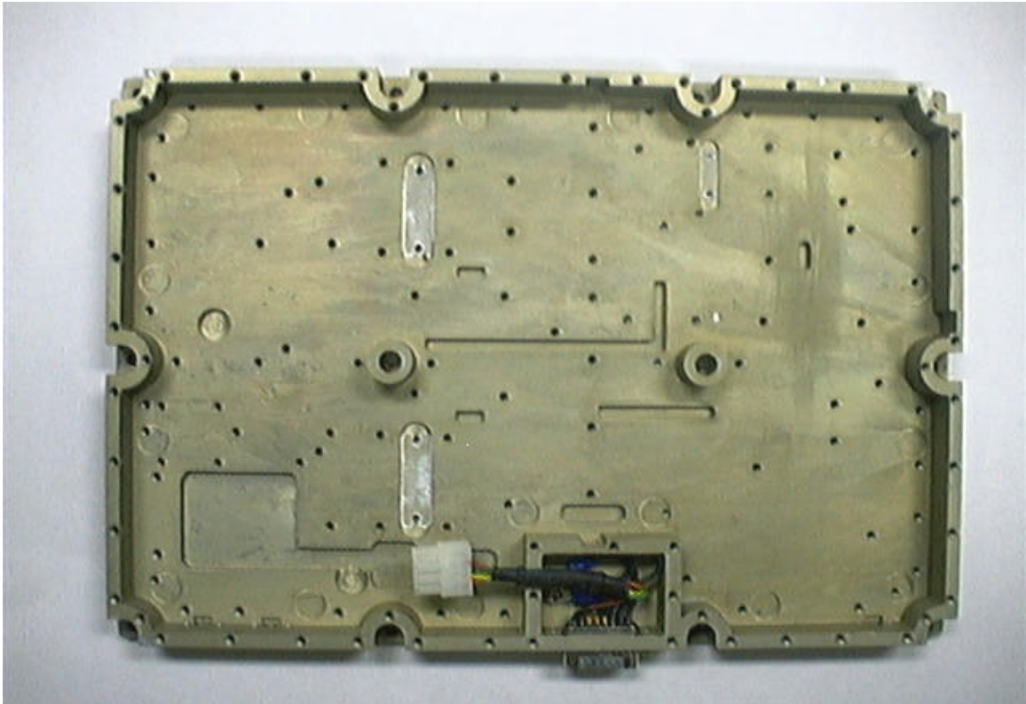
G21: POWER AMPLIFIER MODULE HOUSING (TOP/FRONT VIEW)
