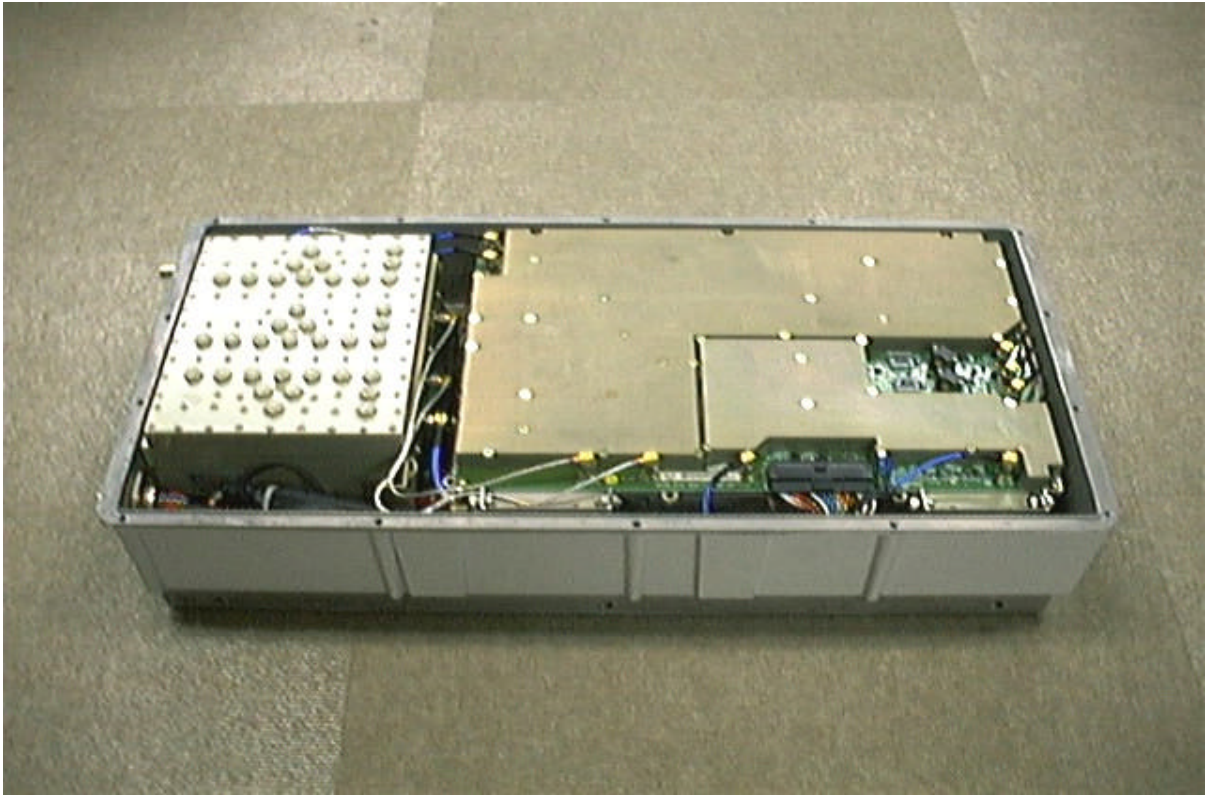
G5: UNIT ASSEMBLED (SIDE VIEW)
