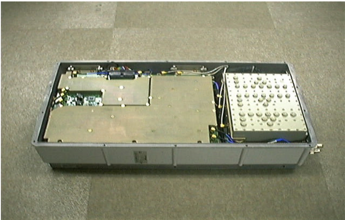
G6: UNIT ASSEMBLED (SIDE VIEW)
