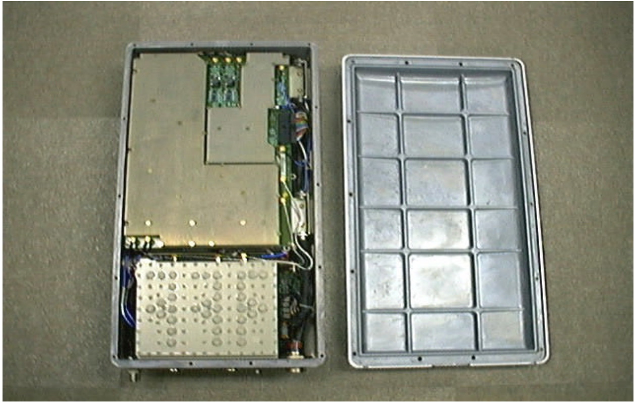
G1: UNIT ASSEMBLED (INSIDE VIEW)
