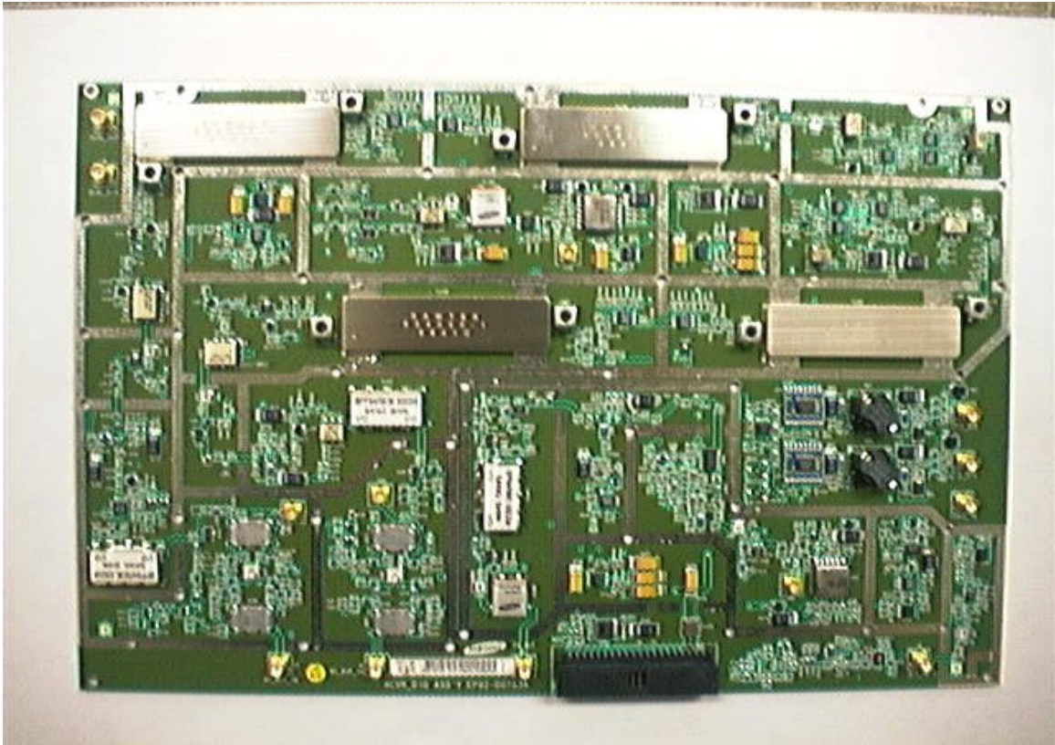
G17: TRANSCEIVER BOARD (TOP VIEW)
