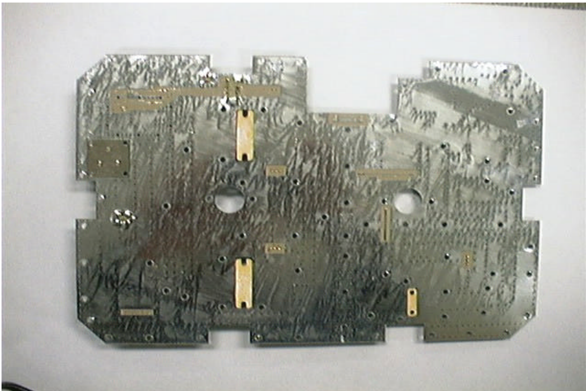
G20: POWER AMPLIFIER AND DRIVER STAGE PCB (BACK VIEW)
