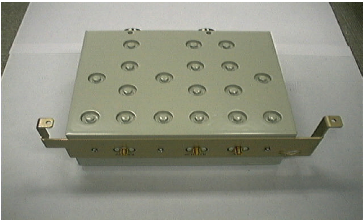
G10: DUPLEX WITH CONNECTORS (BOTTOM VIEW)
