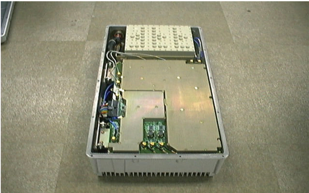
G4: UNIT ASSEMBLED (TOP VIEW)
