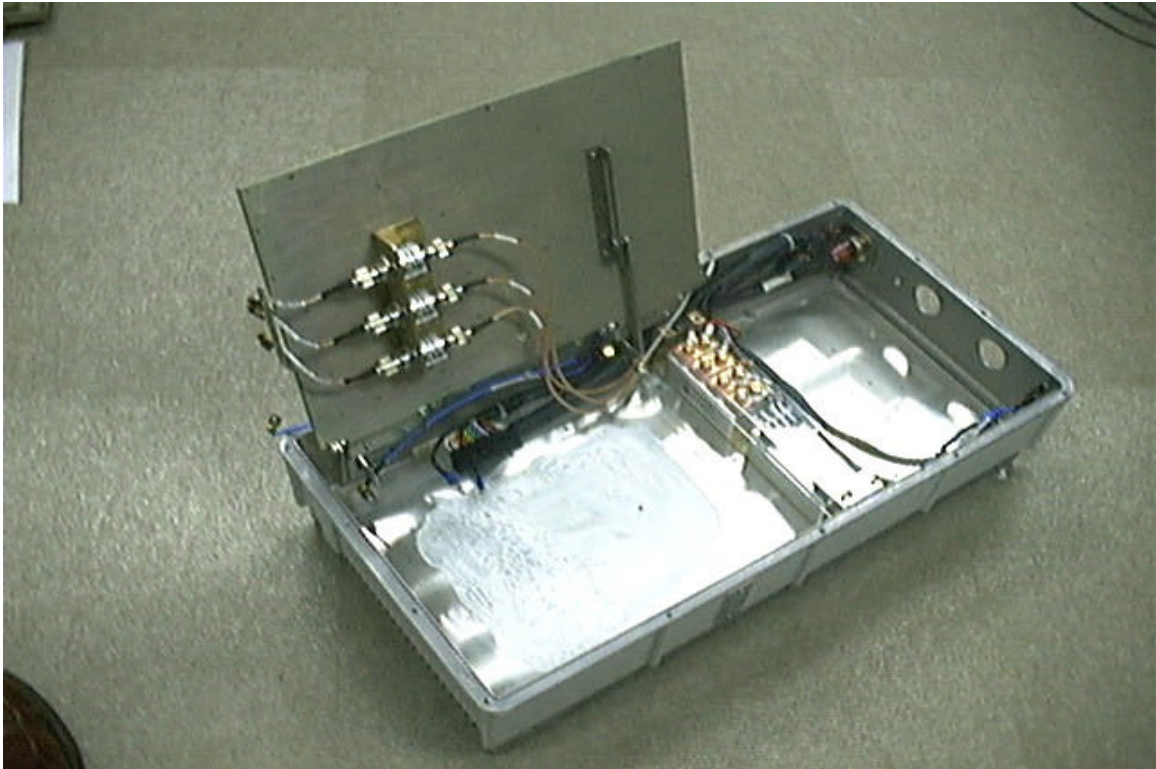
G25: INSIDE HOUSING WITH CARDS REMOVED (SIDE VIEW)
