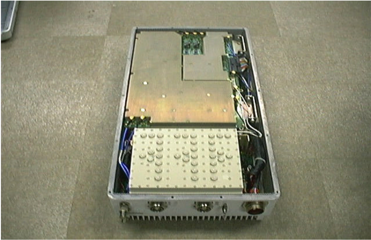
G3: UNIT ASSEMBLED (BOTTOM VIEW)
