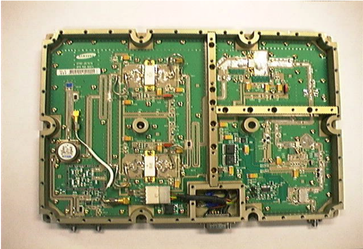
G19: POWER AMPLIFIER MODULE (TOP VIEW)
