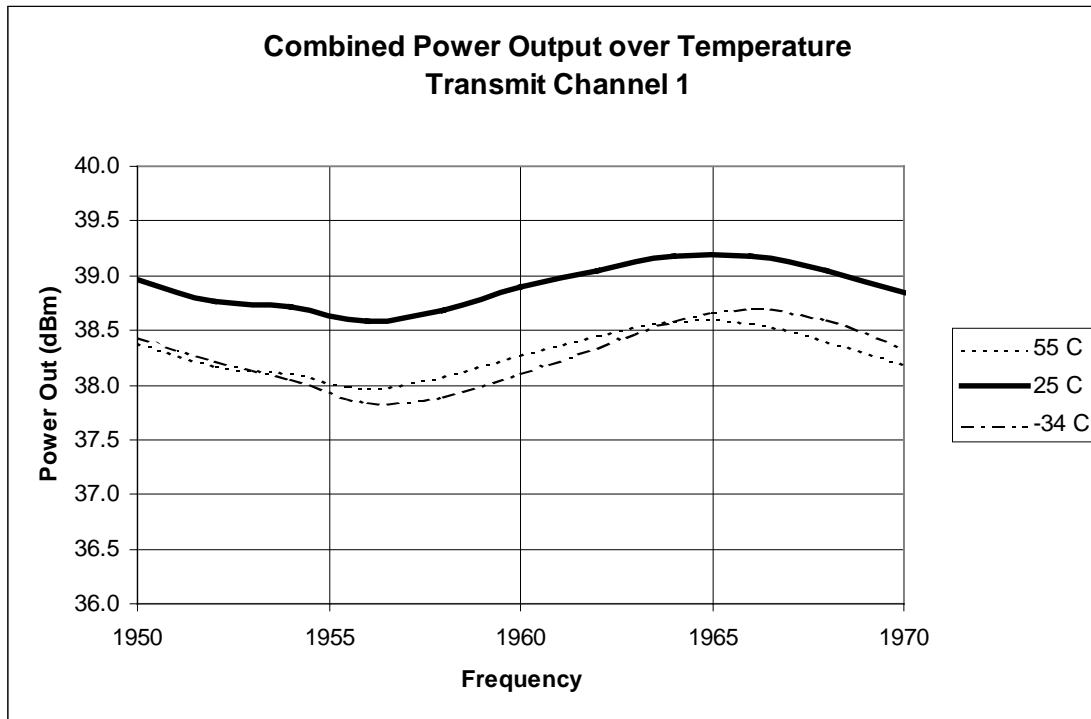
Figure 4-2 RF Power Output over Temperature – Channel 1
