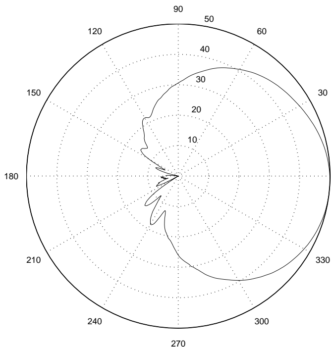
Figure 4-3- Measured Horizontal Radiation Pattern of the Active Antenna Aperture
