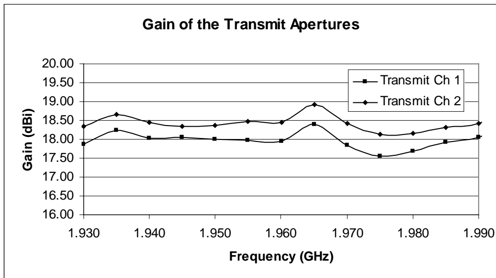
Figure 4-4 Measured Gain of the Transmit Antenna
