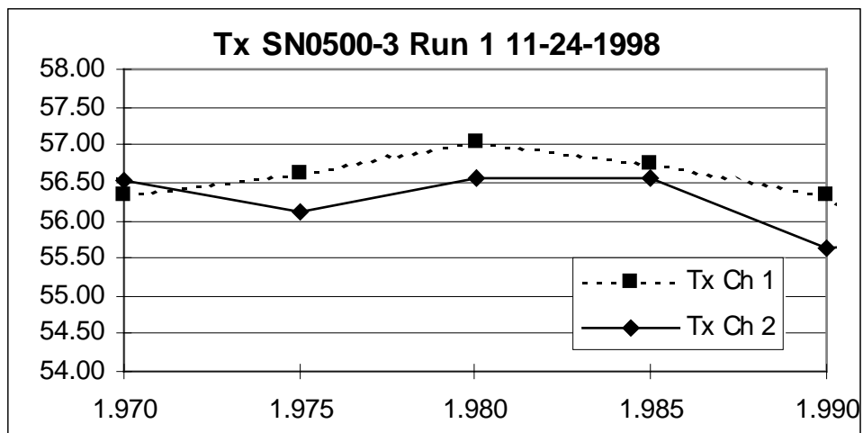
Figure 4-7 – EIRP of the Band 3 Active Antenna (C and F Blocks)
