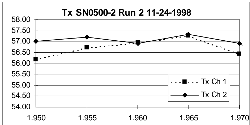
Figure 4-6 – EIRP of the Band 2 Active Antenna (B and E Blocks)
