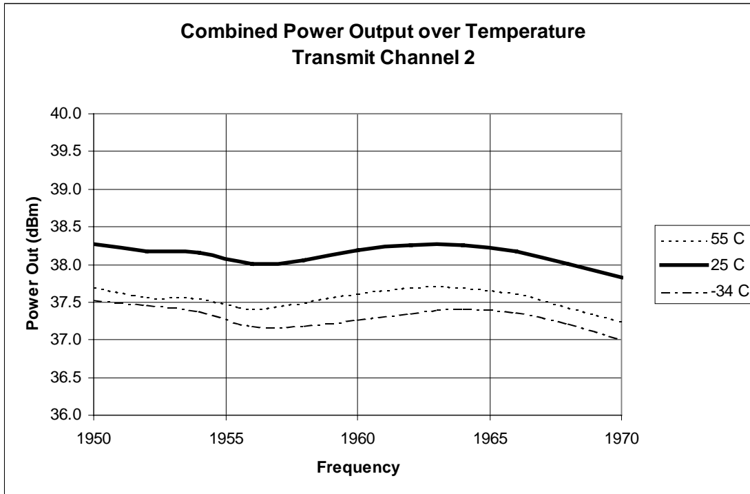
Figure 4-3 RF Power Output over Temperature – Channel 2
