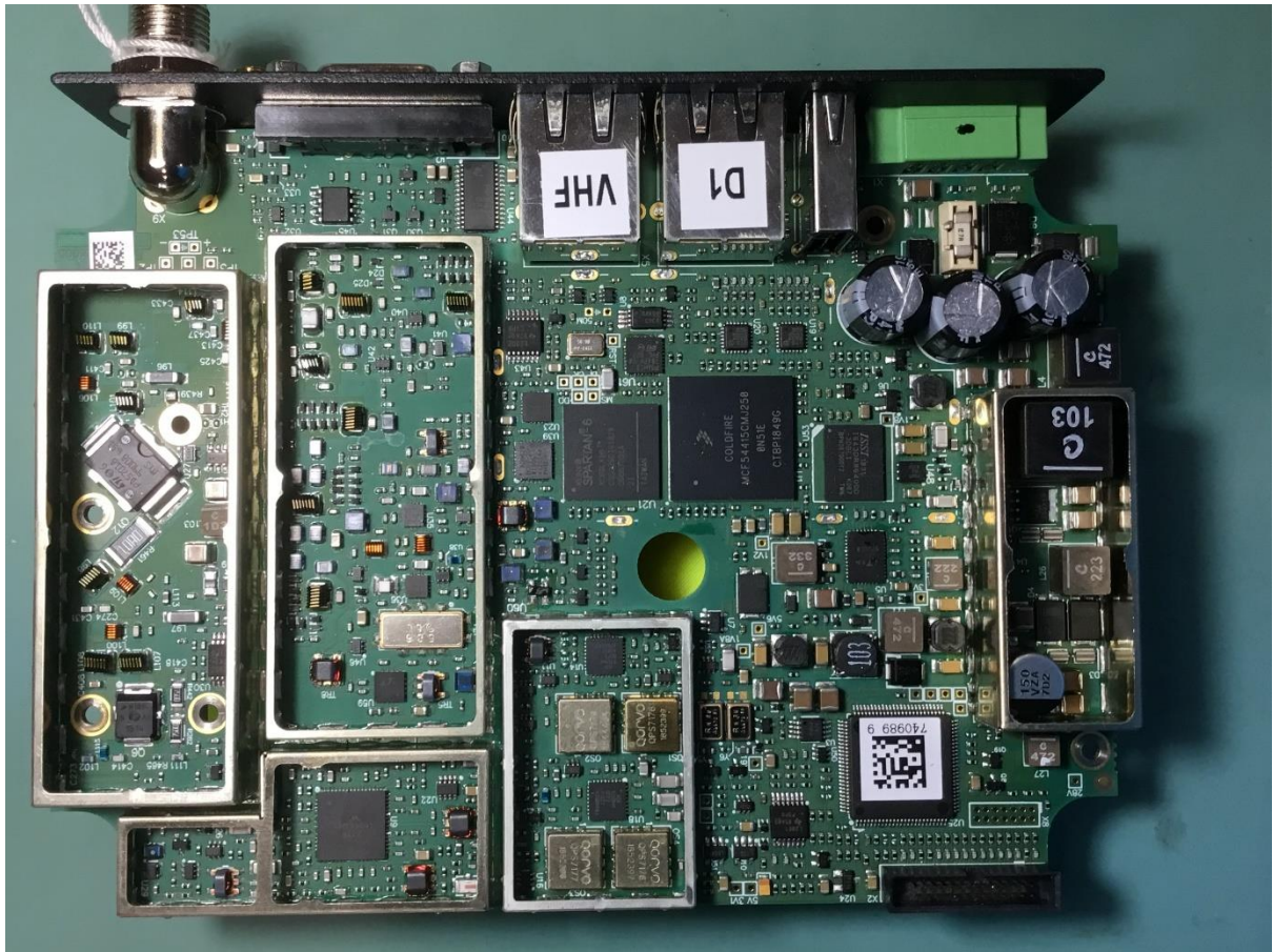
Figure 3 Top Side - Shields off
