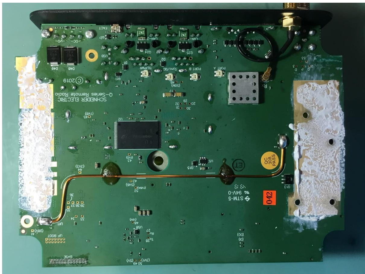
Figure 2 Bottom Side - Shields on
